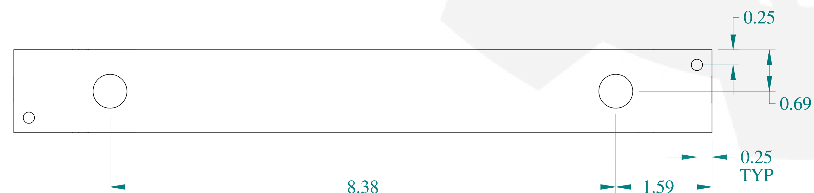
BOTTOM VIEW
