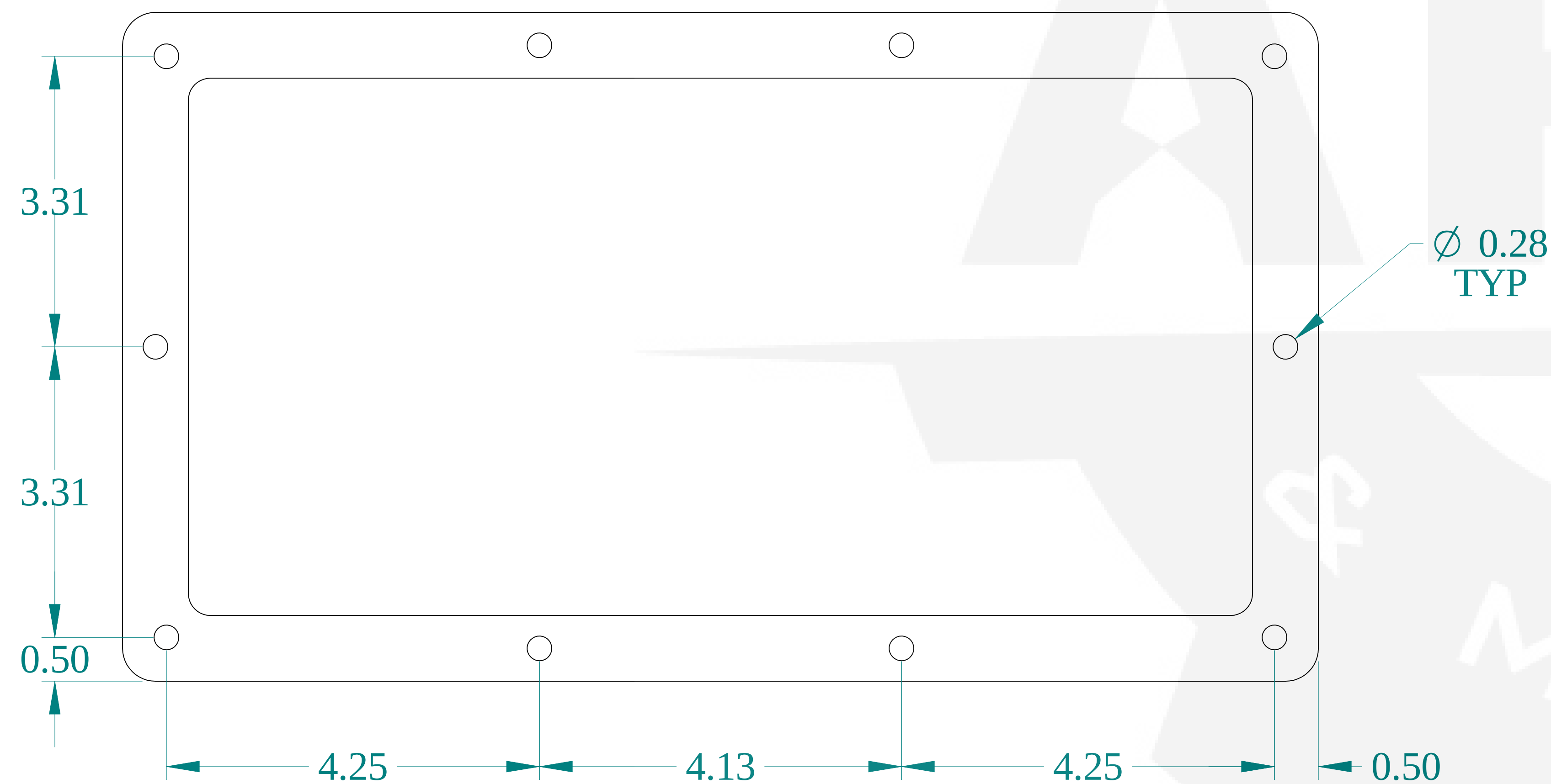
FRONT VIEW
