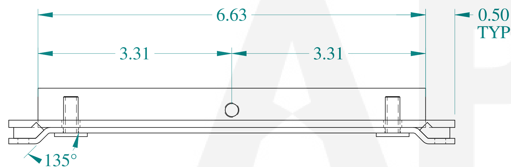
FRONT VIEW
