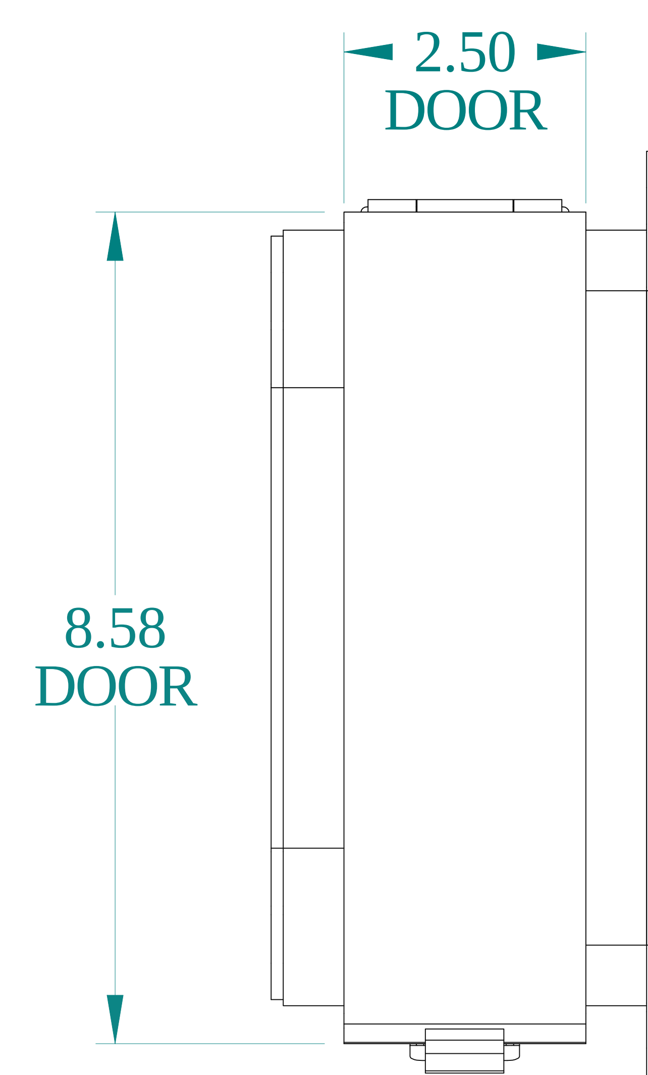
TOP VIEW
