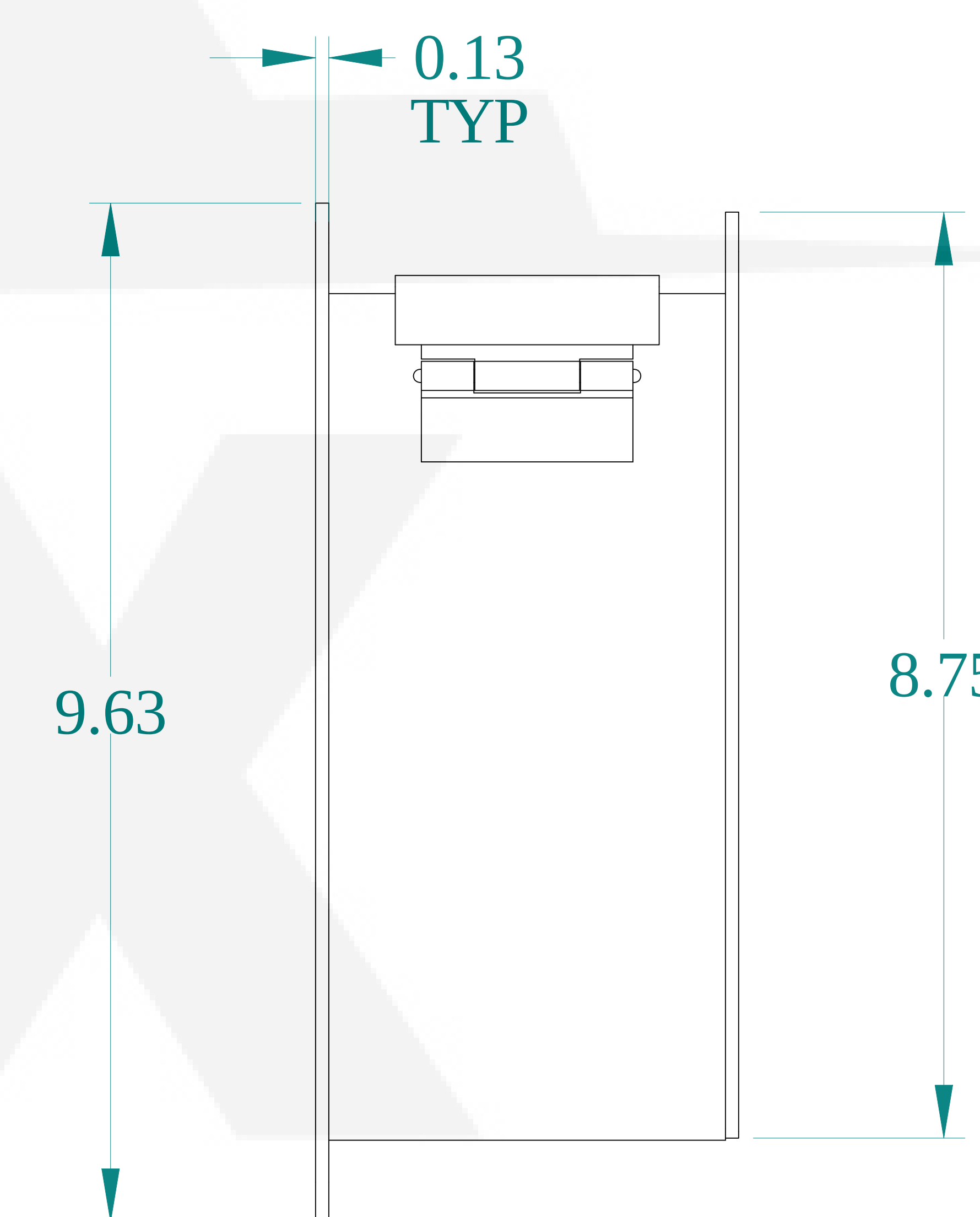
BACK VIEW
