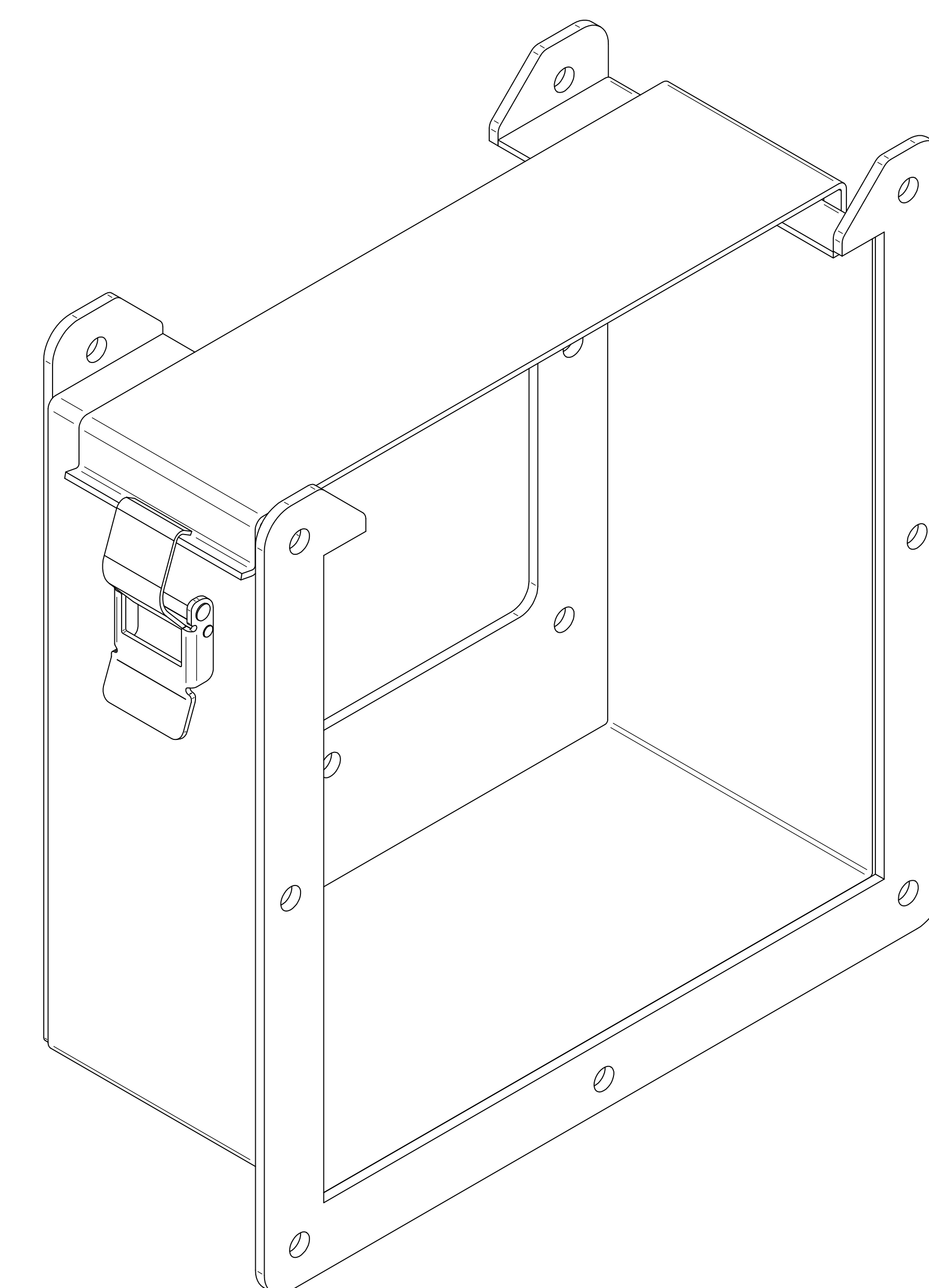
ISOMETRIC VIEWS
