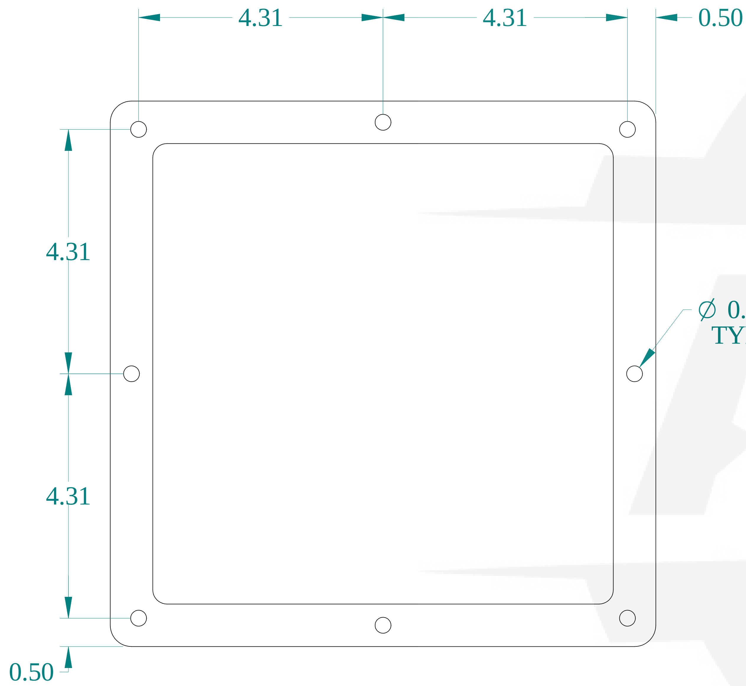
FRONT VIEW
