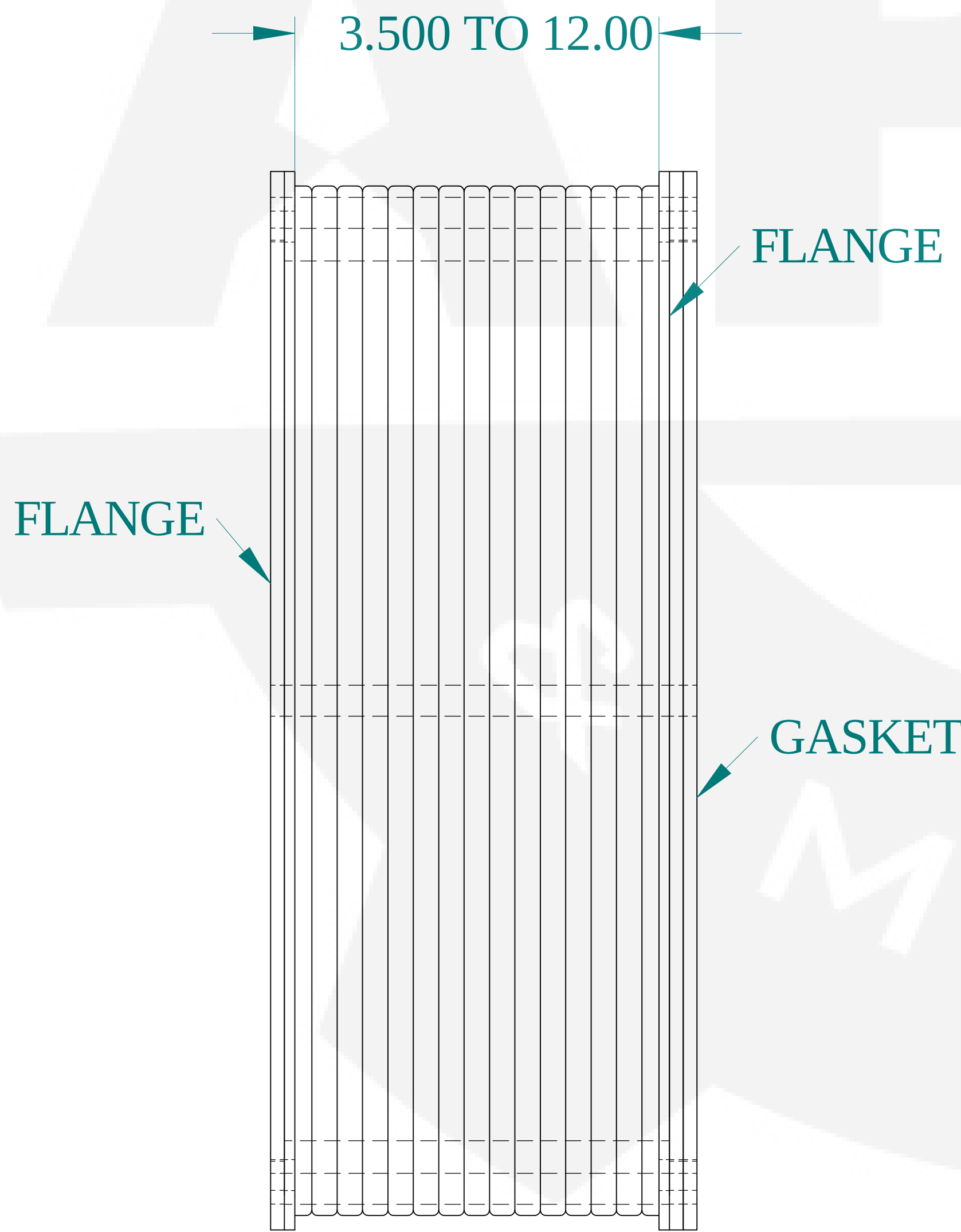
FRONT VIEW
