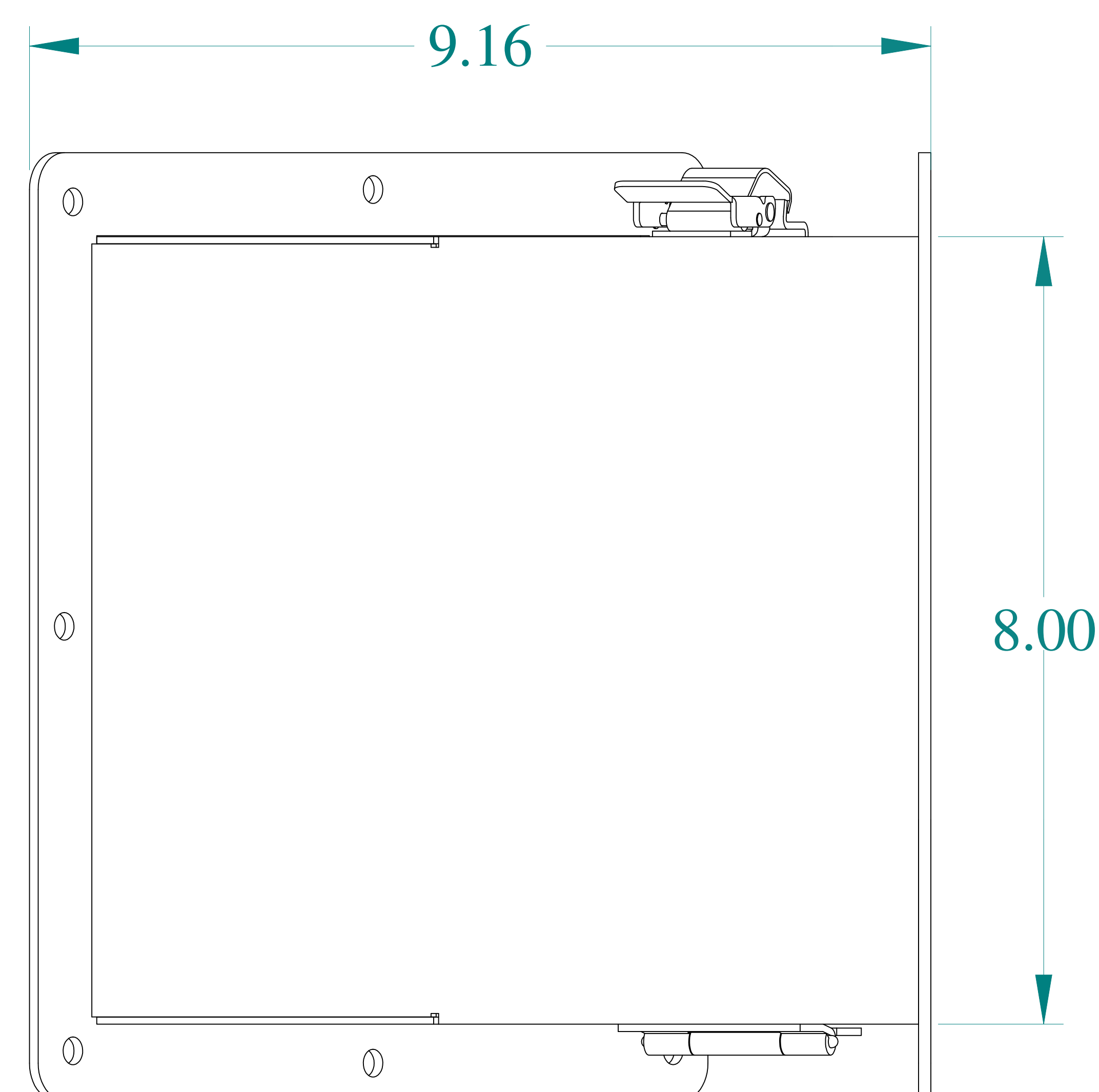
BOTTOM VIEW
