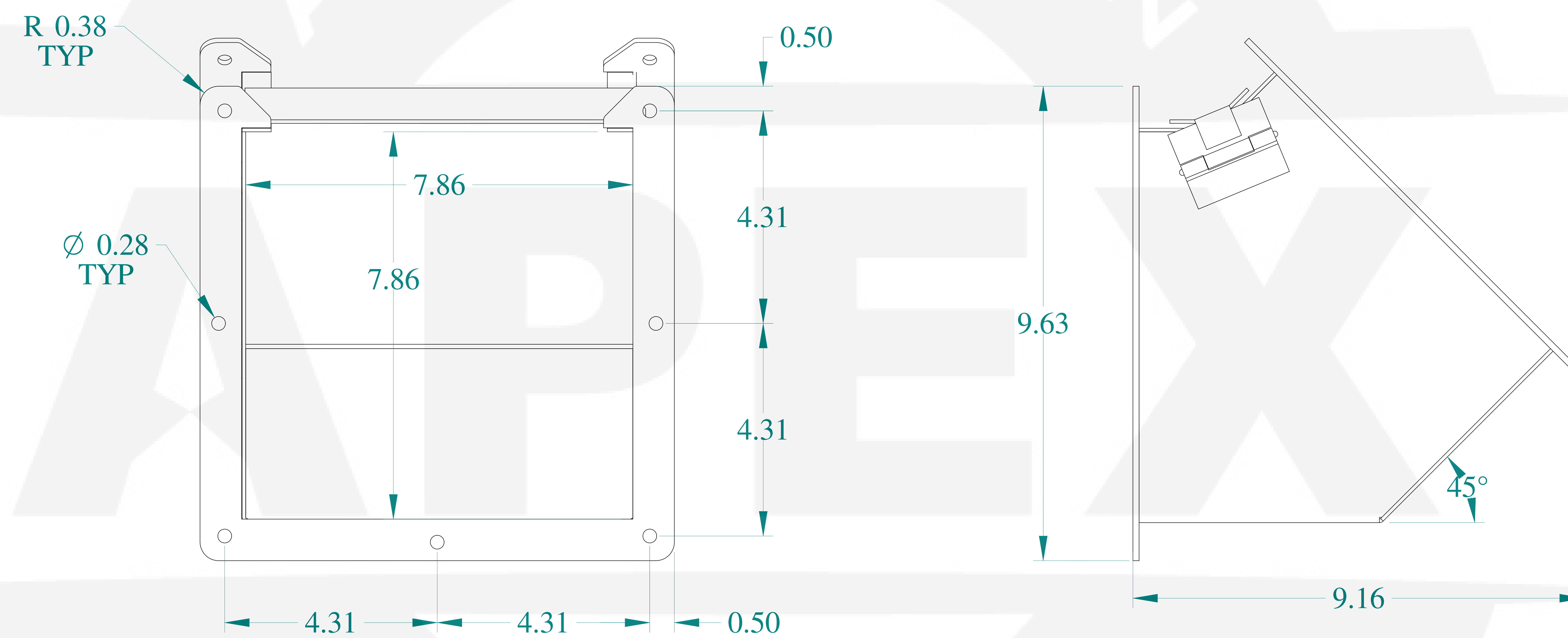
BACK VIEW
