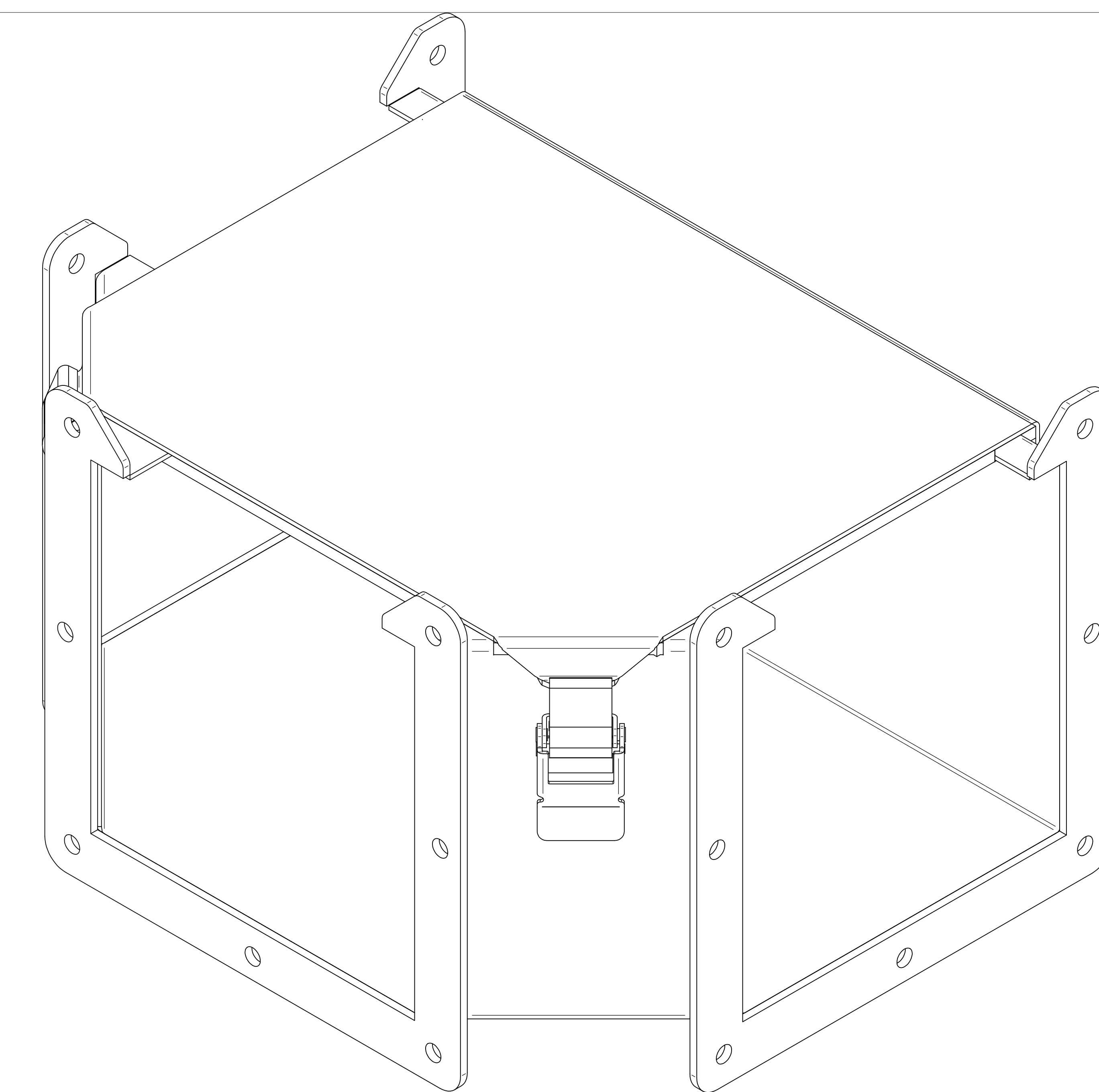
ISOMETRIC VIEWS
