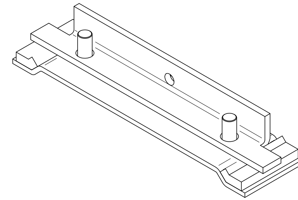
ISOMETRIC VIEWS
