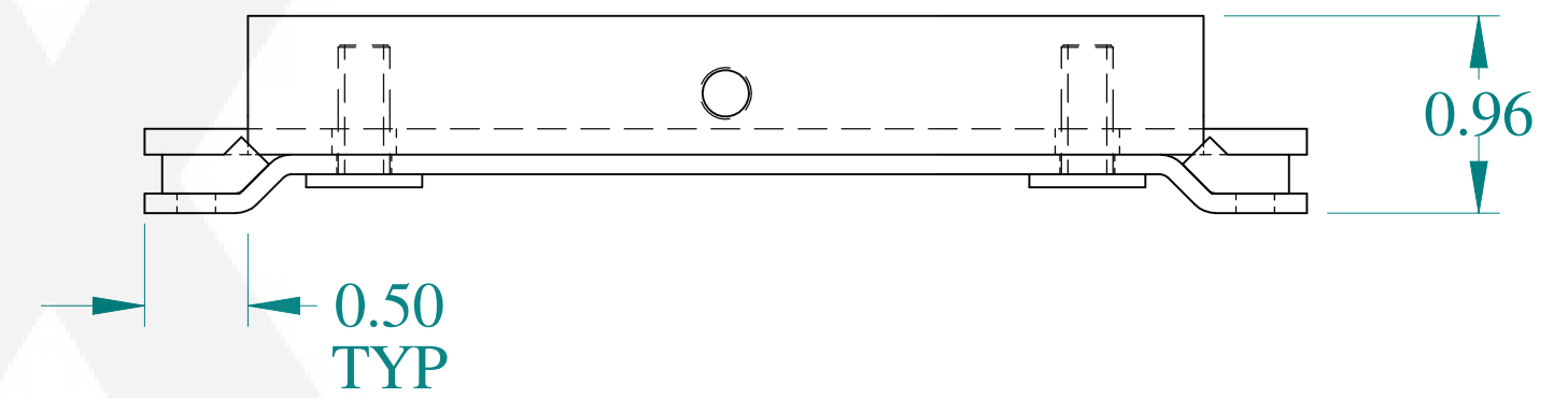
BACK VIEW
