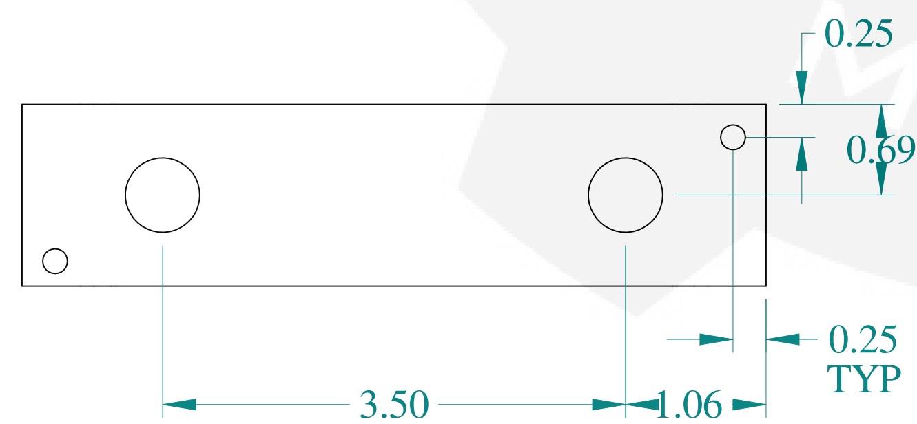
BOTTOM VIEW
