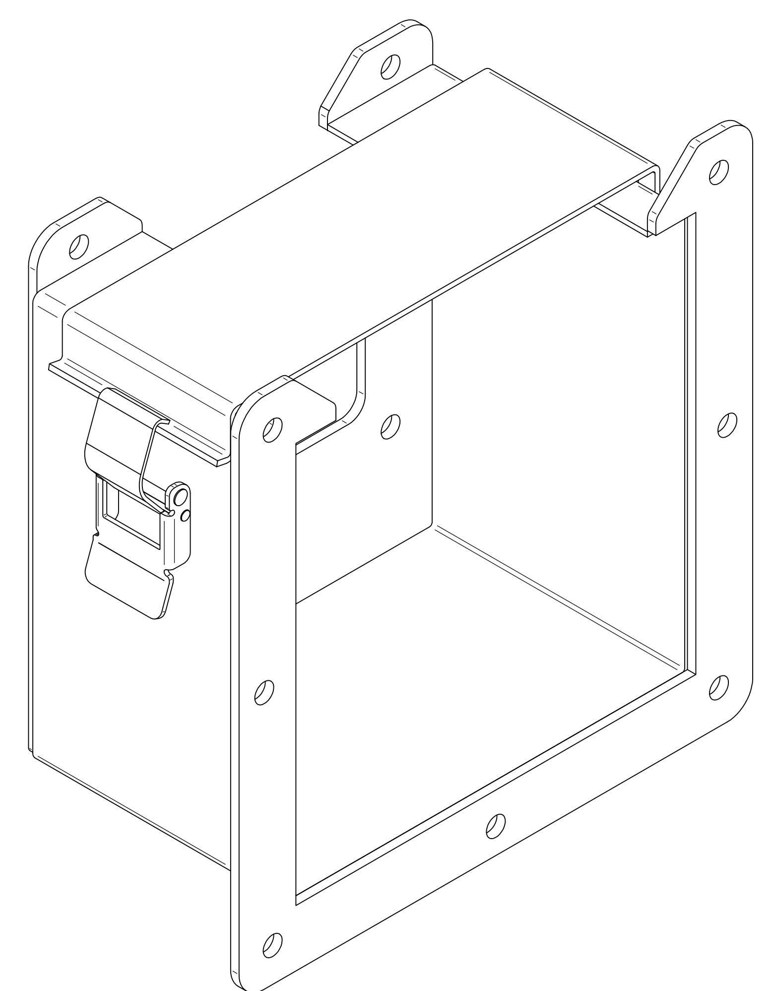
ISOMETRIC VIEWS
