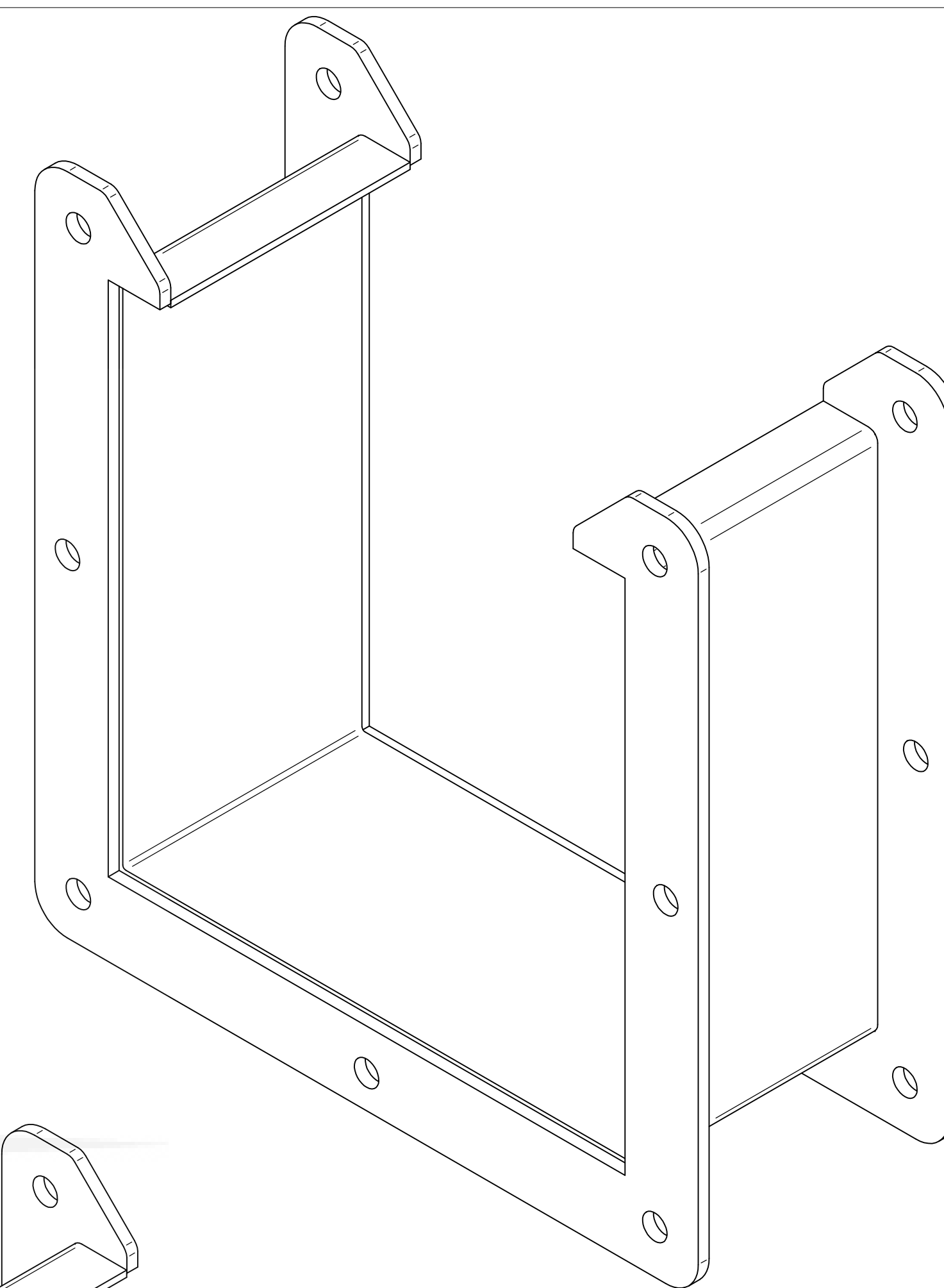
ISOMETRIC VIEWS
