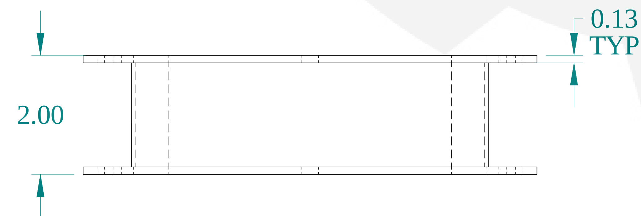
BOTTOM VIEW
