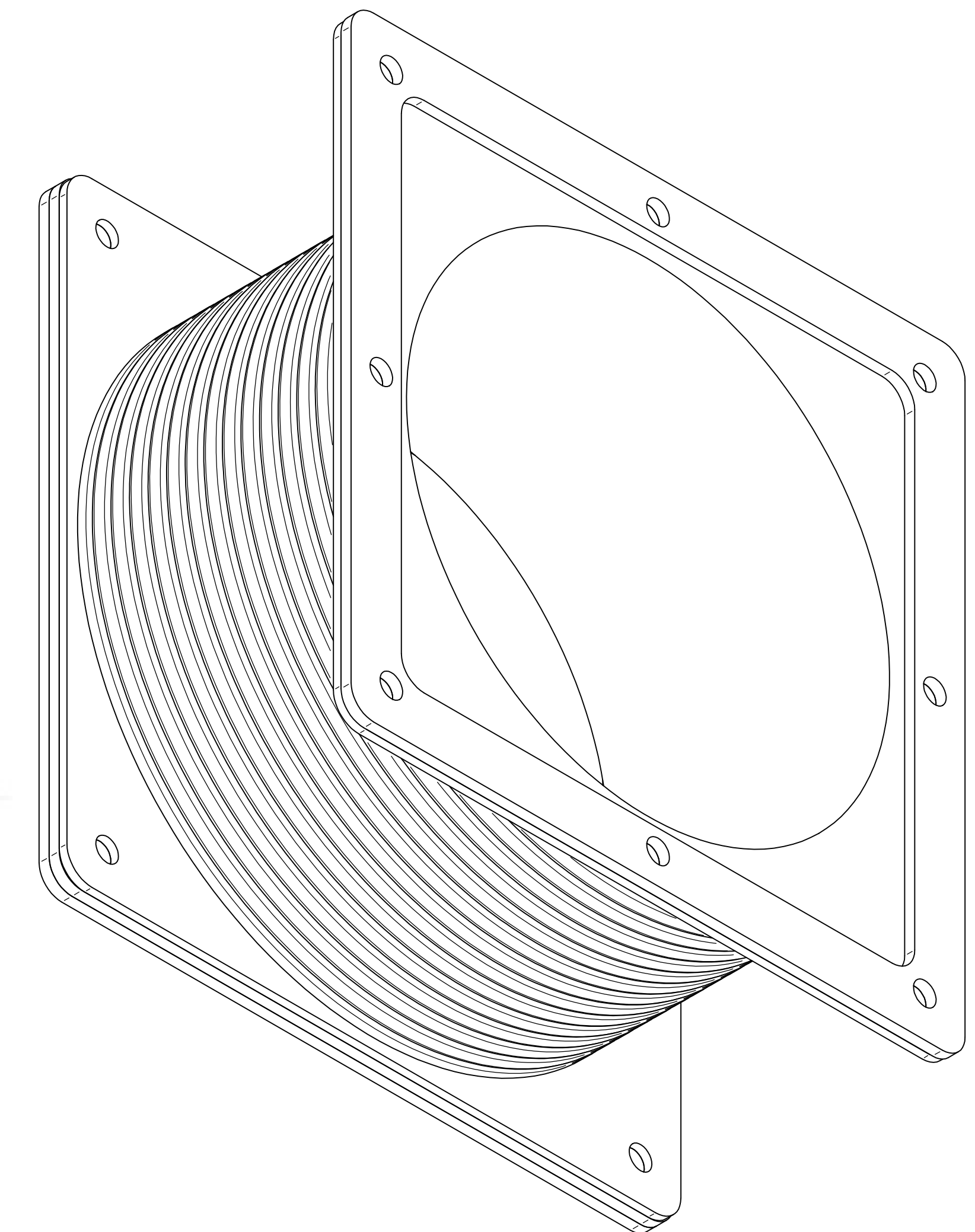
ISOMETRIC VIEWS
