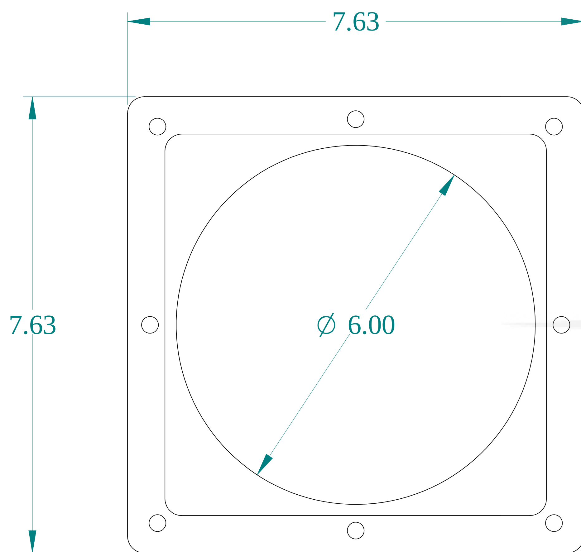
SIDE VIEW
