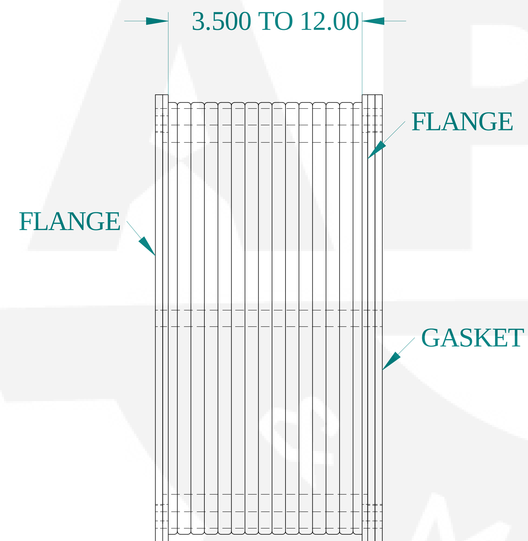
FRONT VIEW
