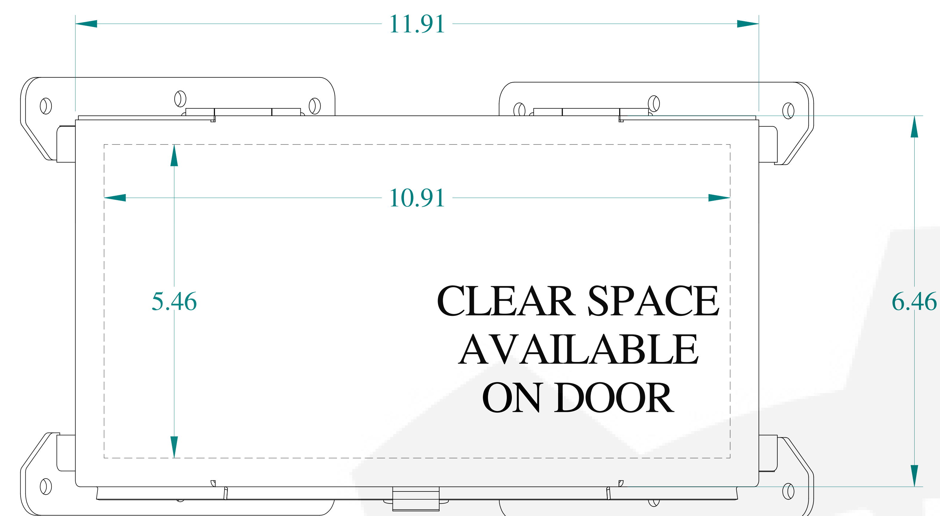
TOP VIEW
