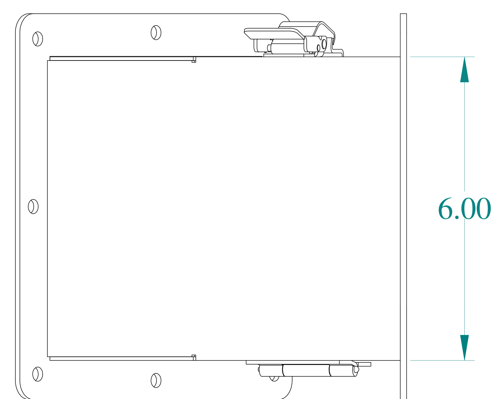
BOTTOM VIEW
