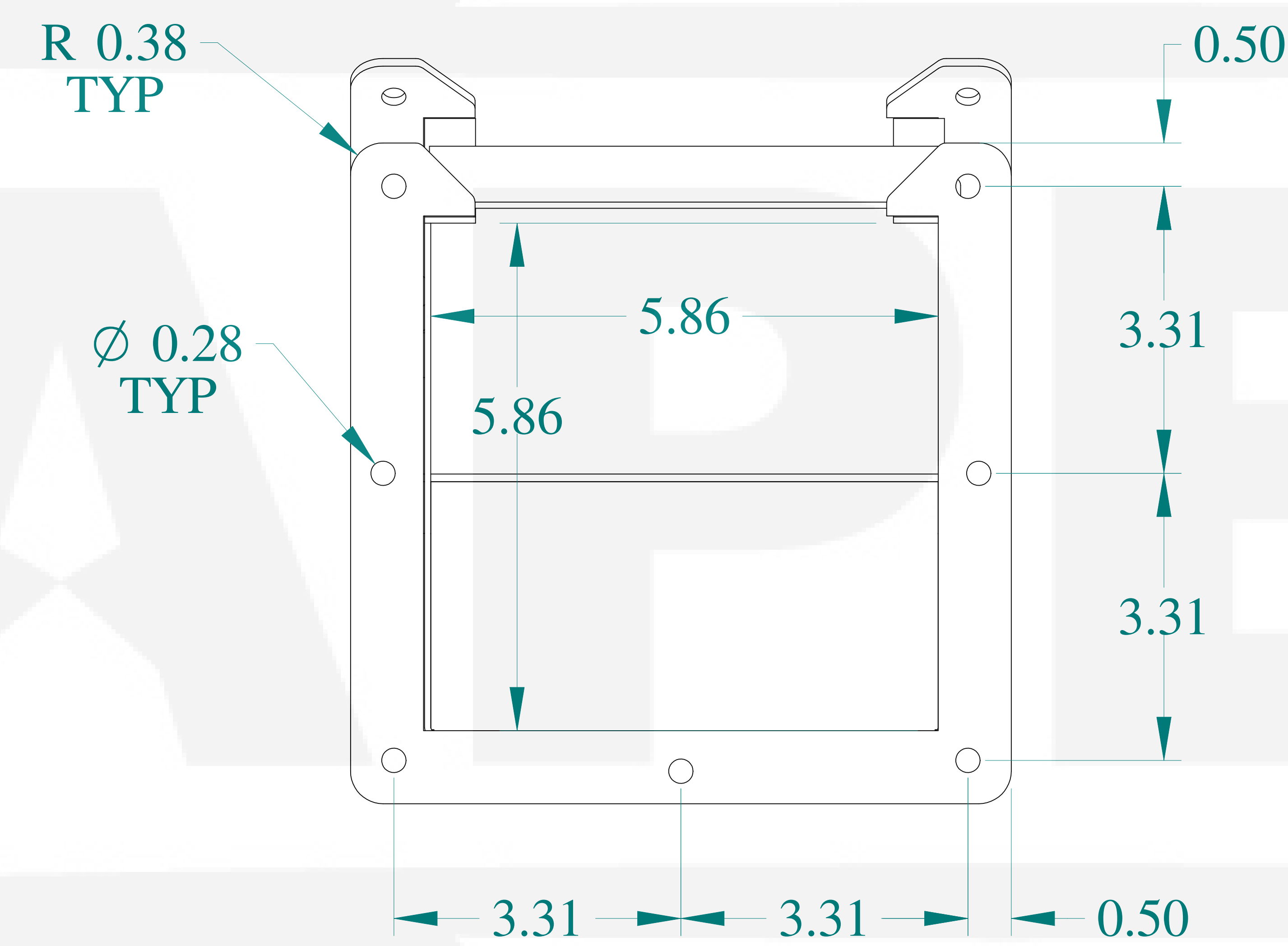
SIDE VIEW
