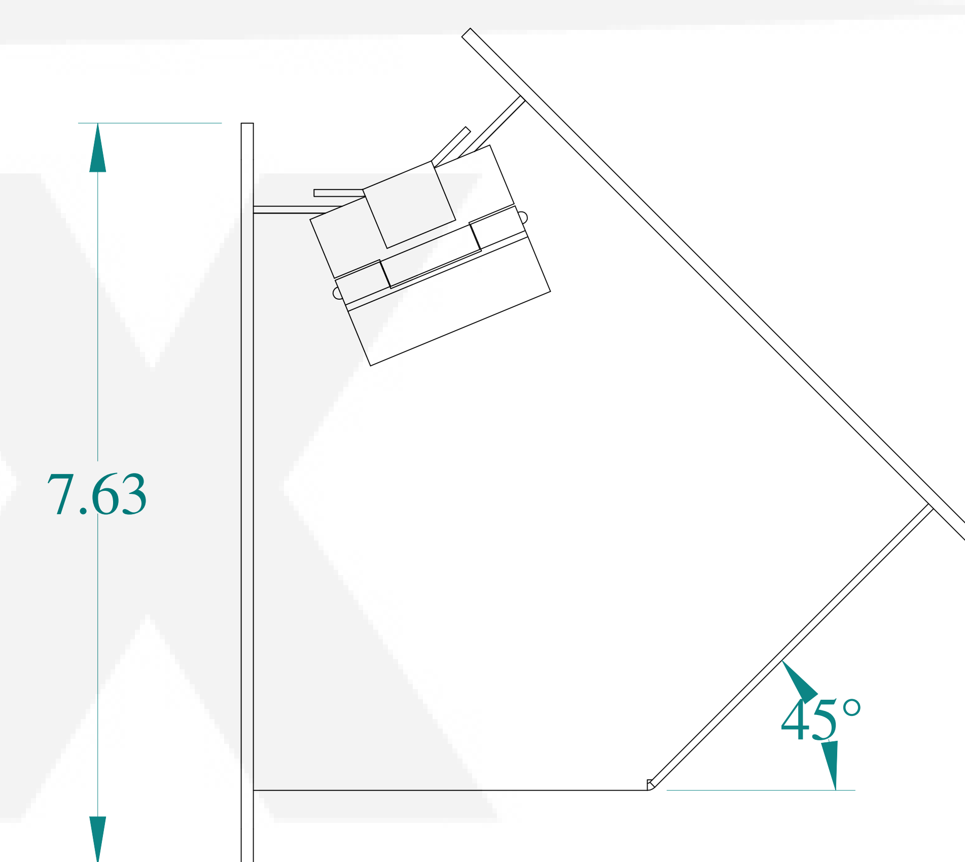
BACK VIEW
