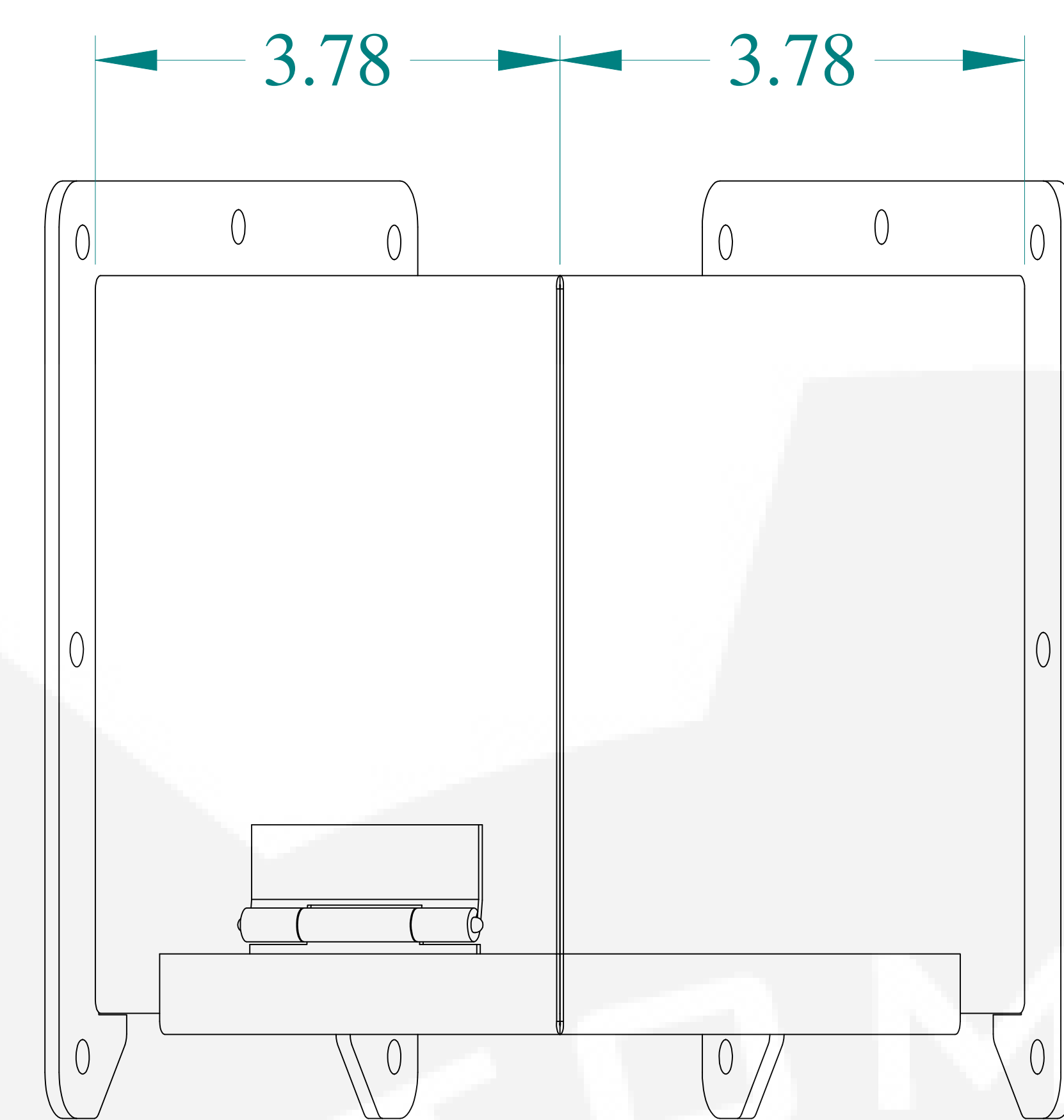
TOP VIEW
