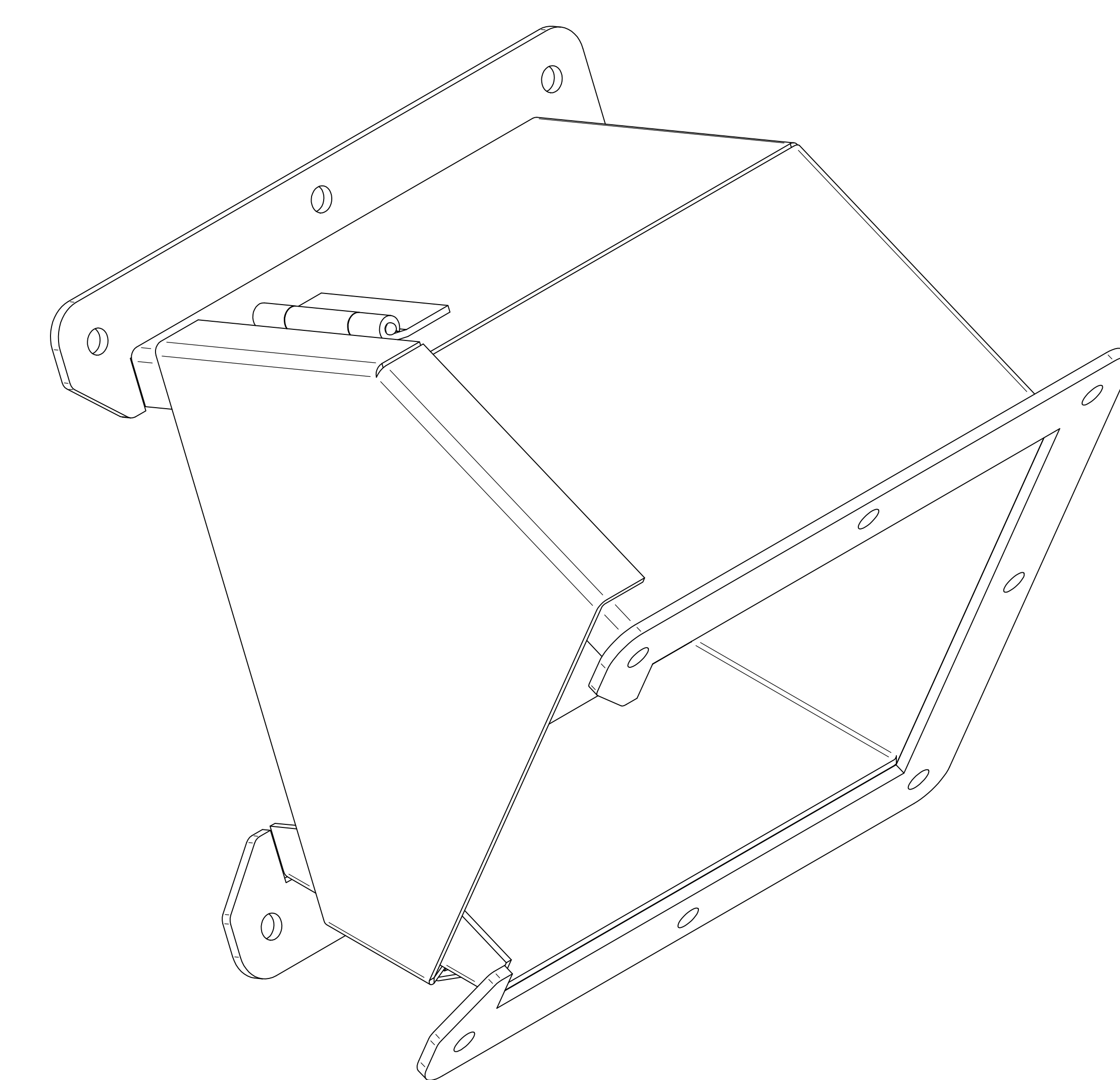
ISOMETRIC VIEWS
