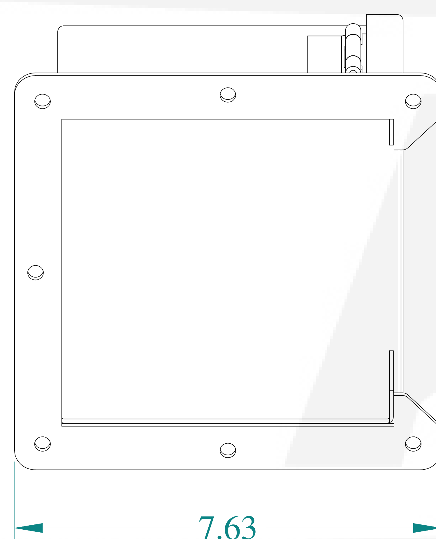
SIDE VIEW
