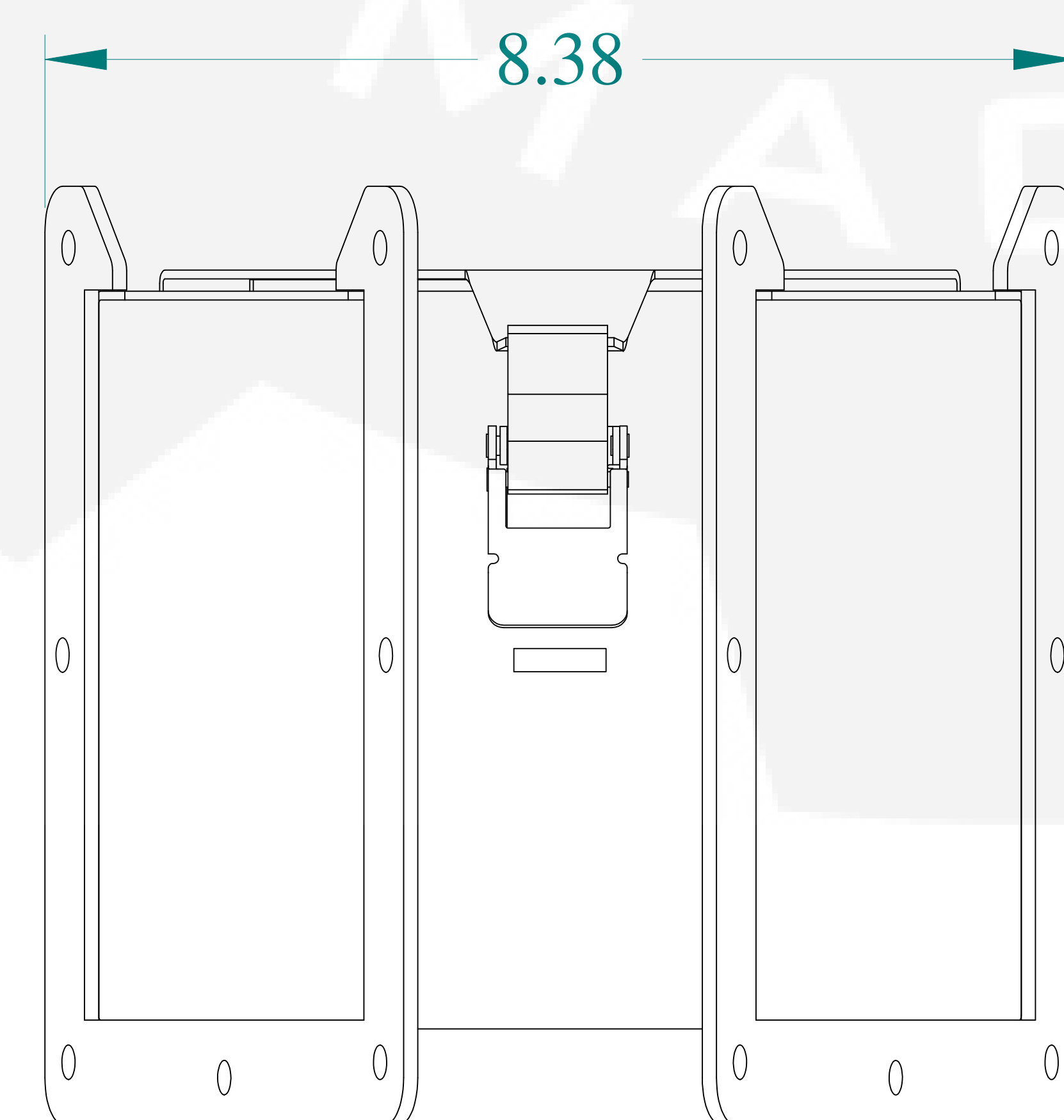
BOTTOM VIEW
