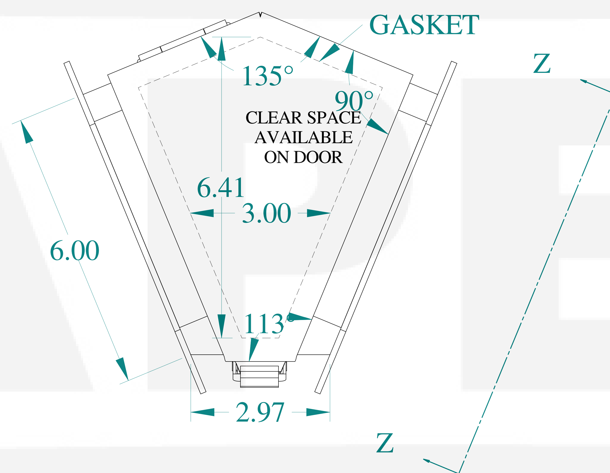
FRONT VIEW
