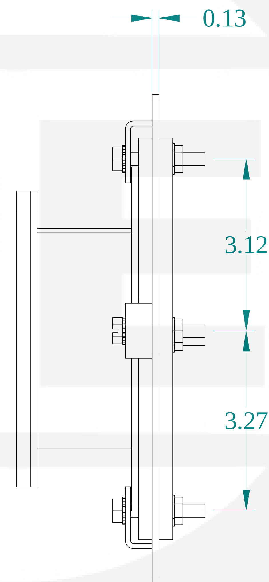
SIDE VIEW
