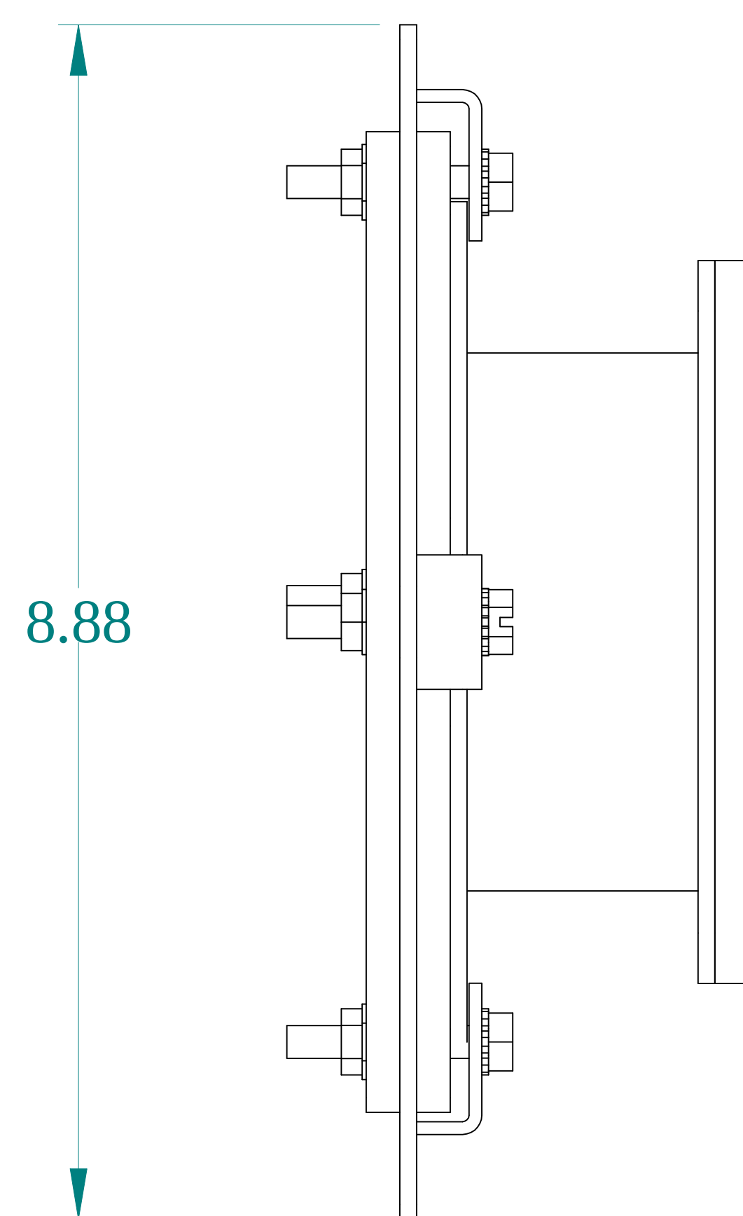
SIDE VIEW
