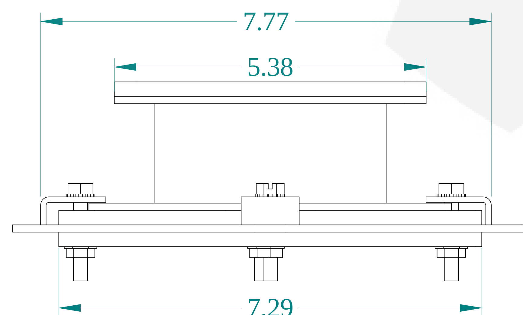
BOTTOM VIEW
