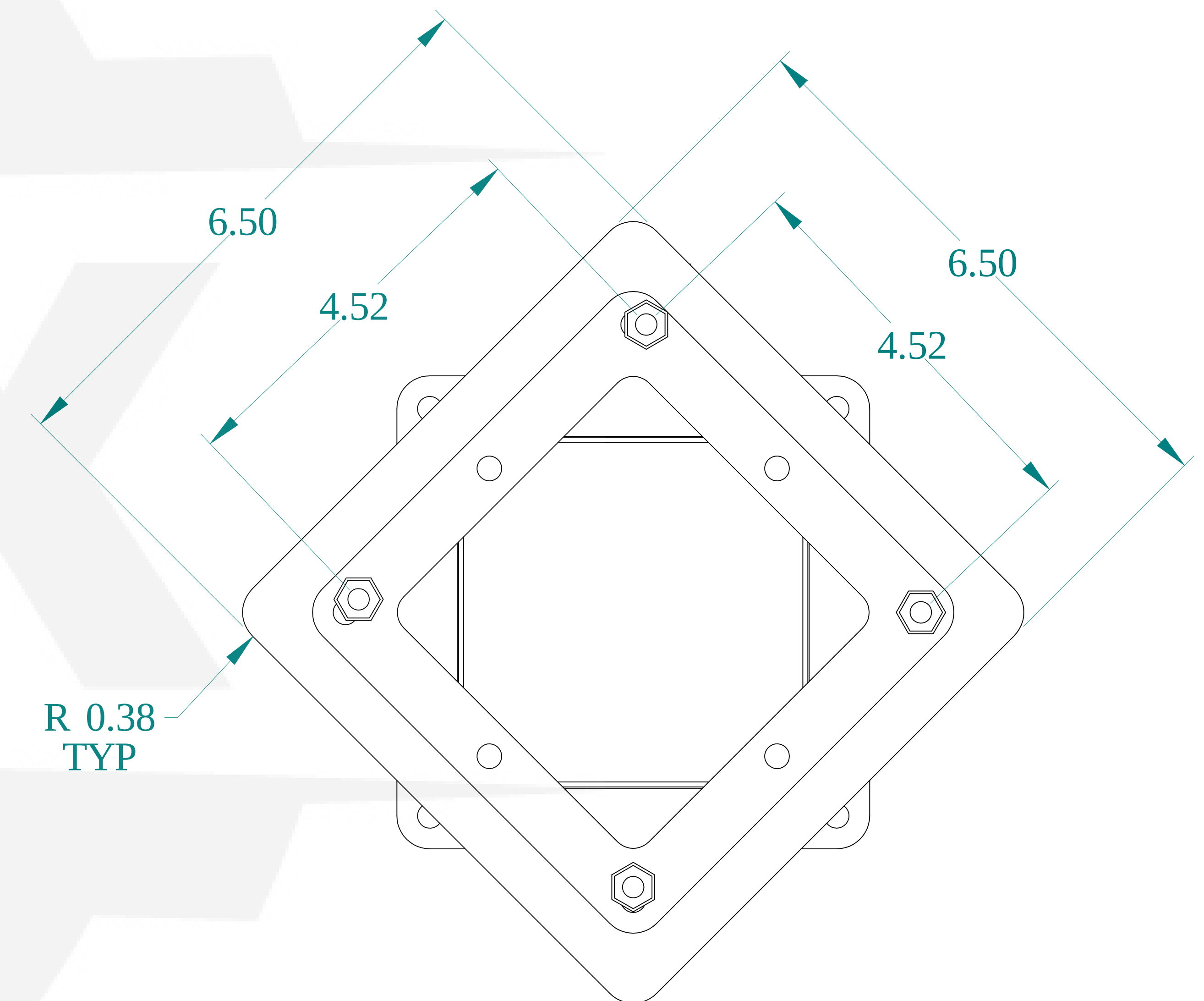
BACK VIEW
