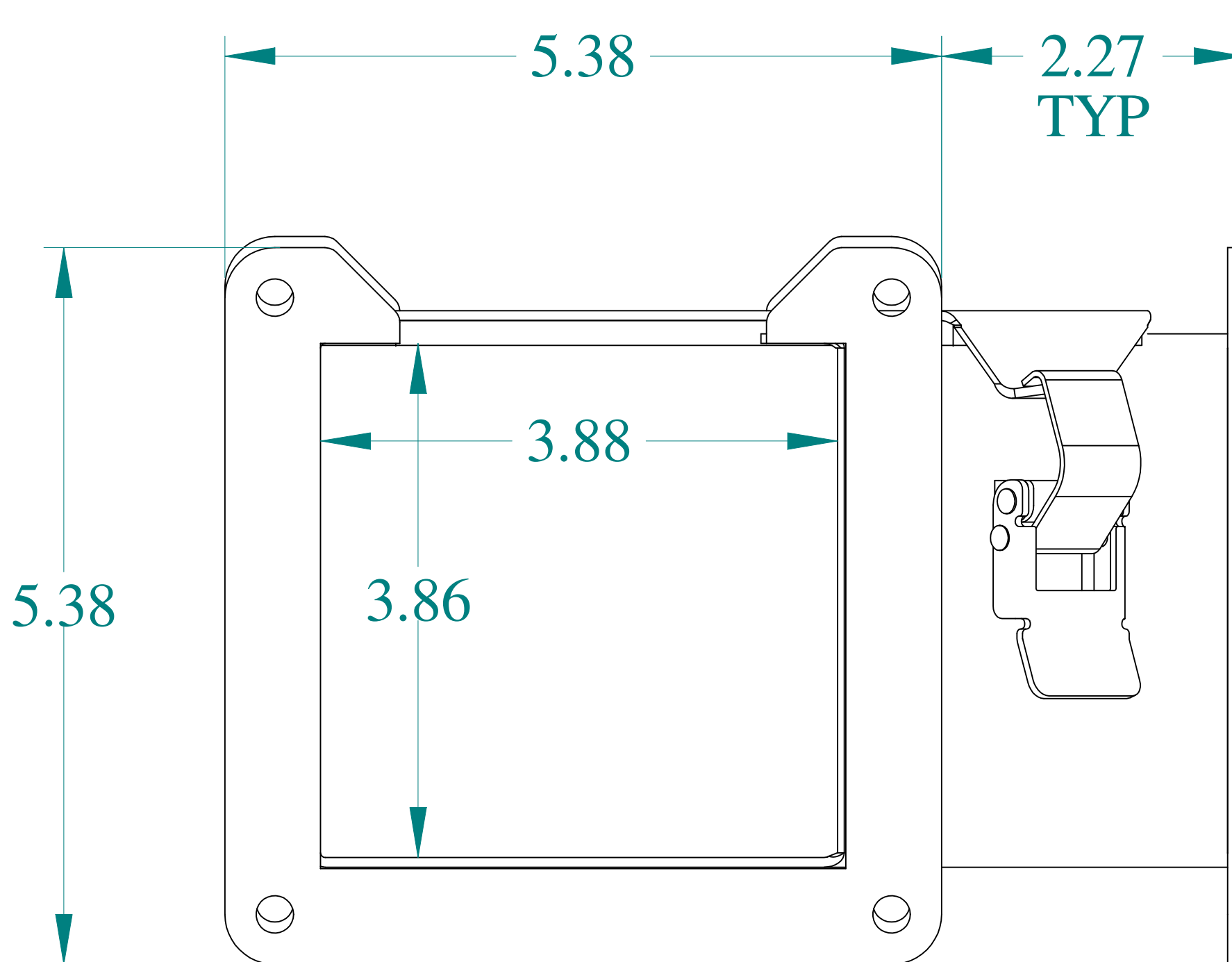
SIDE VIEW
