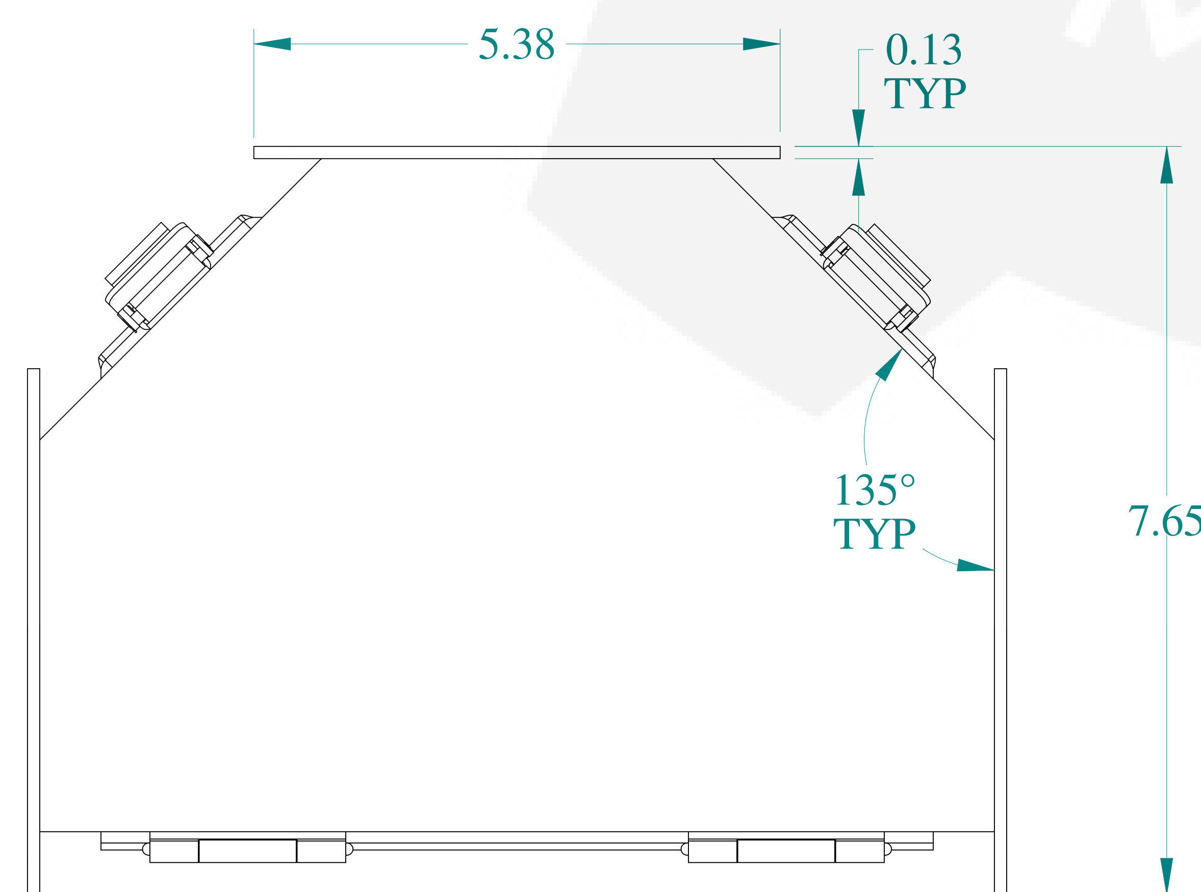
BOTTOM VIEW
