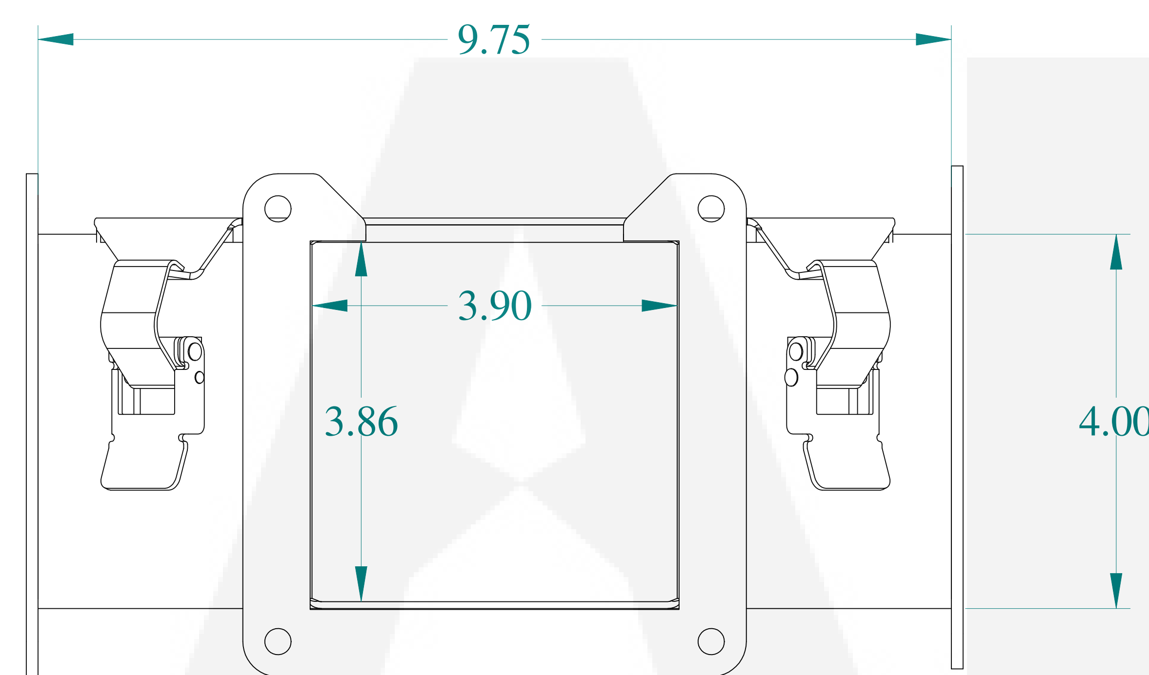
FRONT VIEW
