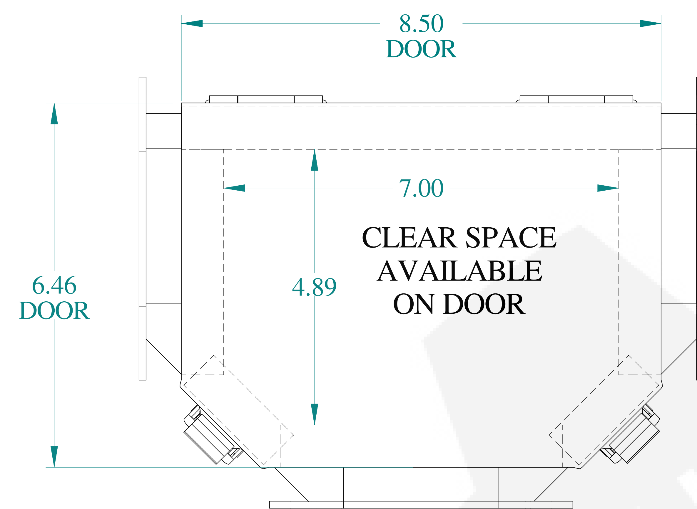
TOP VIEW
