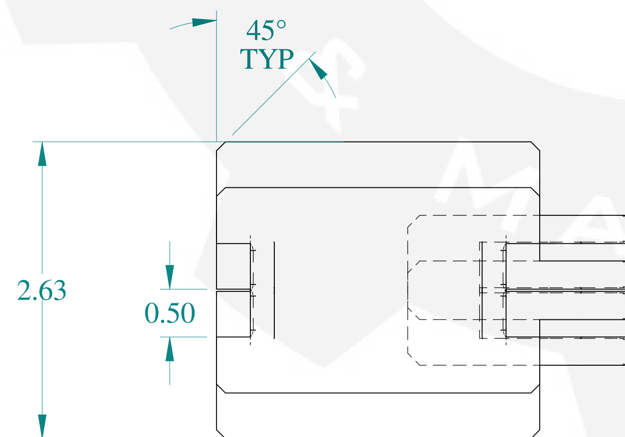
BOTTOM VIEW
