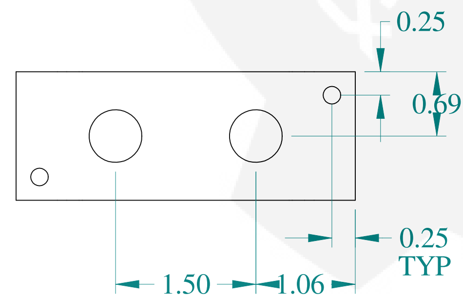
BOTTOM VIEW
