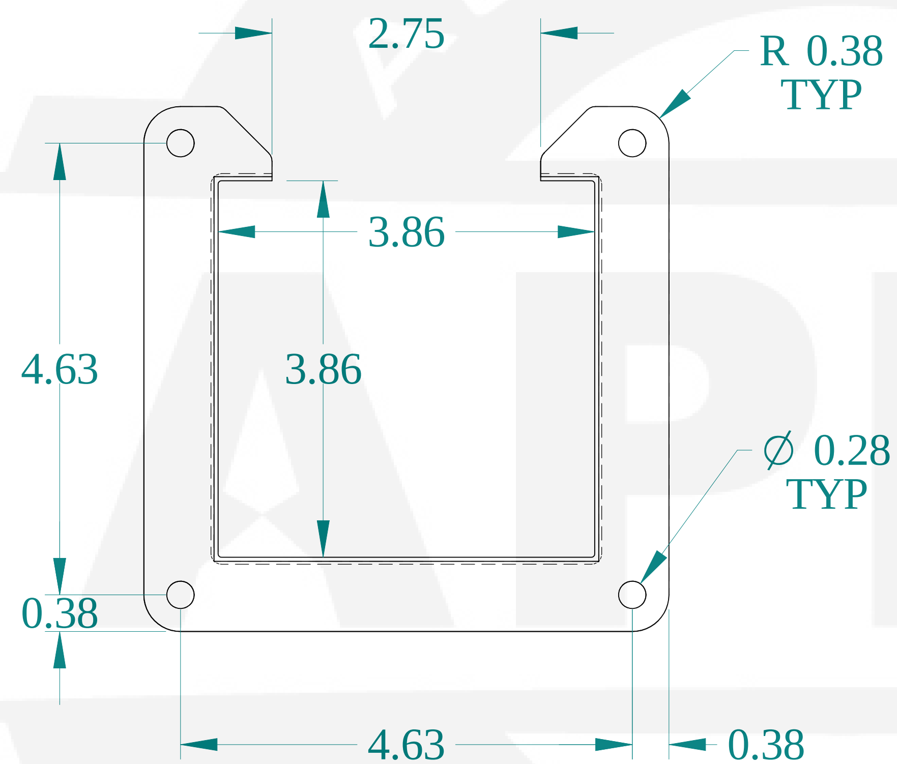
FRONT VIEW
