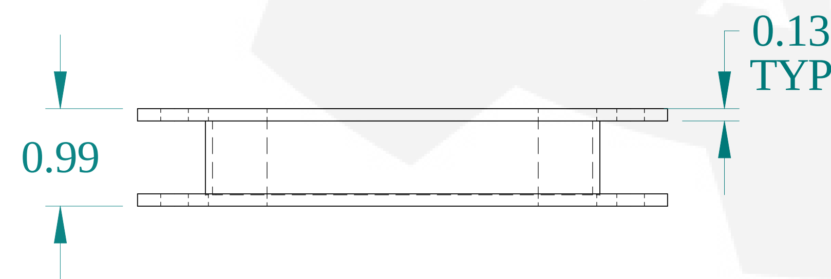
BOTTOM VIEW
