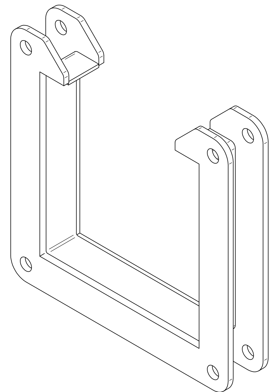
ISOMETRIC VIEWS
