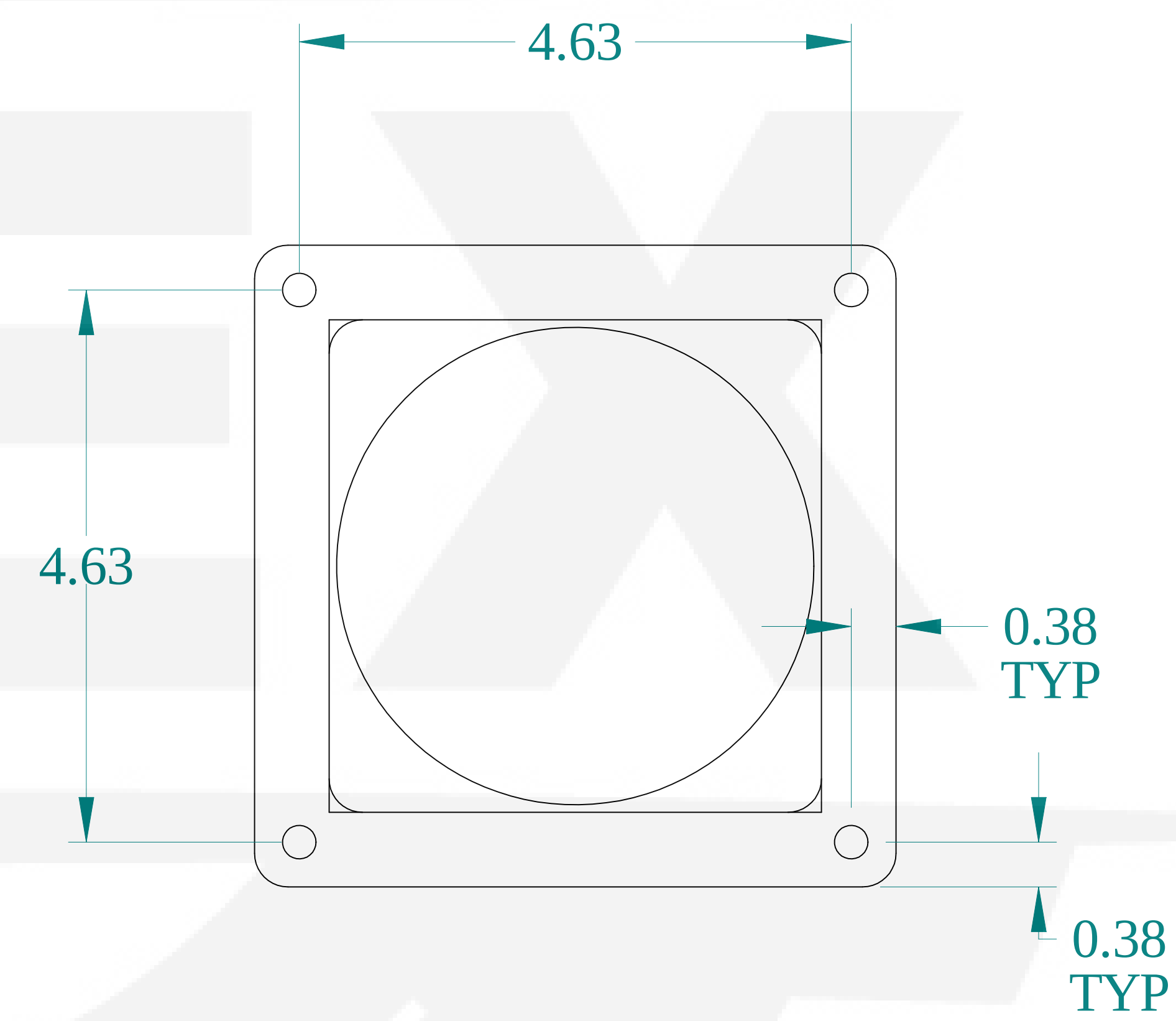
SIDE VIEW
