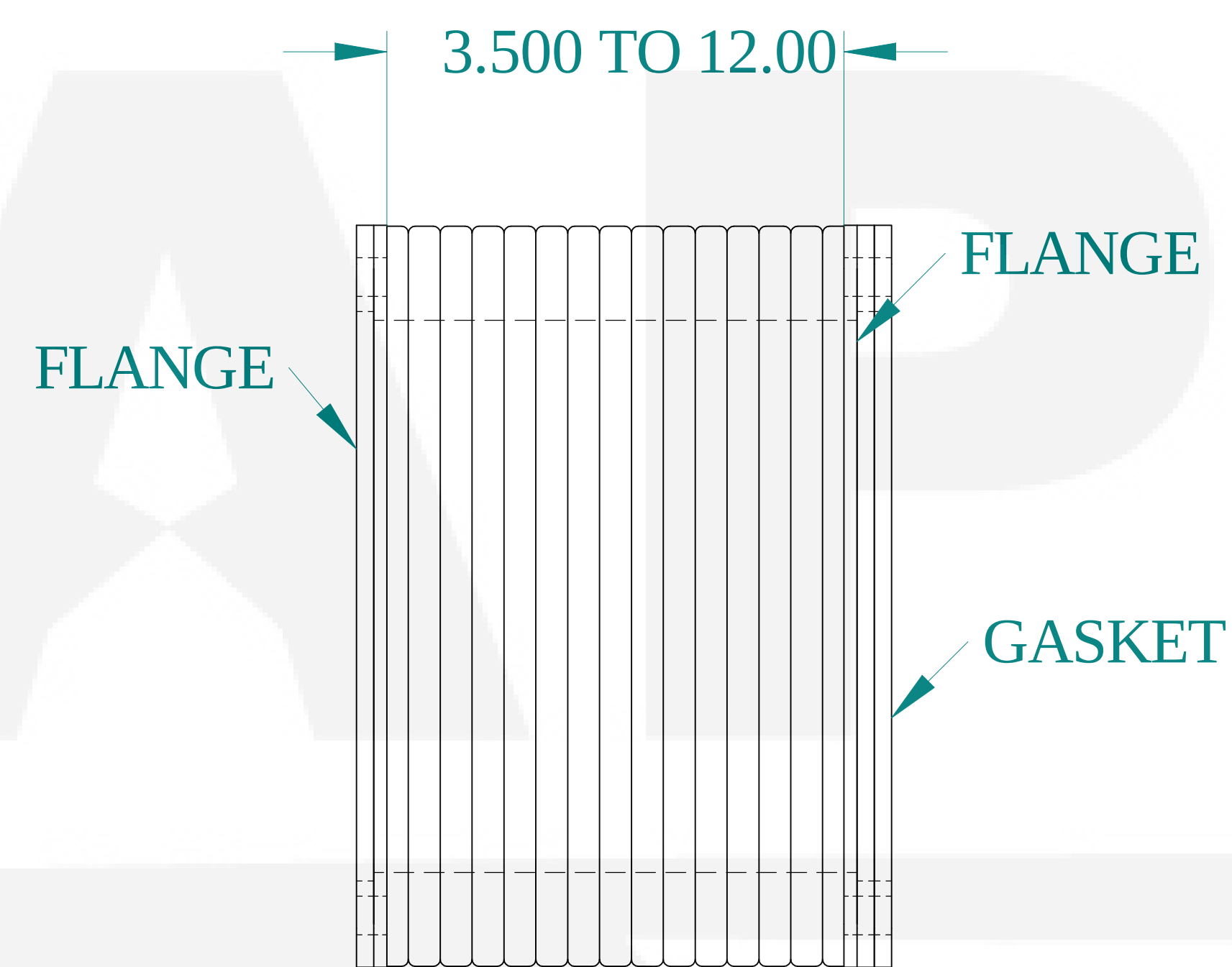
FRONT VIEW
