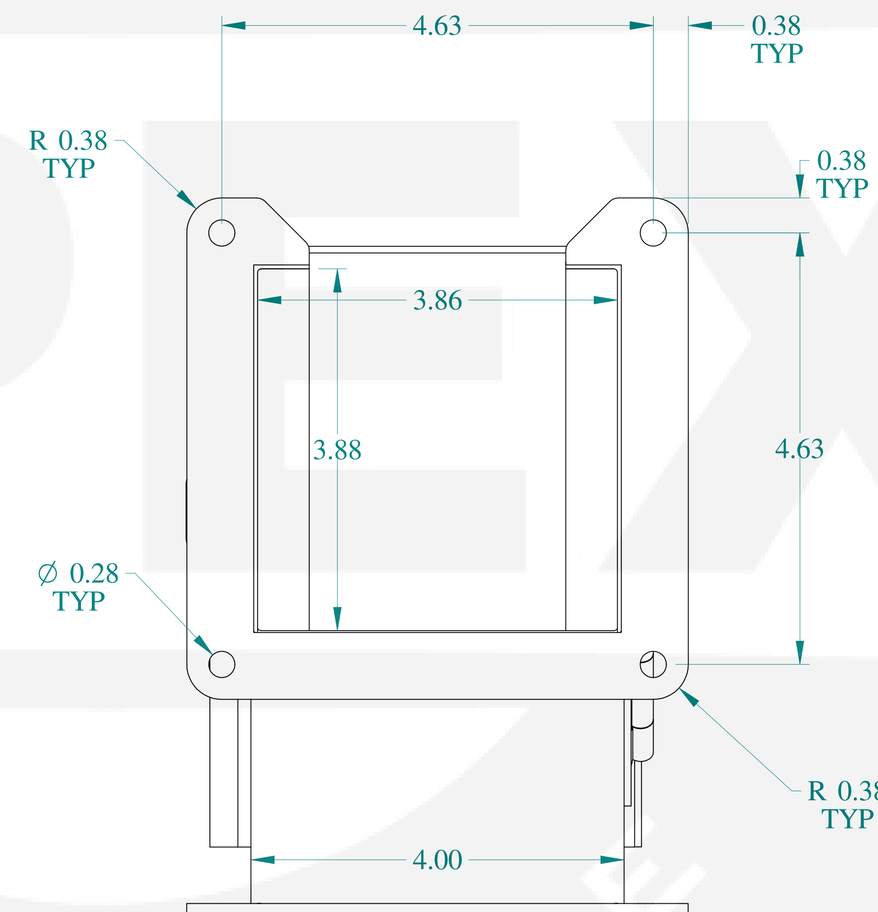
VIEW Z-Z
