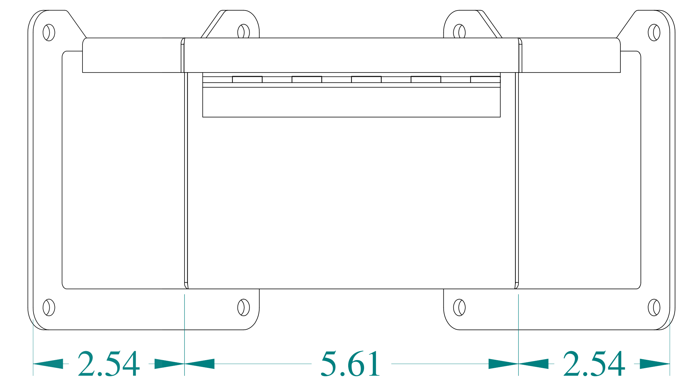
BACK VIEW
