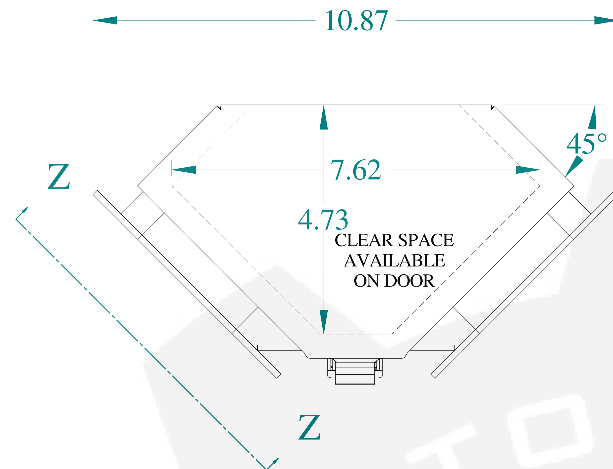
TOP VIEW
