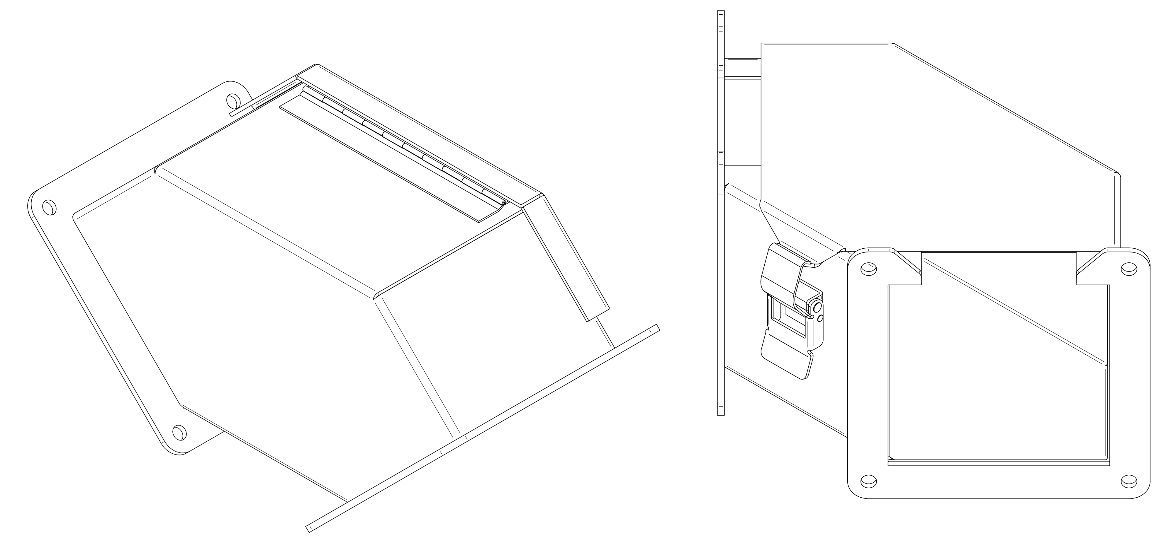
ISOMETRIC VIEWS
