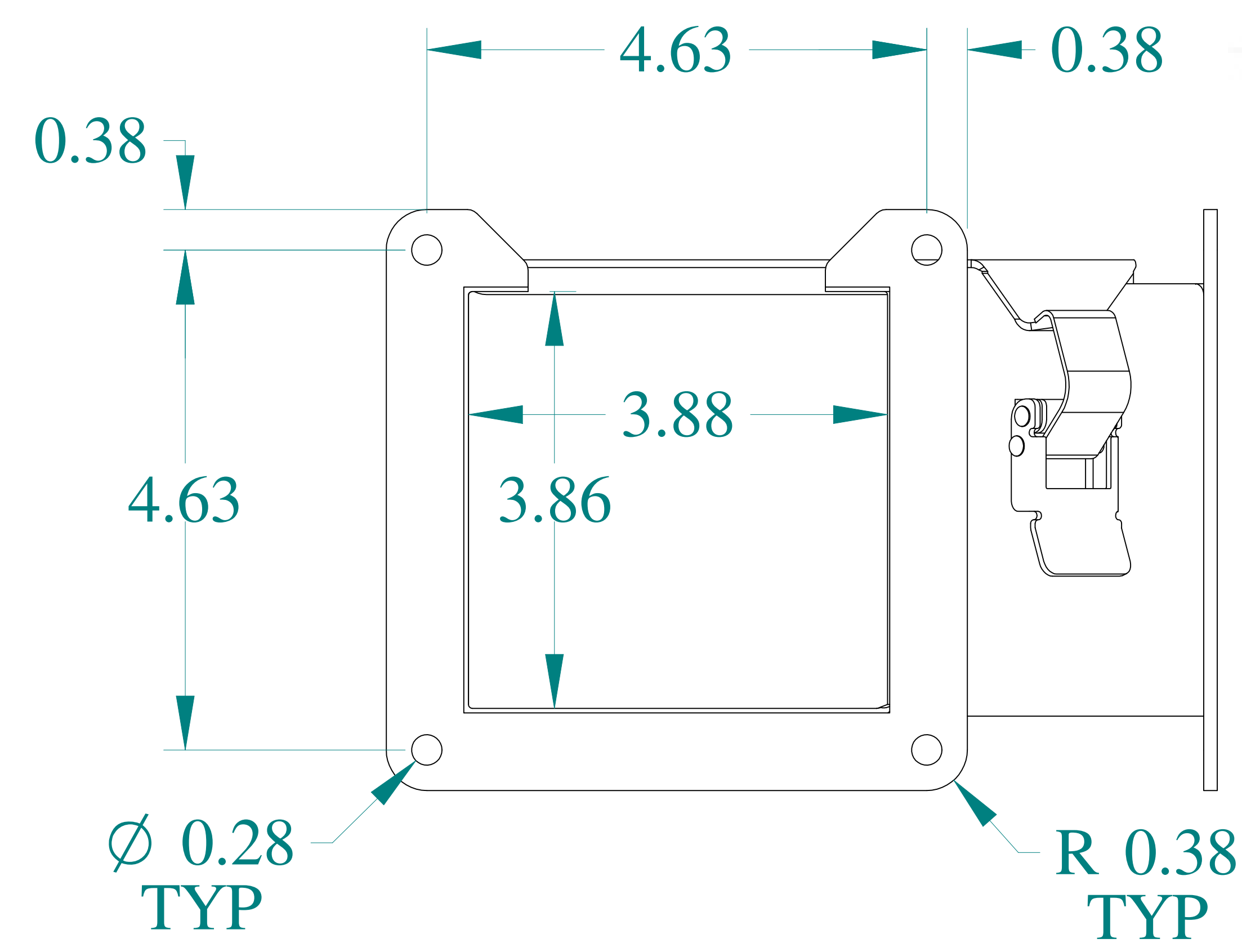
VIEW Z-Z
