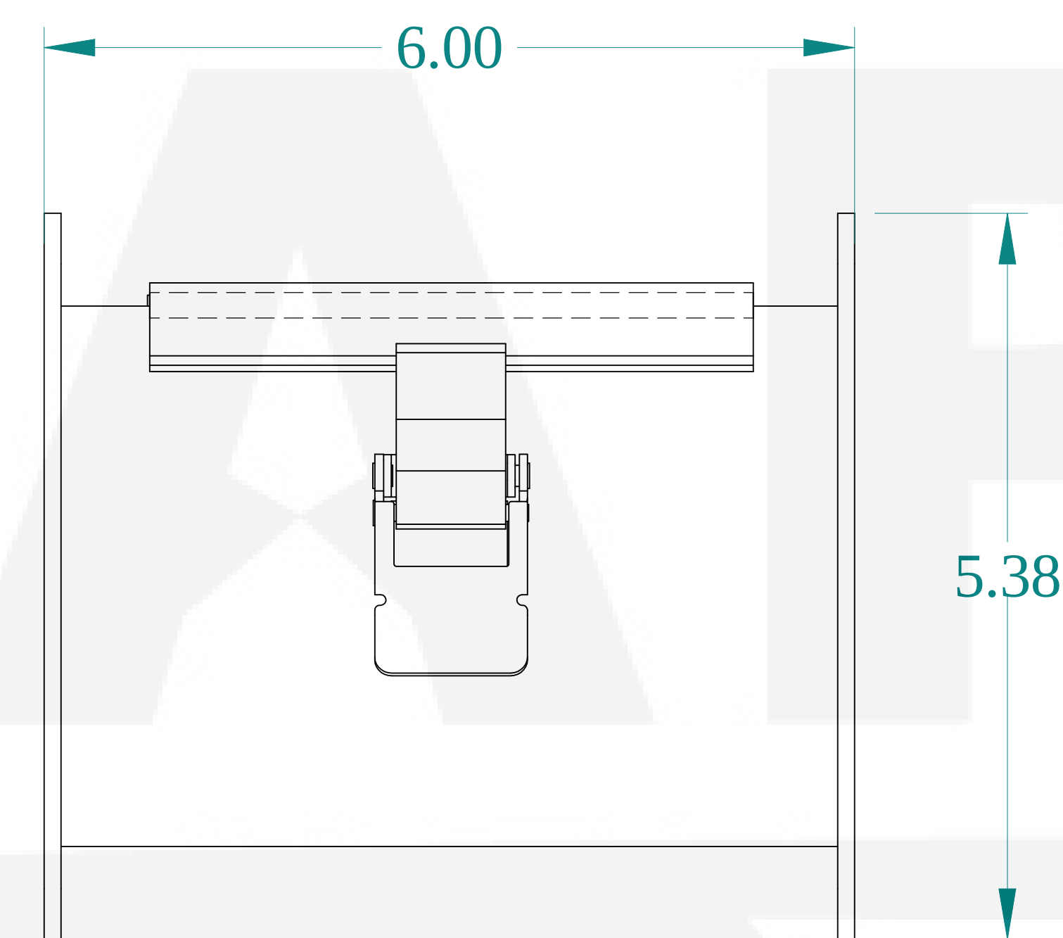
FRONT VIEW
