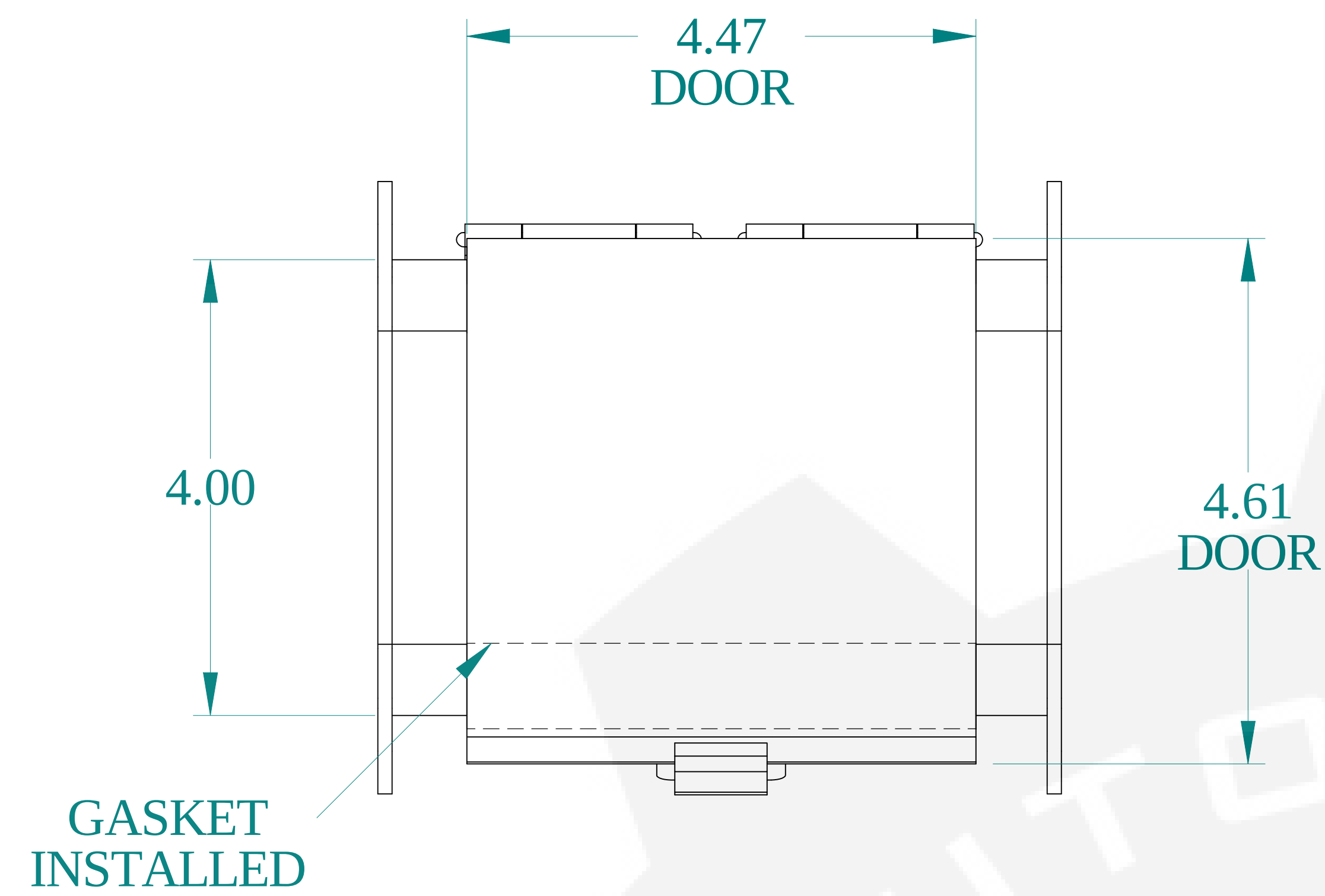
TOP VIEW
