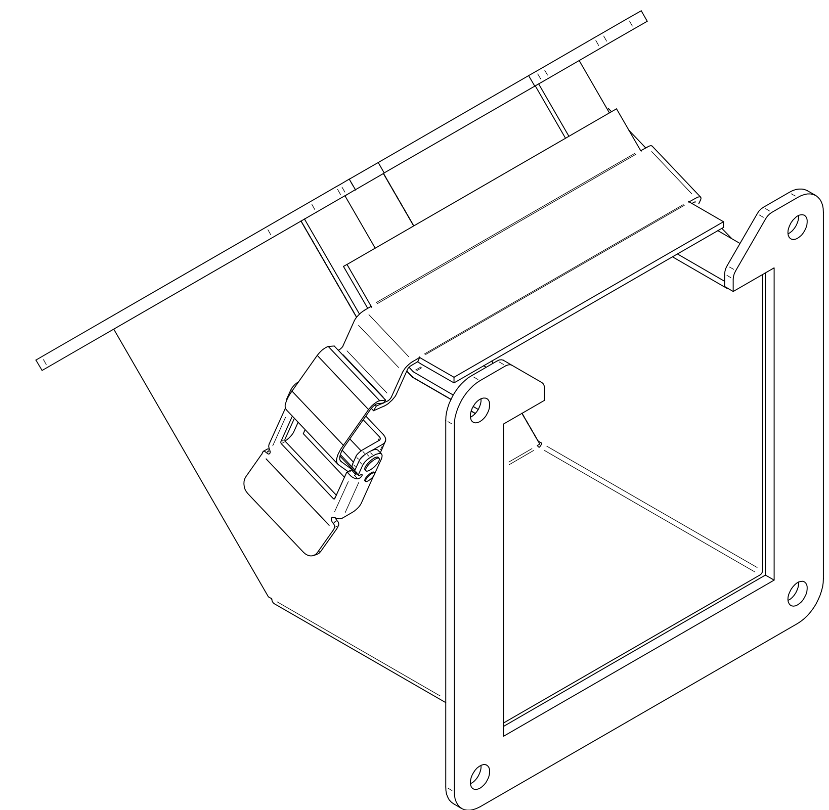
ISOMETRIC VIEWS
