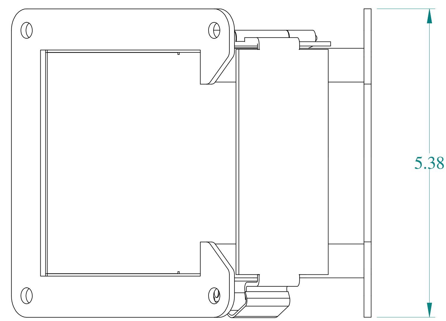
TOP VIEW
