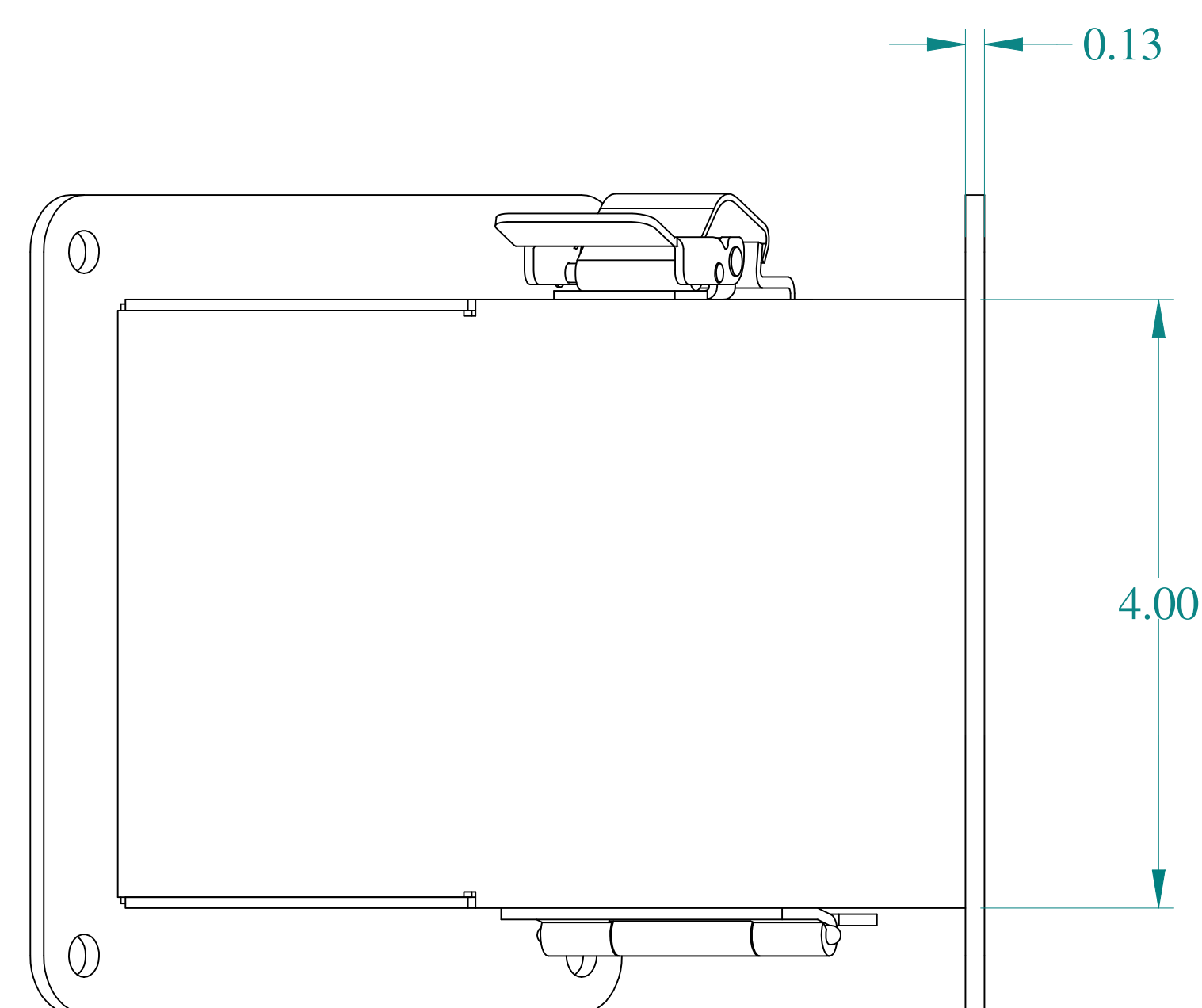
BOTTOM VIEW
