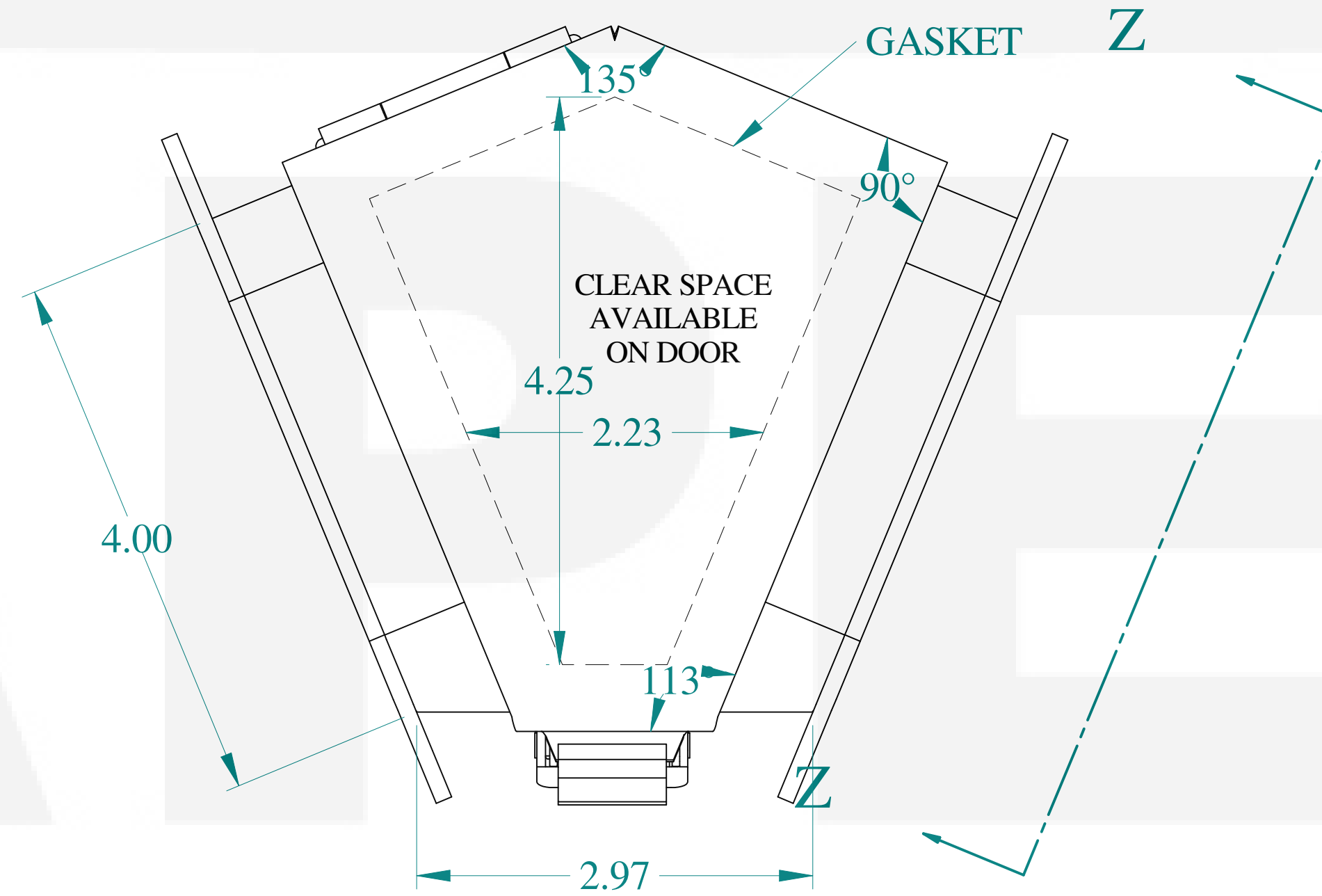
FRONT VIEW
