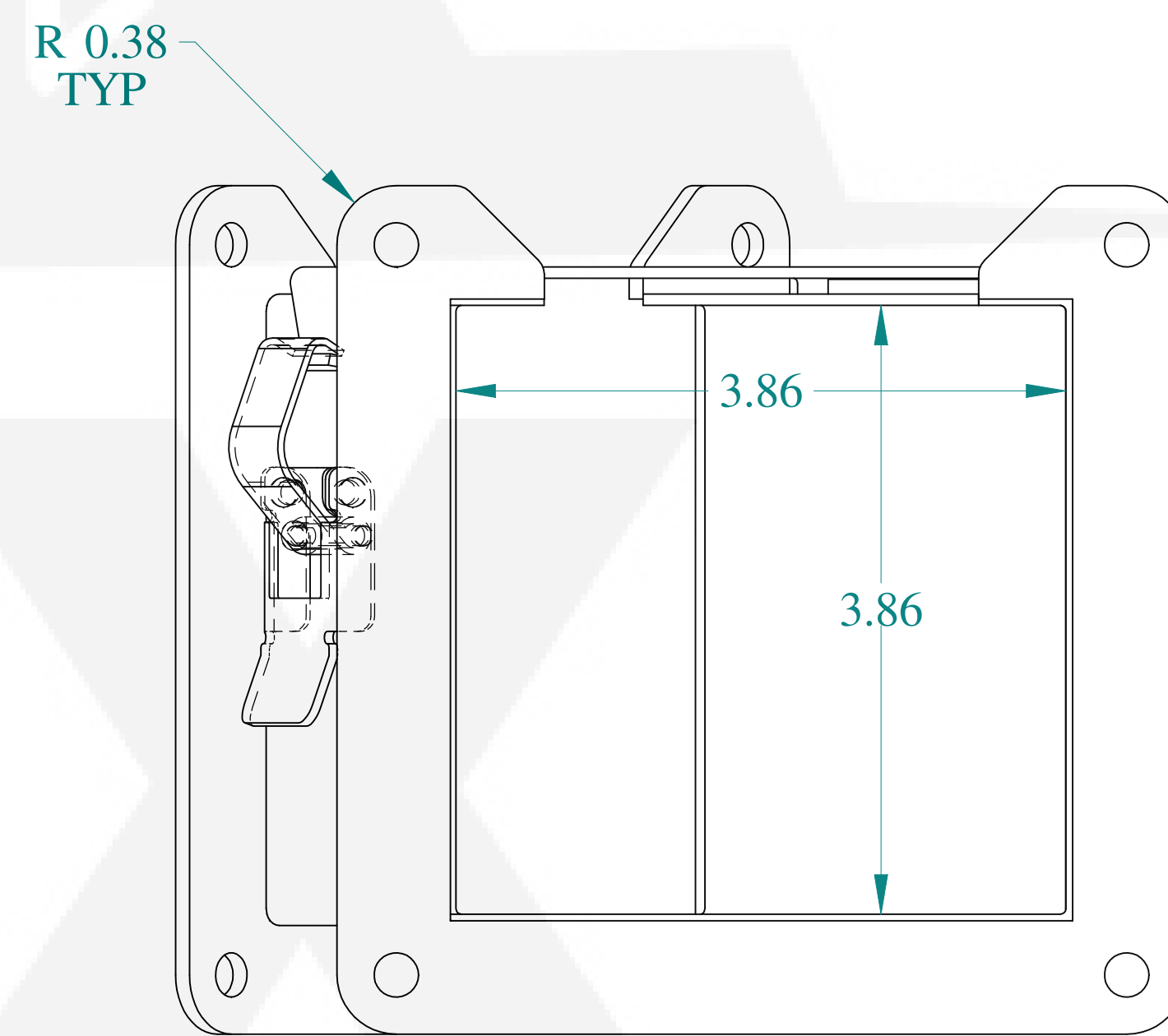
VIEW Z-Z
