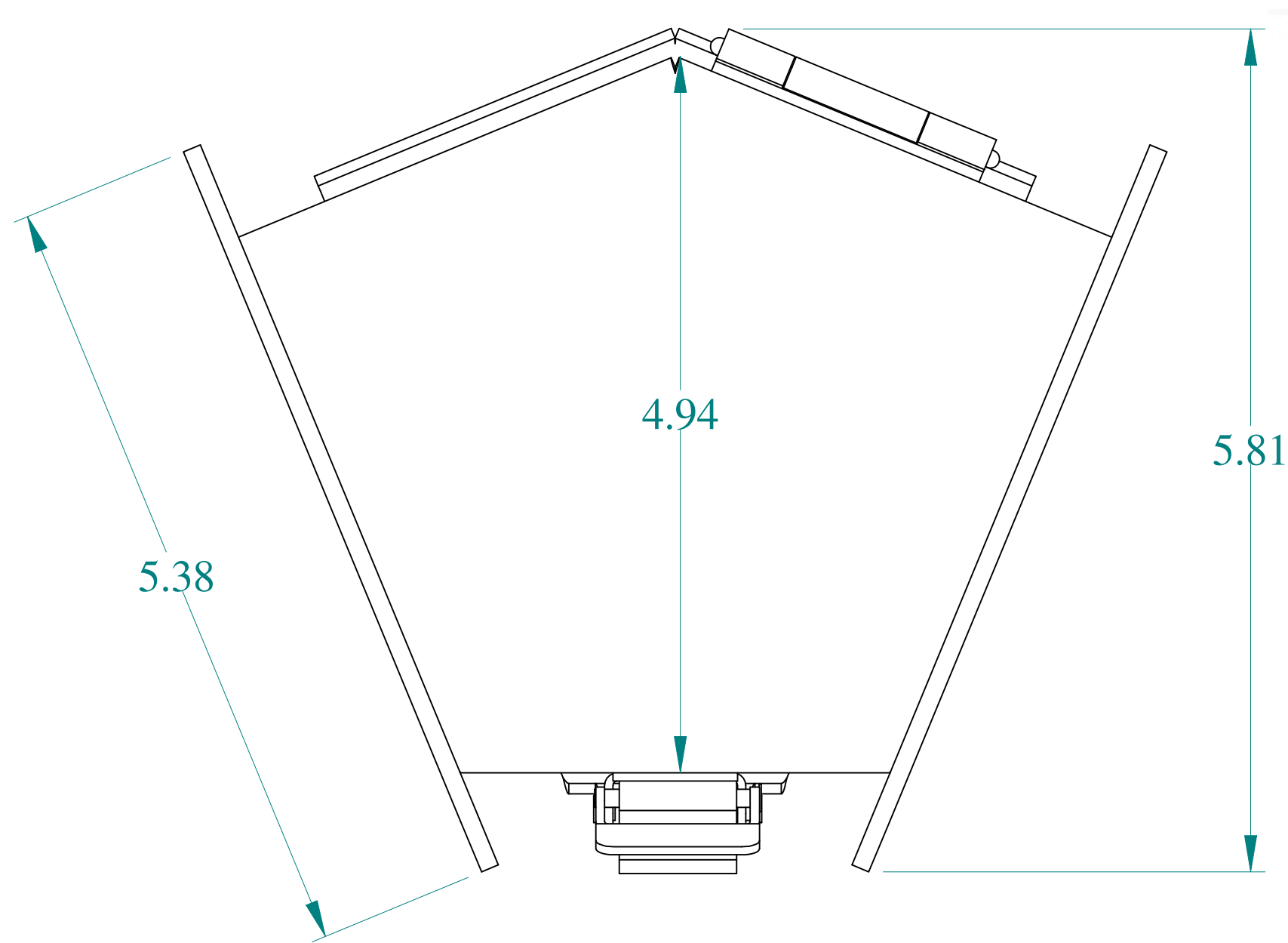
BACK VIEW
