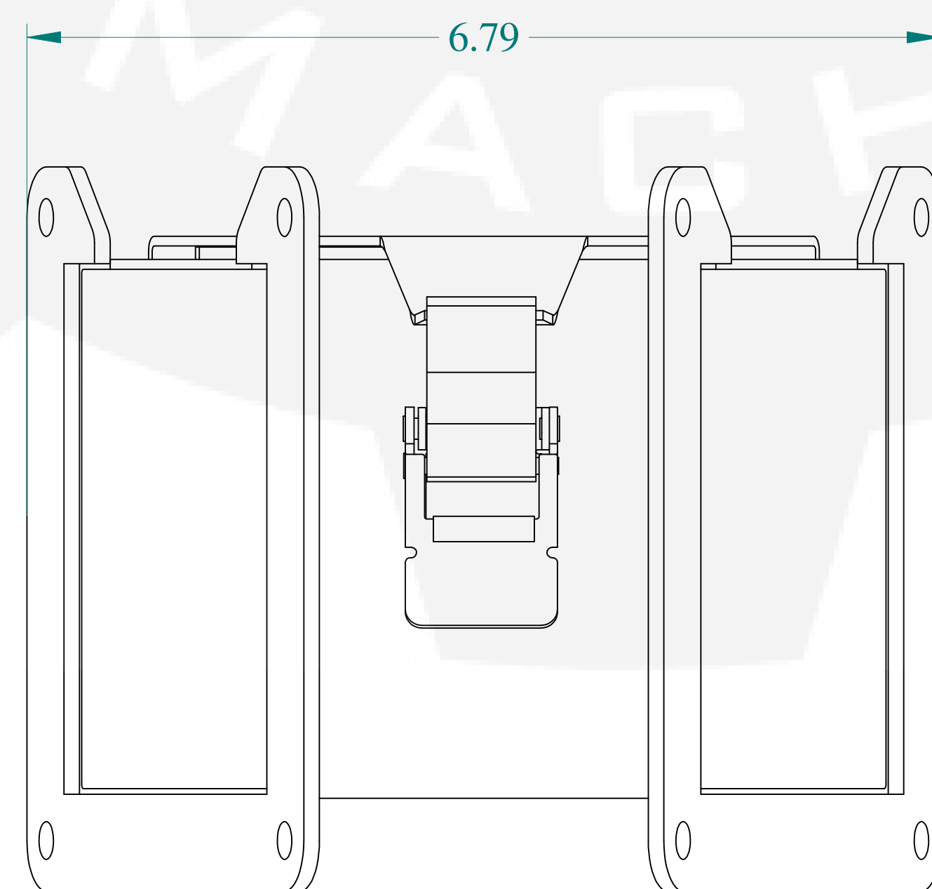
BOTTOM VIEW
