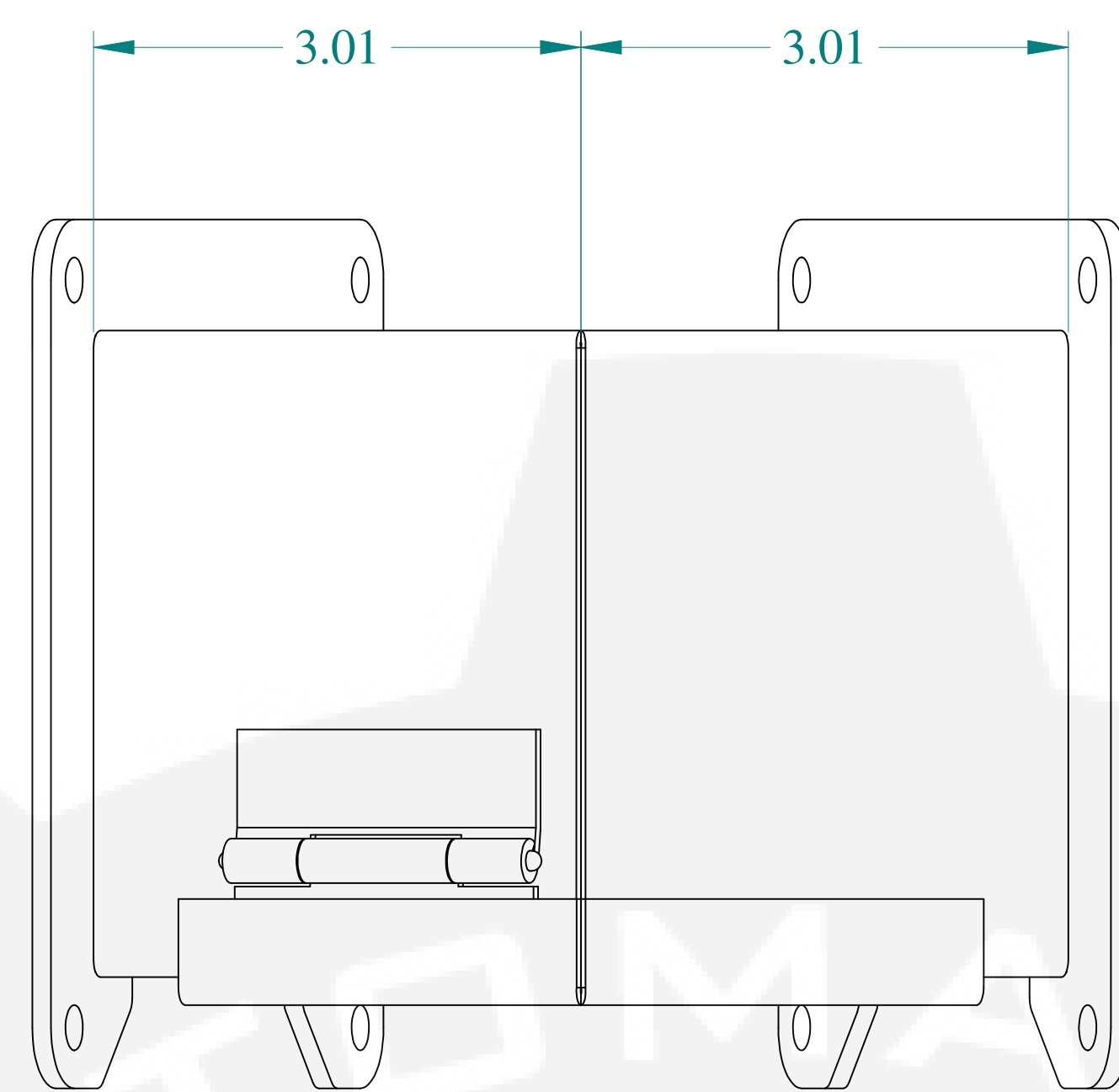
TOP VIEW
