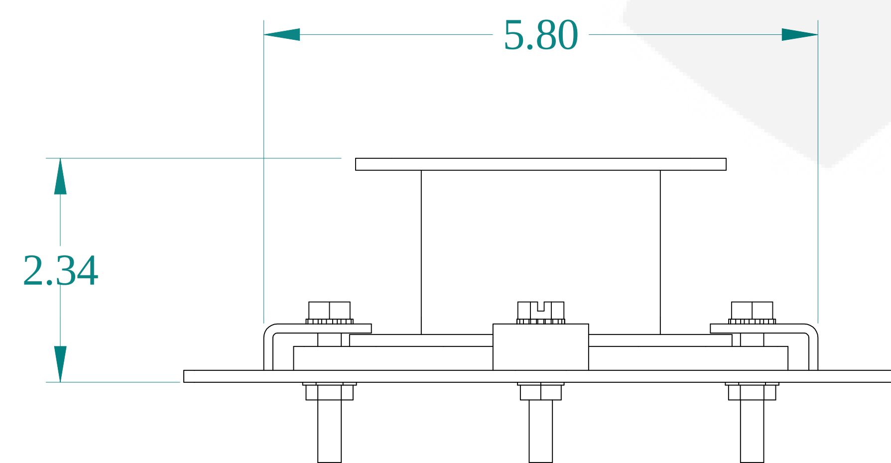
BOTTOM VIEW
