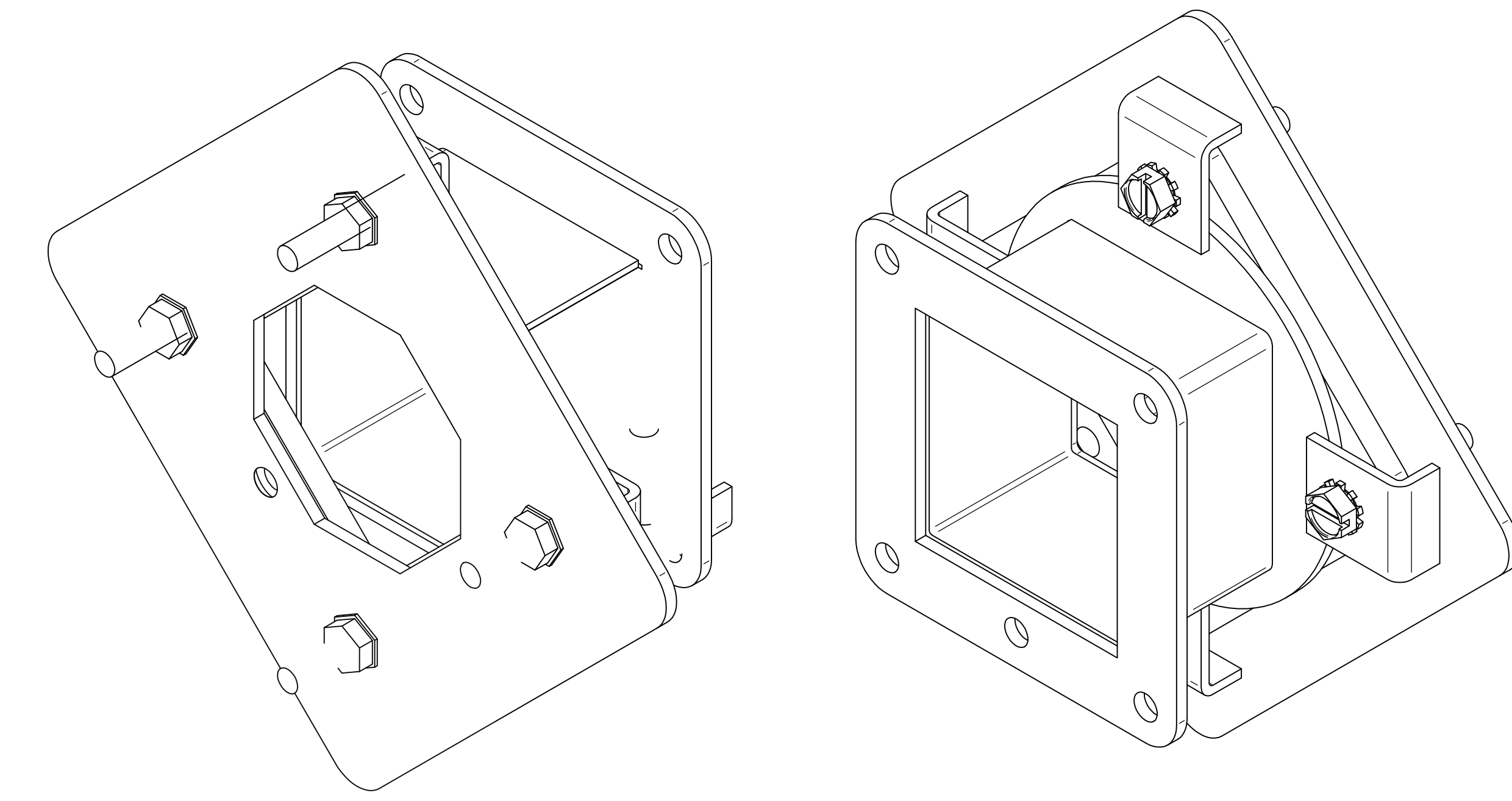
ISOMETRIC VIEWS
