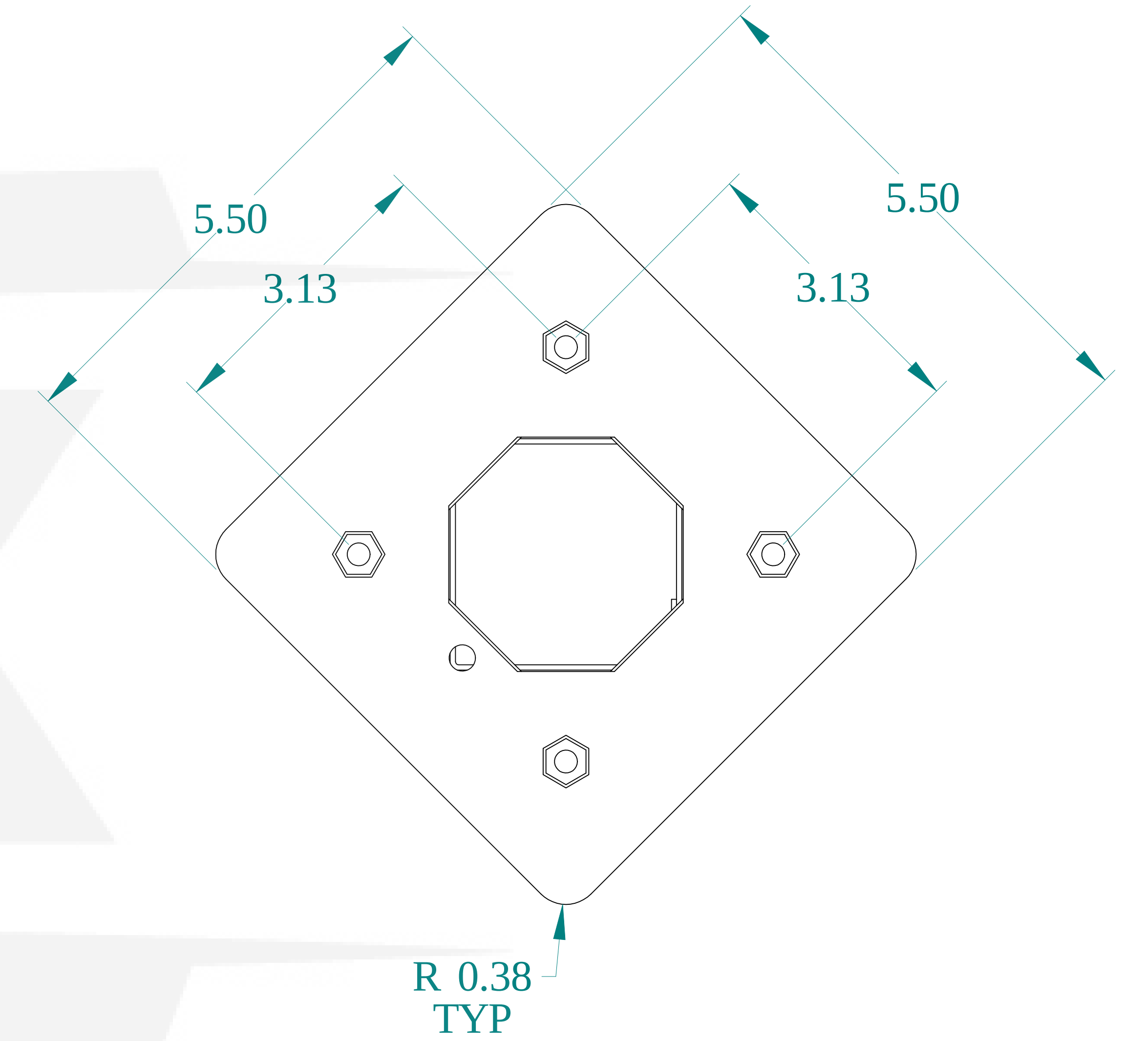
BACK VIEW
