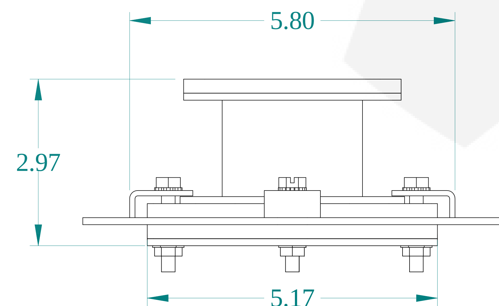
BOTTOM VIEW
