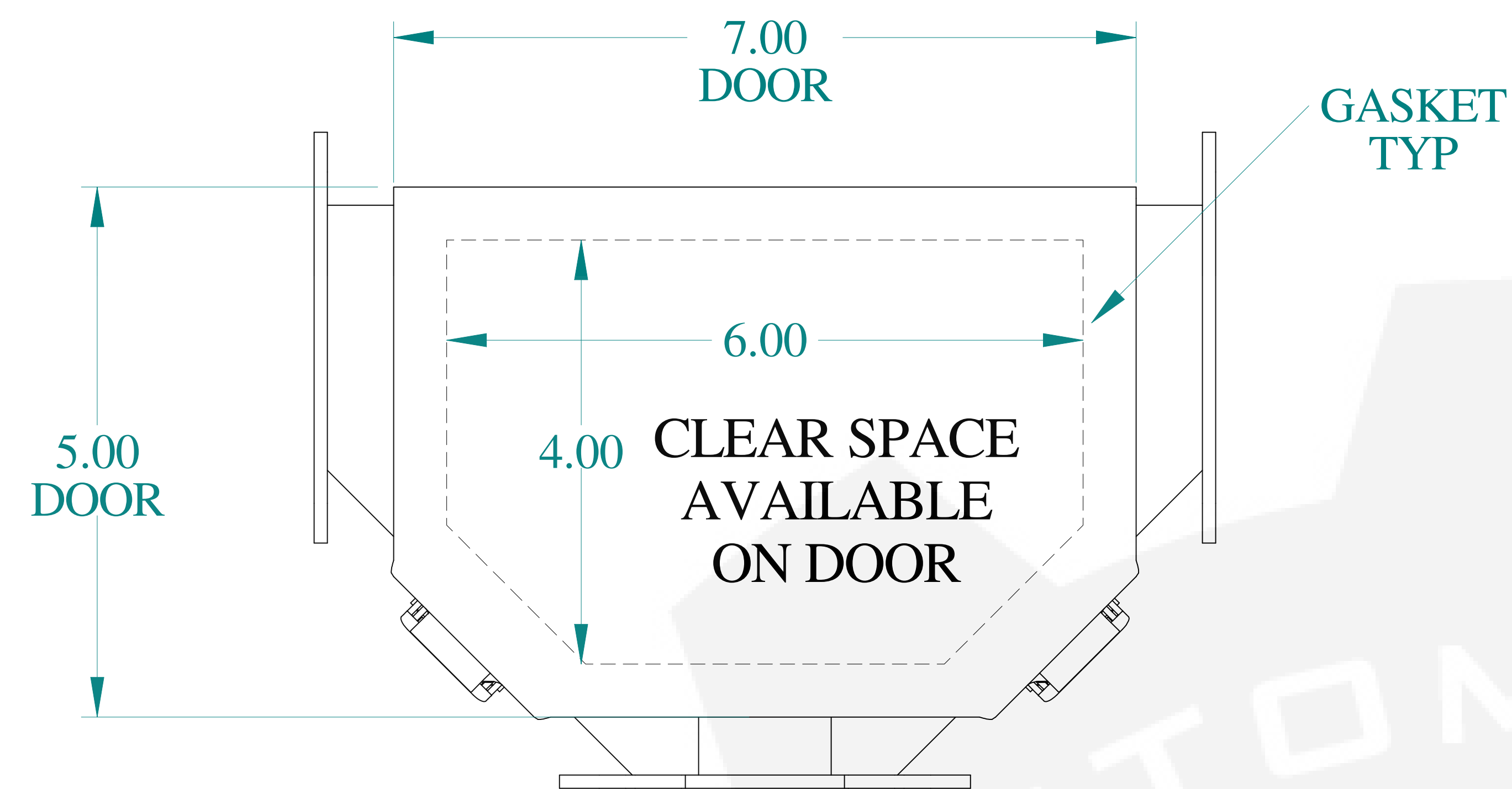
TOP VIEW
