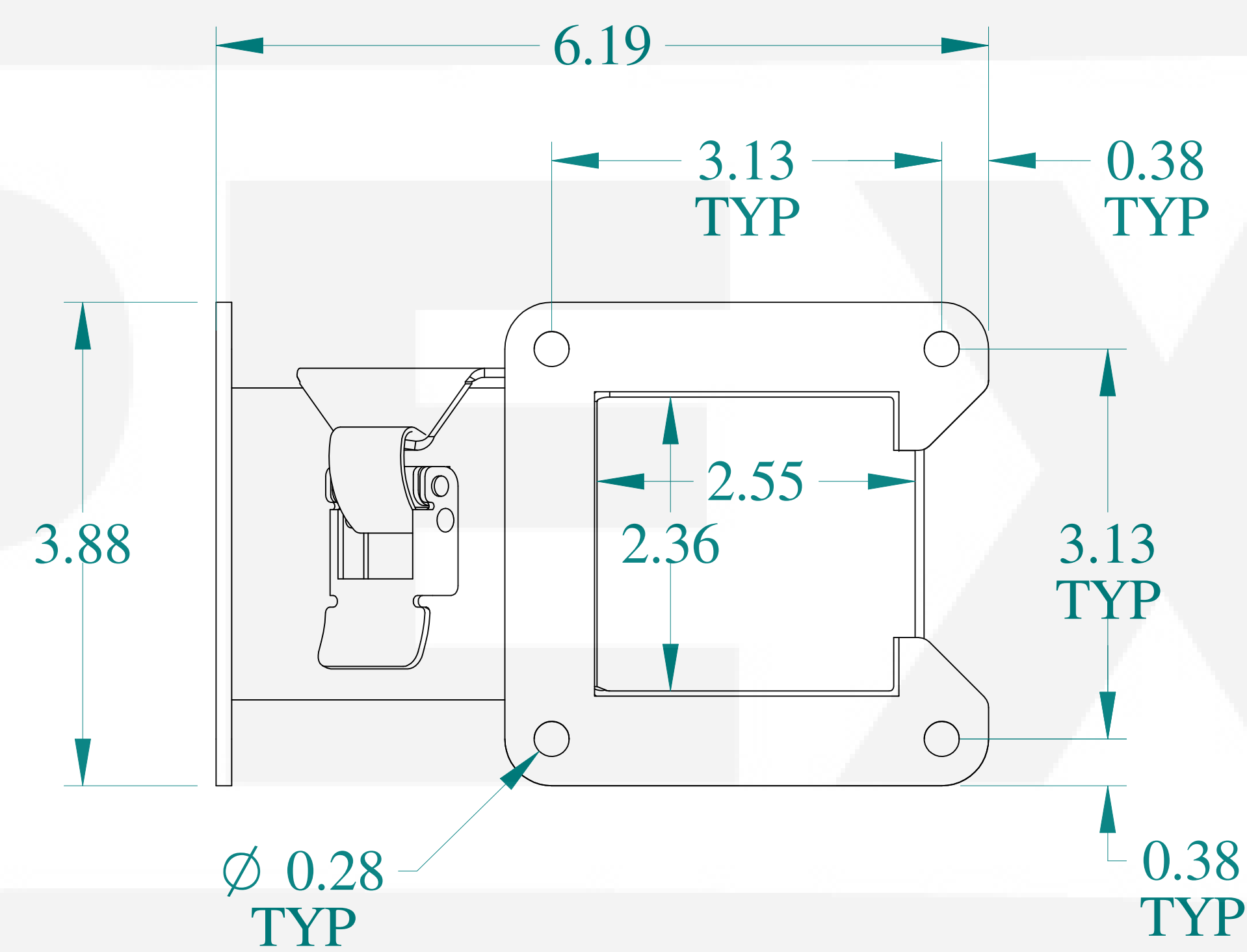
SIDE VIEW
