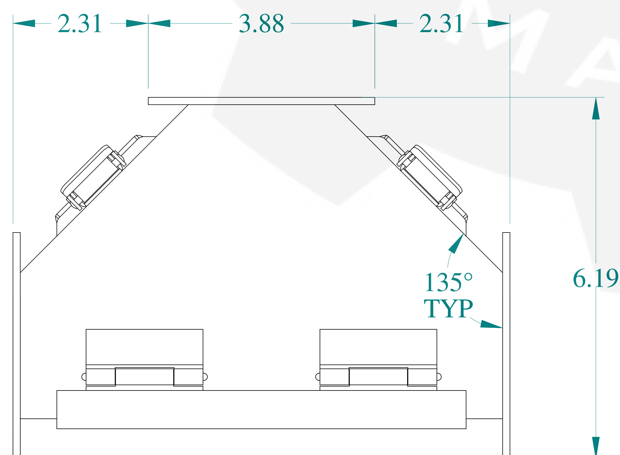
BOTTOM VIEW
