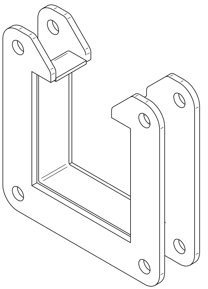
ISOMETRIC VIEWS
