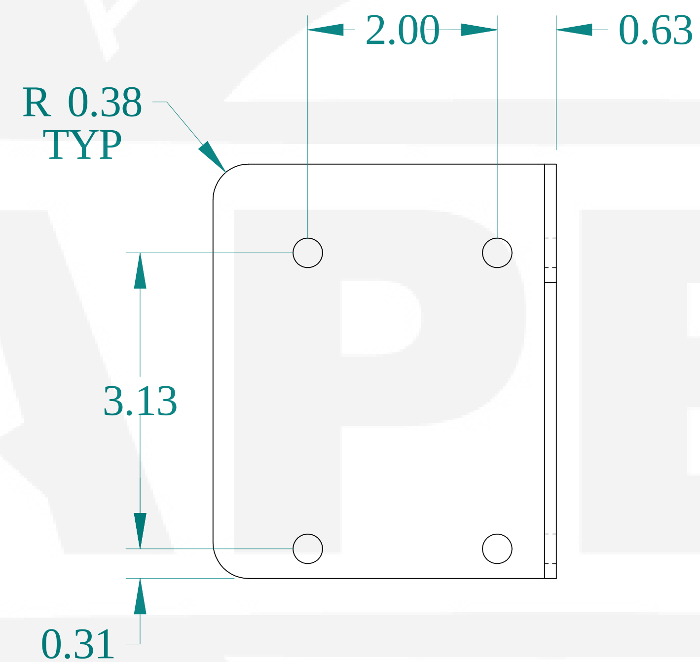
SIDE VIEW
