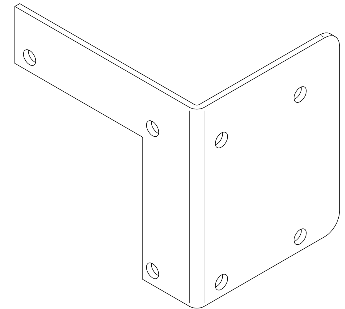
ISOMETRIC VIEWS
