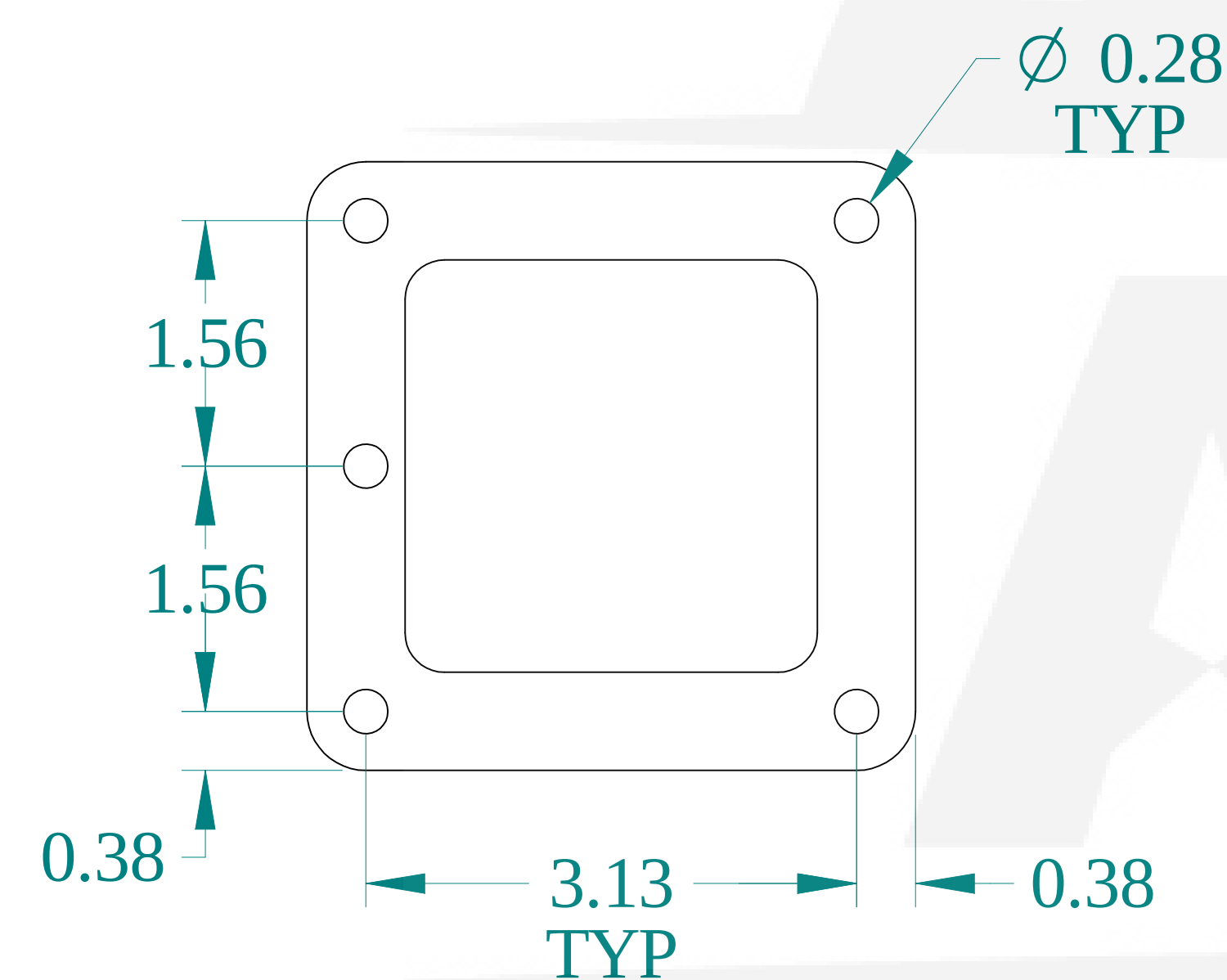
FRONT VIEW
