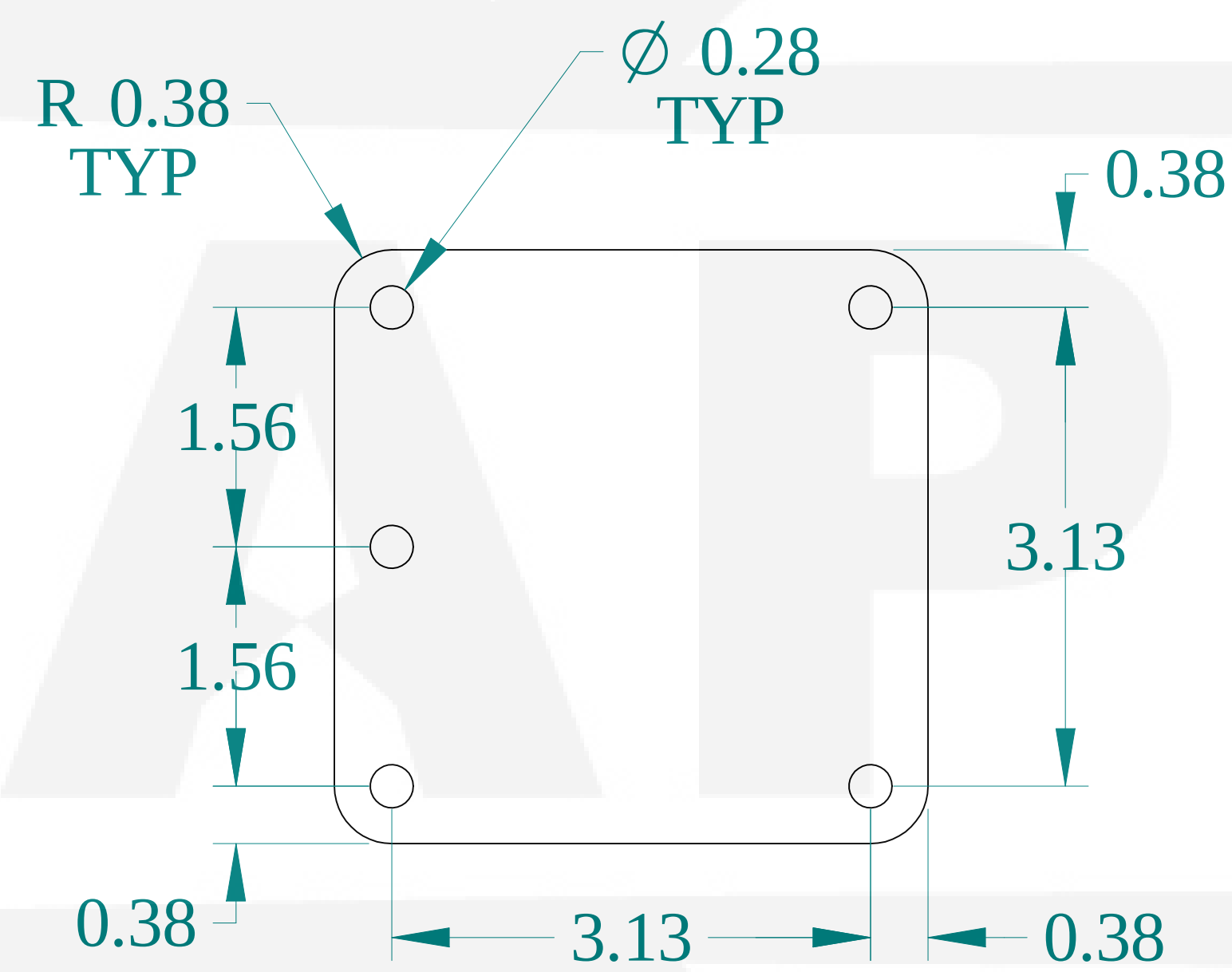
FRONT VIEW
