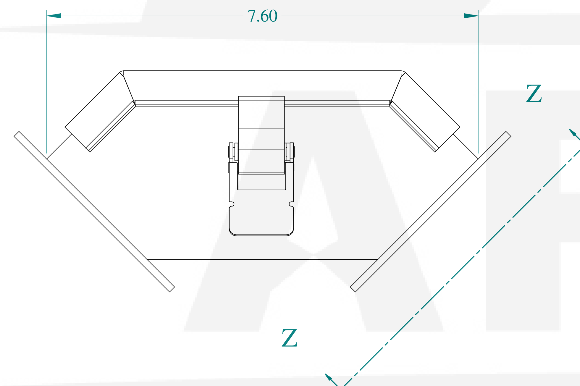
FRONT VIEW
