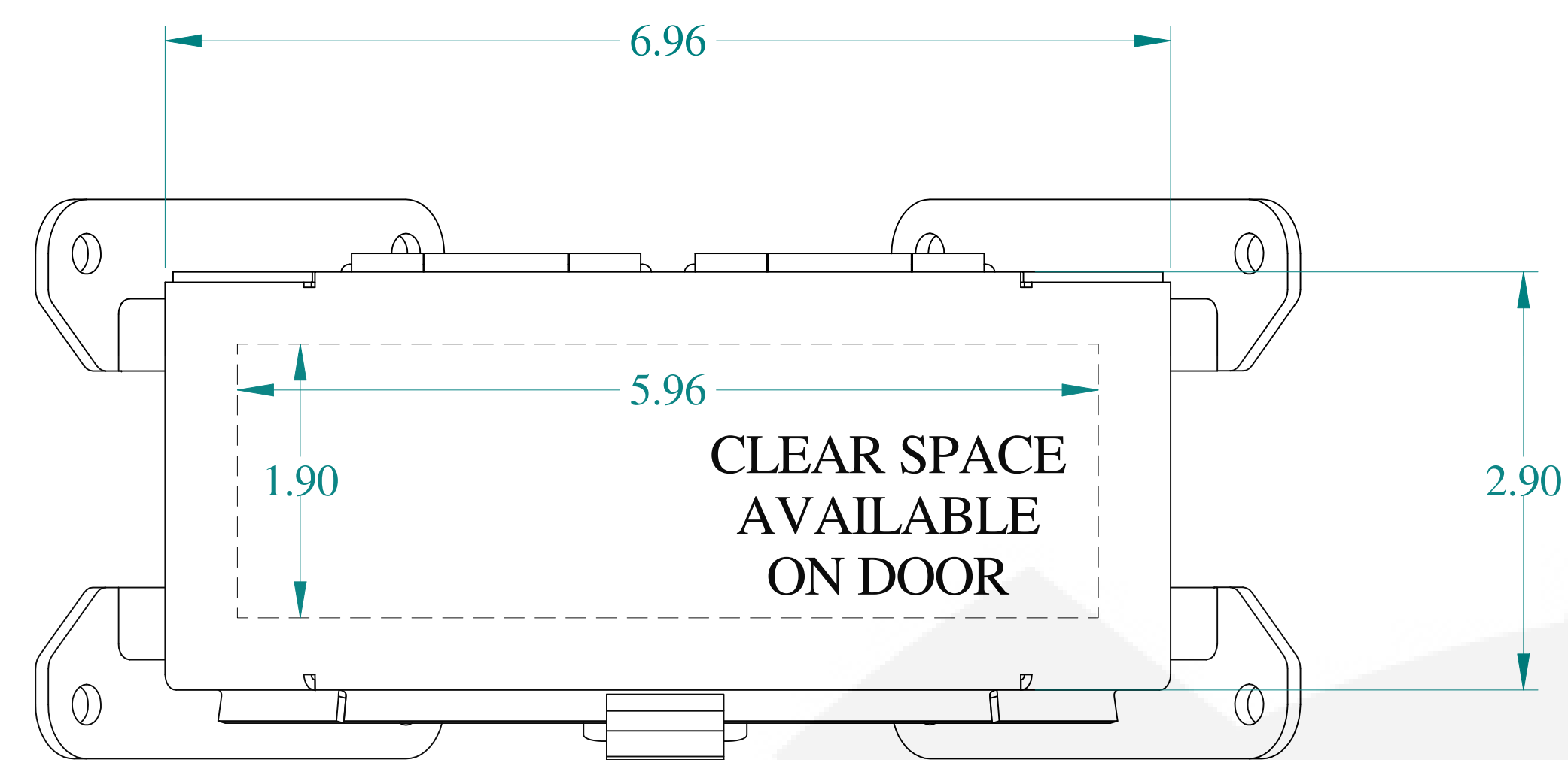
TOP VIEW
