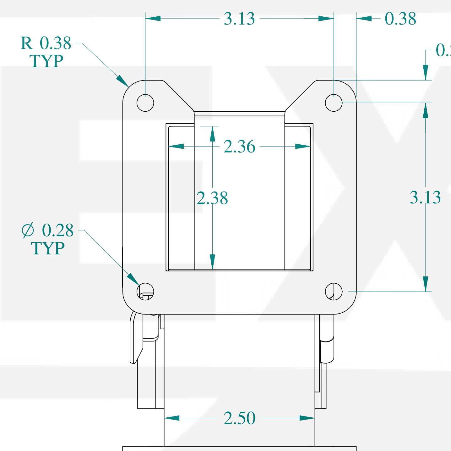
VIEW Z-Z
