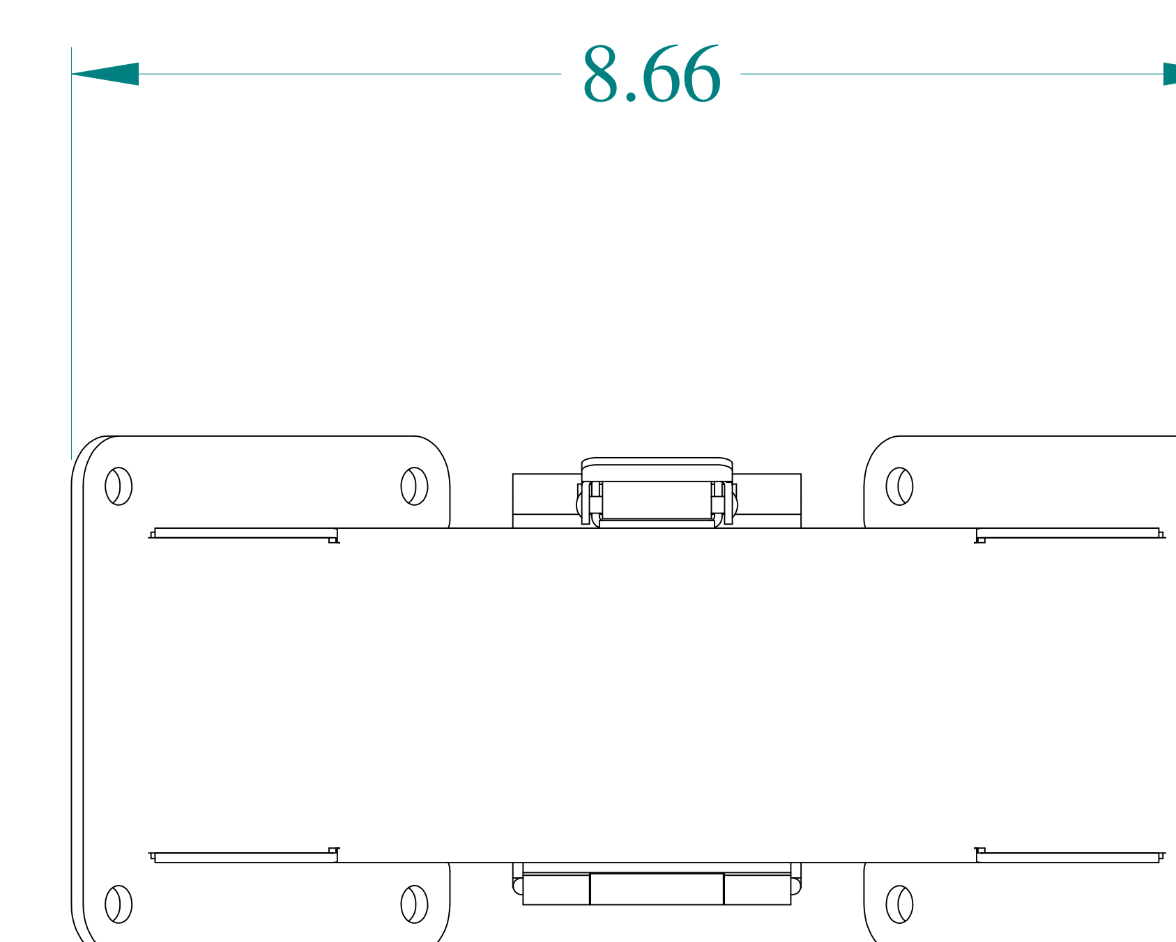
BACK VIEW
