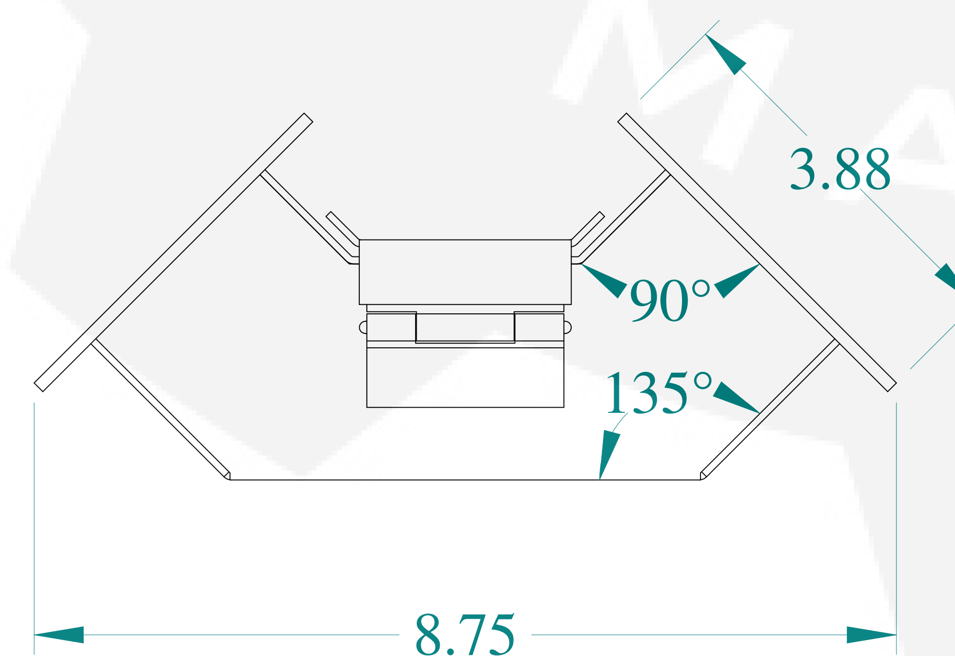
BOTTOM VIEW
