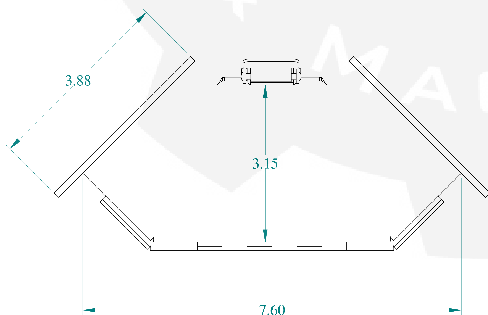
BOTTOM VIEW
