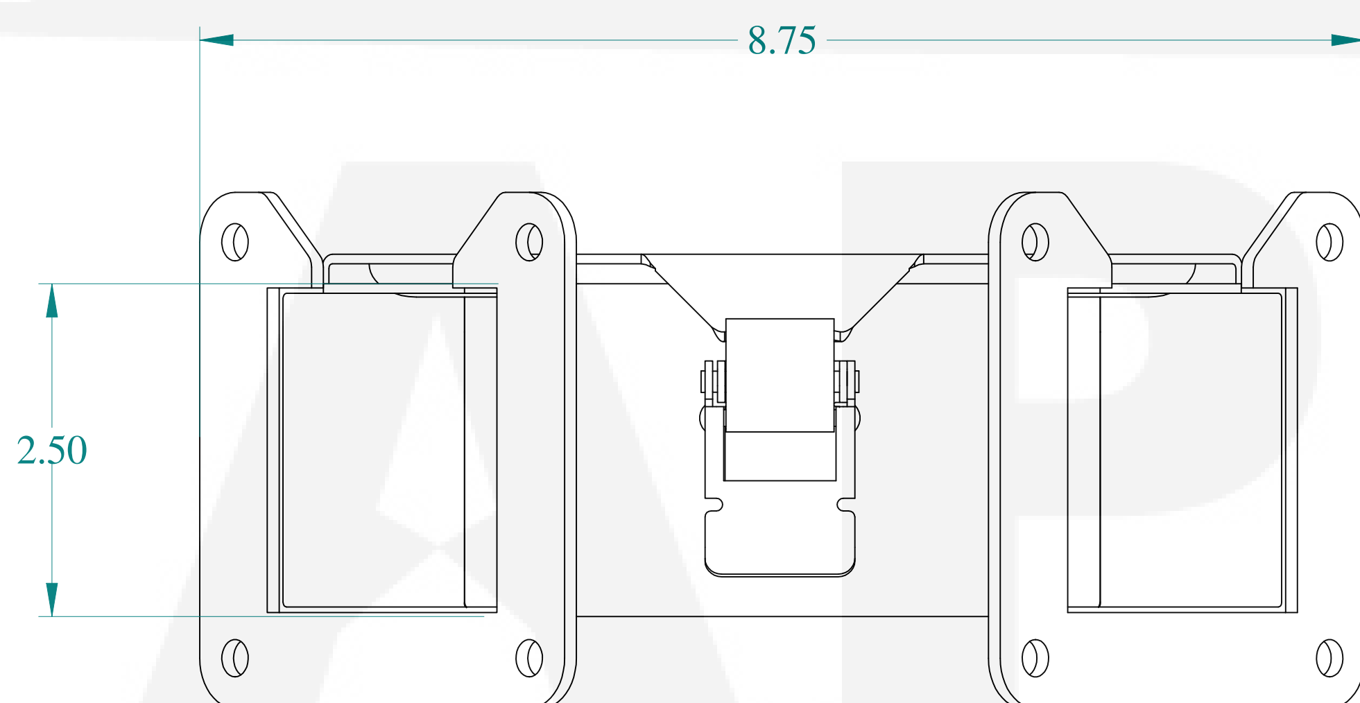
FRONT VIEW
