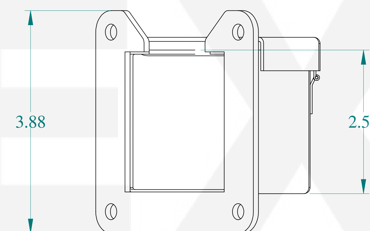
SIDE VIEW
