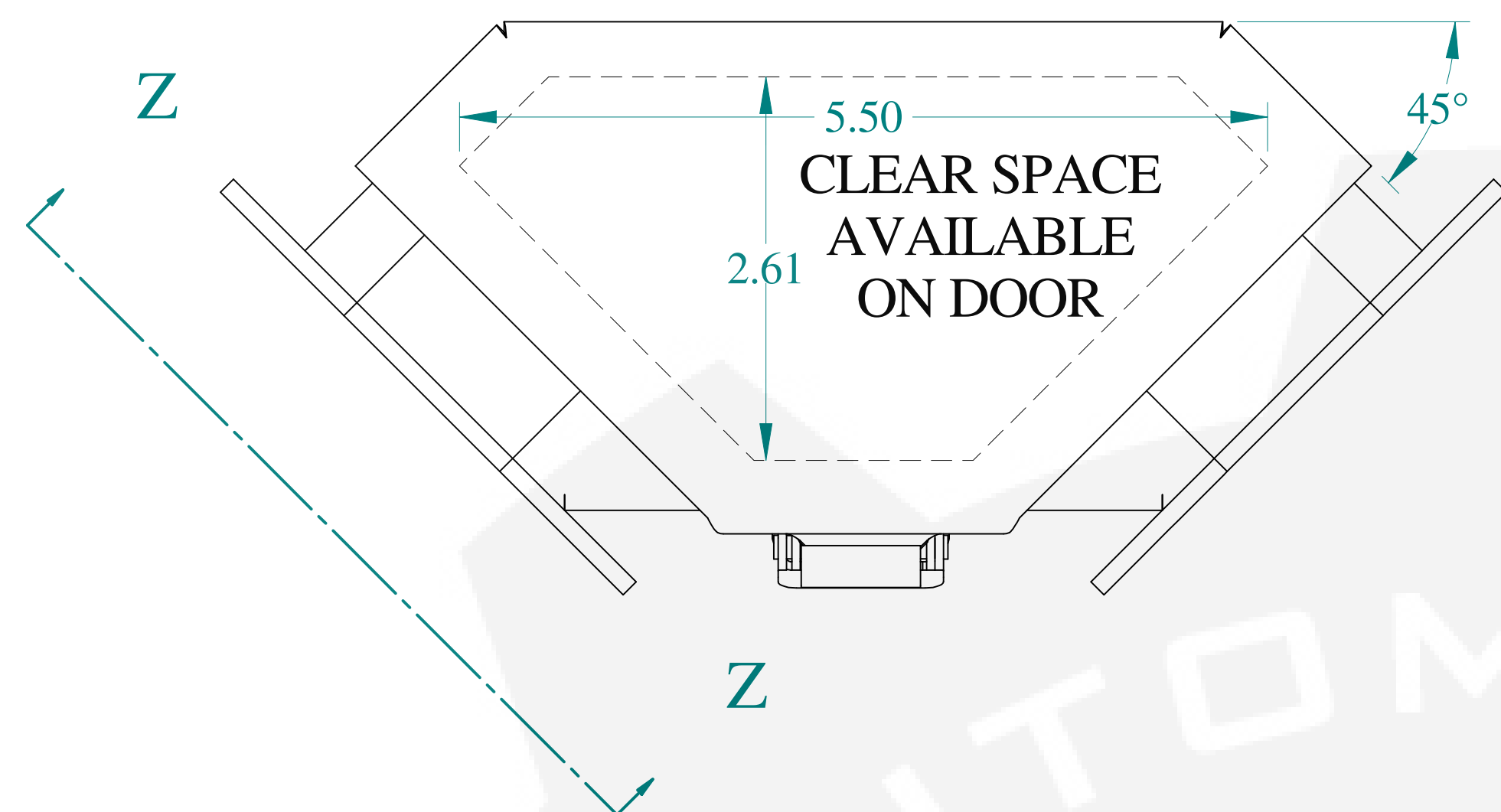
TOP VIEW
