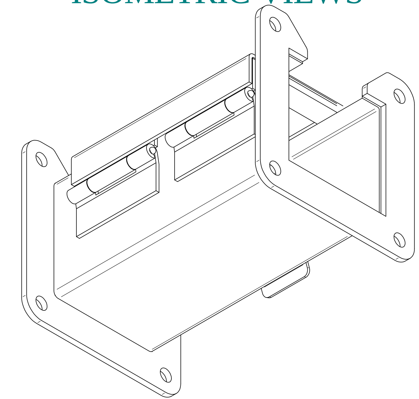
ISOMETRIC VIEWS
