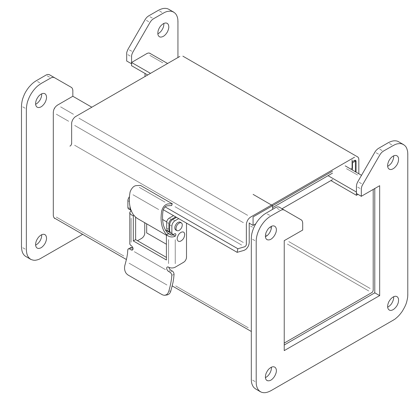
ISOMETRIC VIEWS
