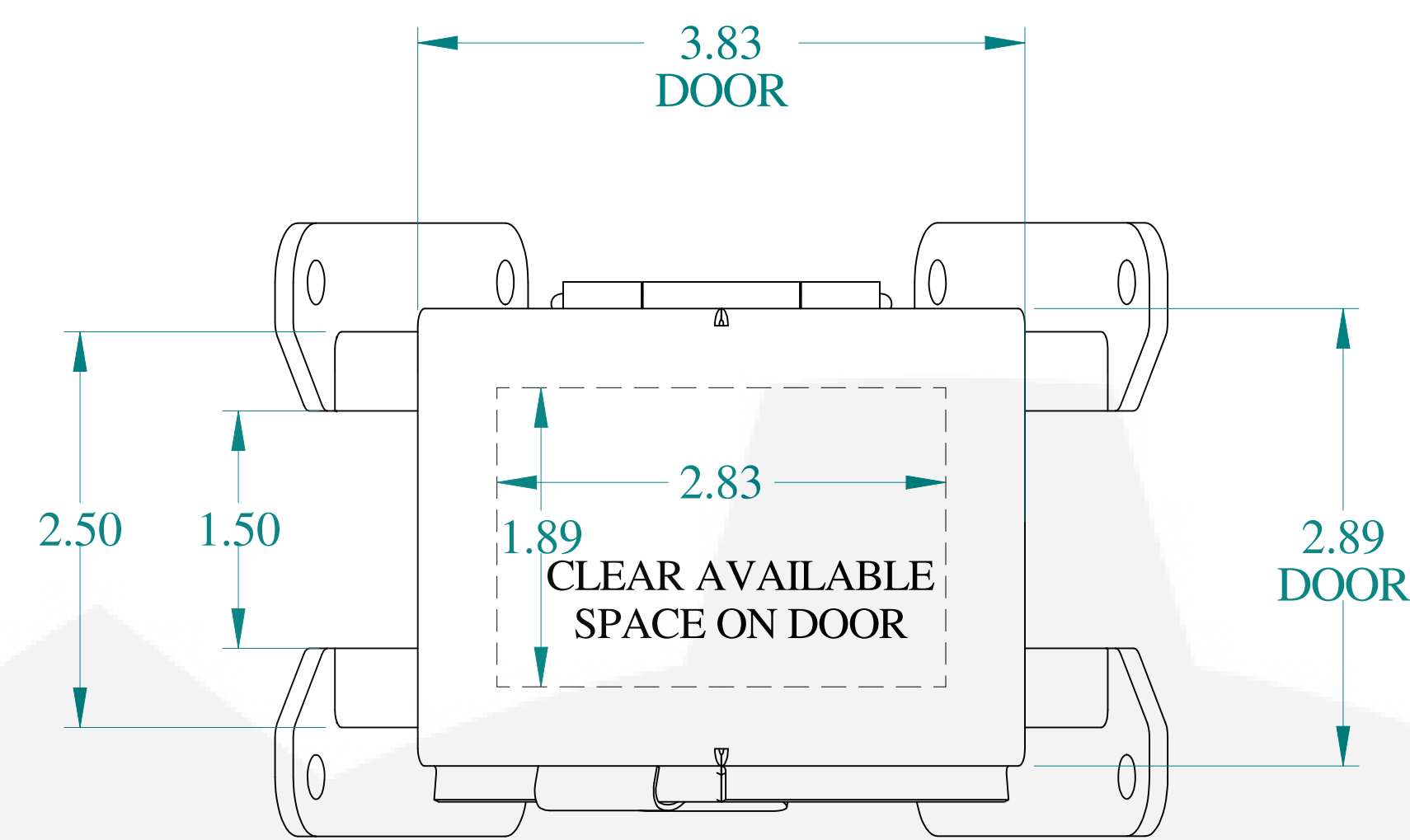
TOP VIEW
