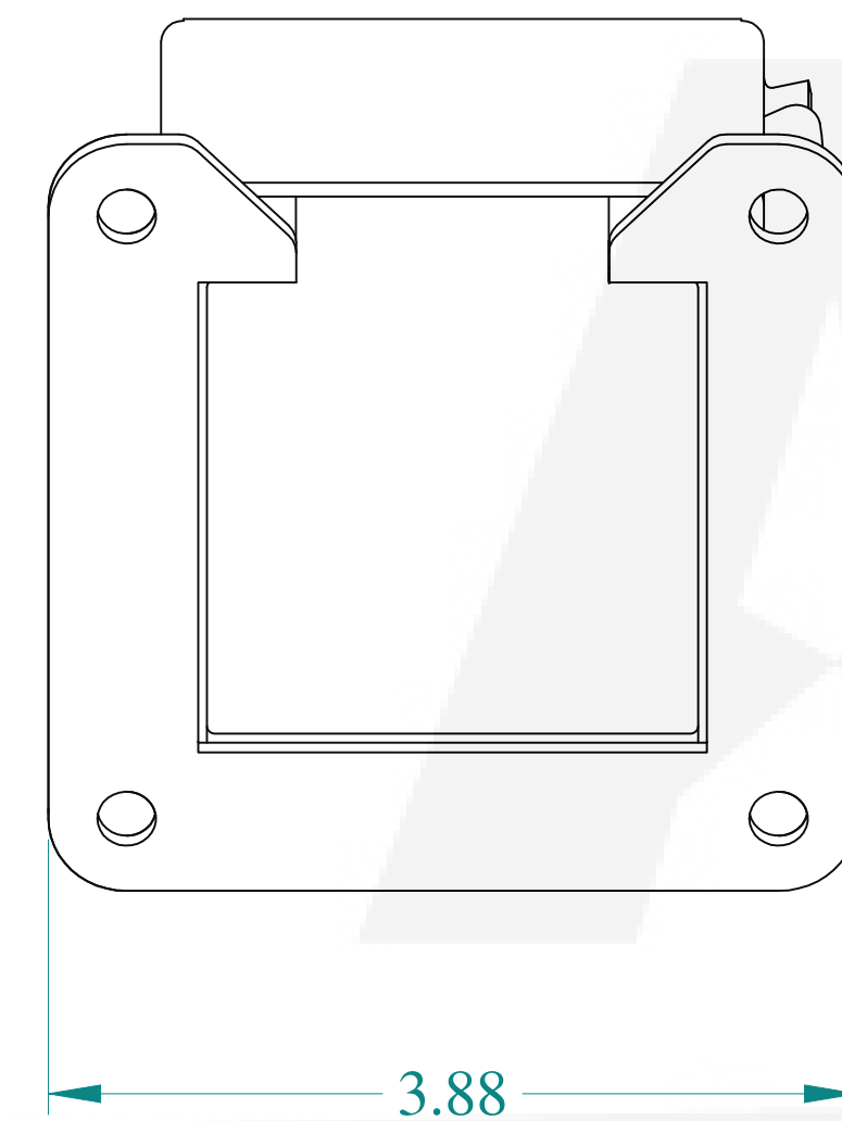
SIDE VIEW
