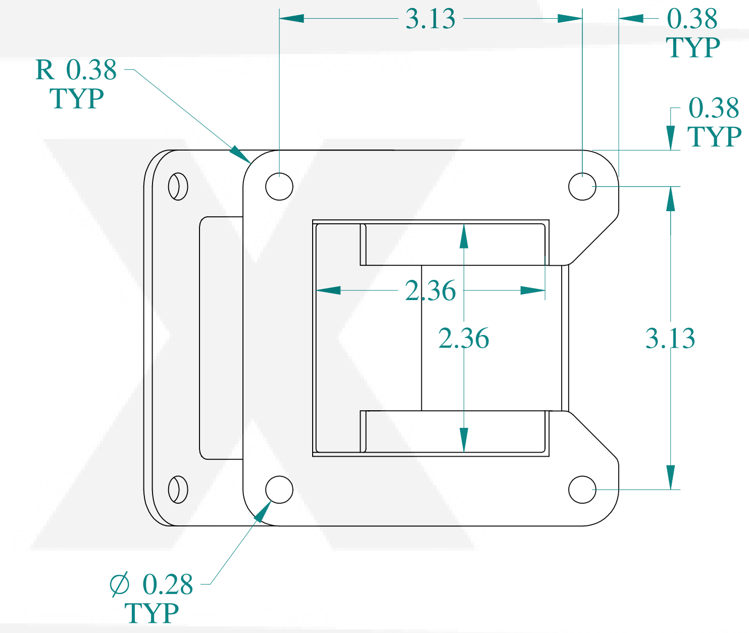
VIEW Z-Z
