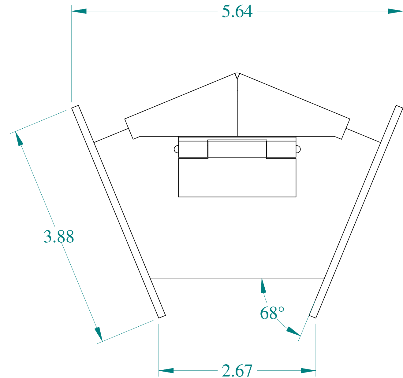
BACK VIEW
