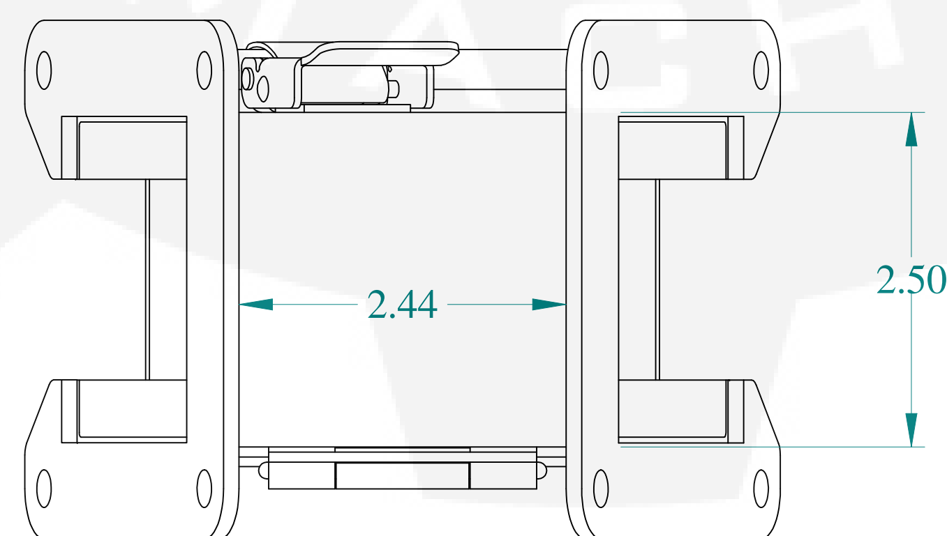
BOTTOM VIEW
