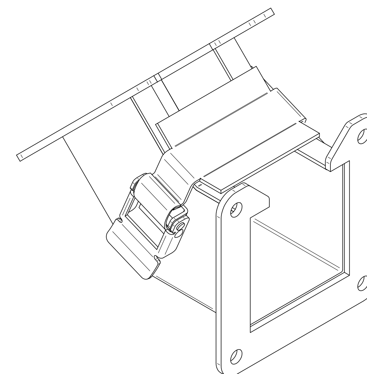
ISOMETRIC VIEWS
