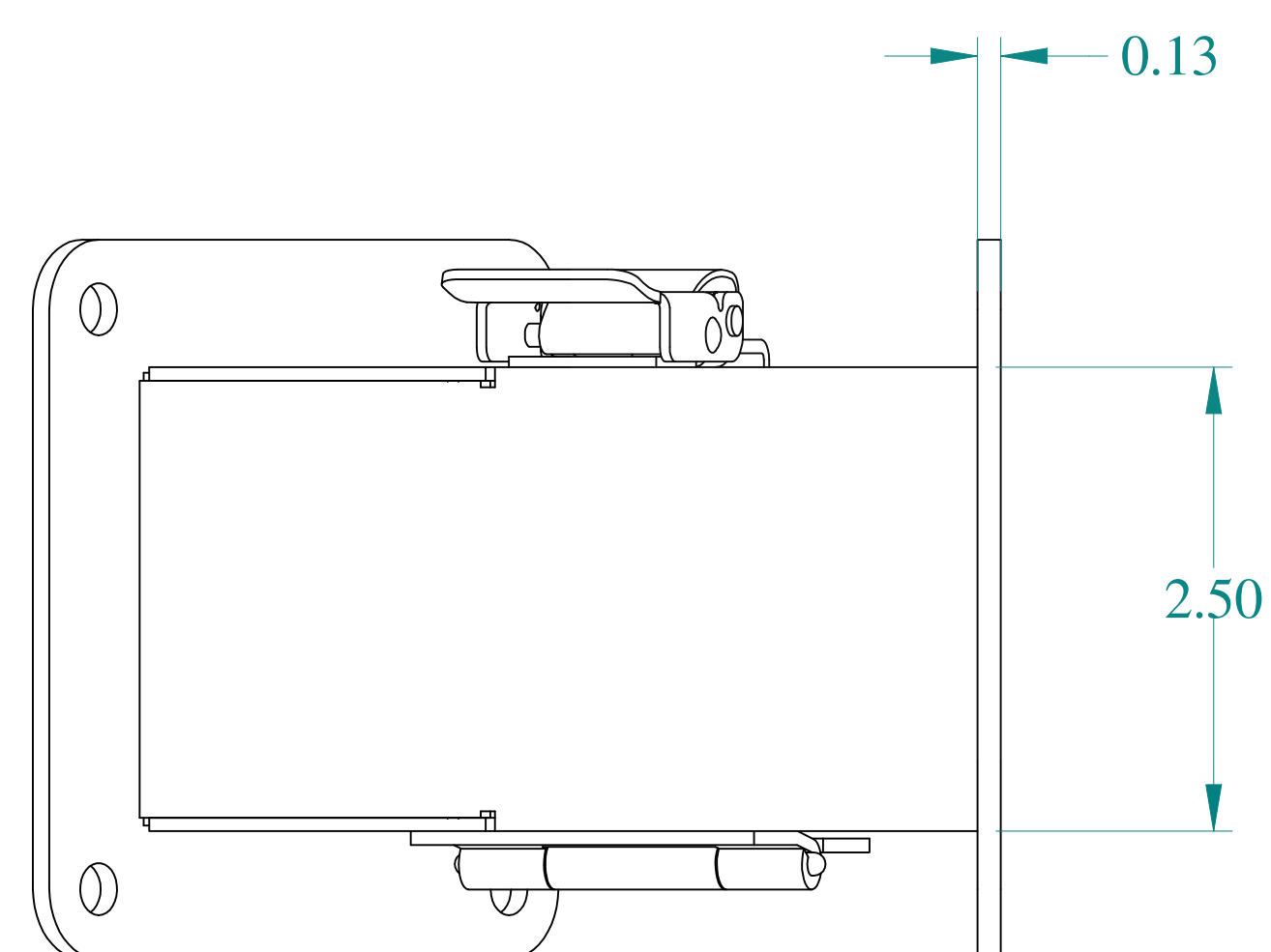
BOTTOM VIEW
