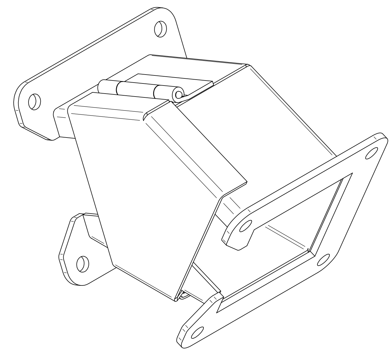
ISOMETRIC VIEWS
