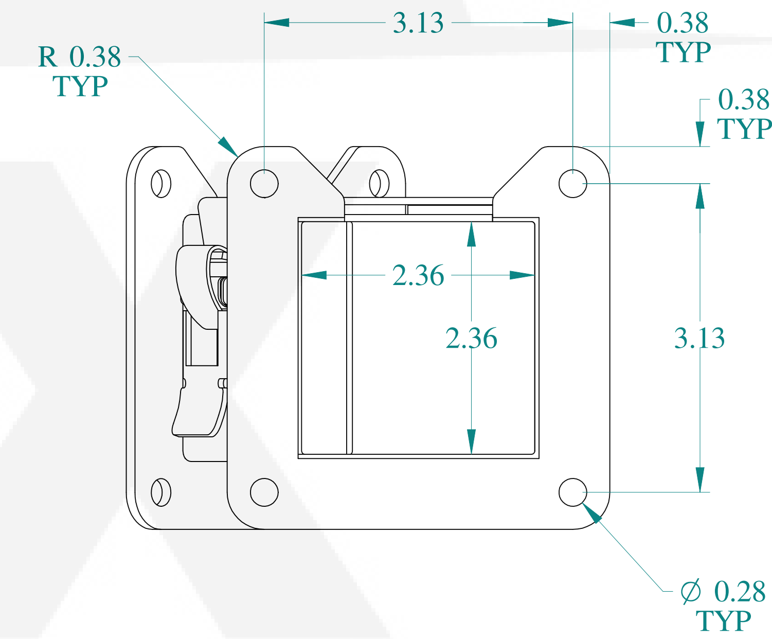
VIEW Z-Z
