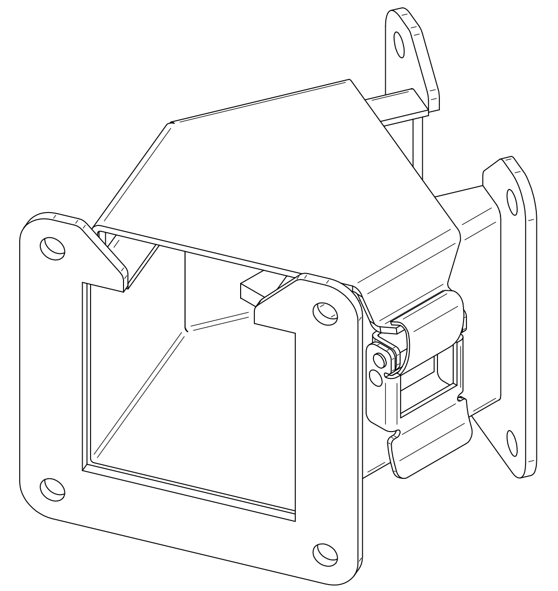
ISOMETRIC VIEWS
