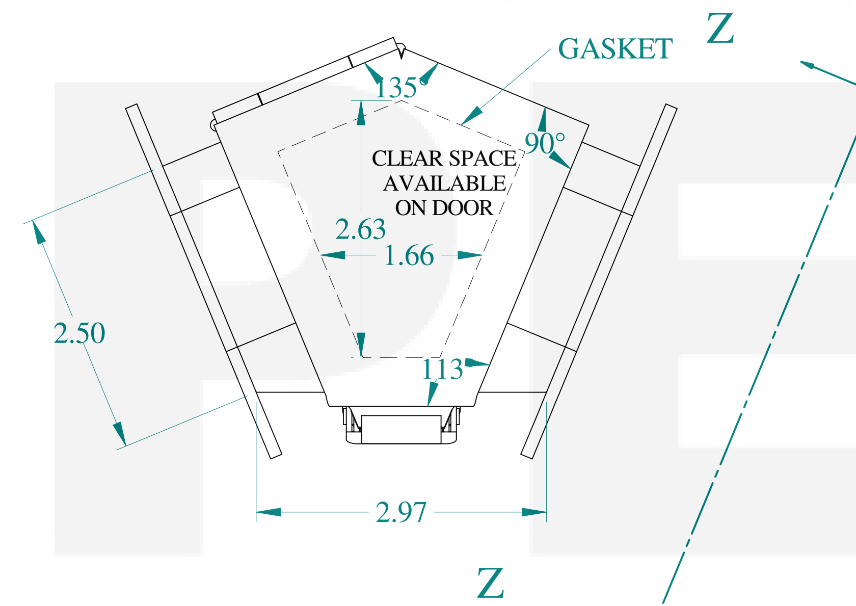
FRONT VIEW
