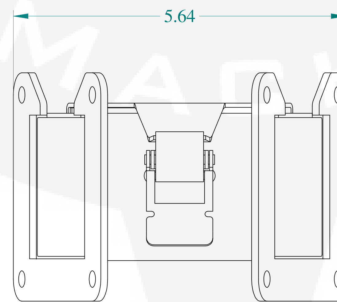
BOTTOM VIEW
