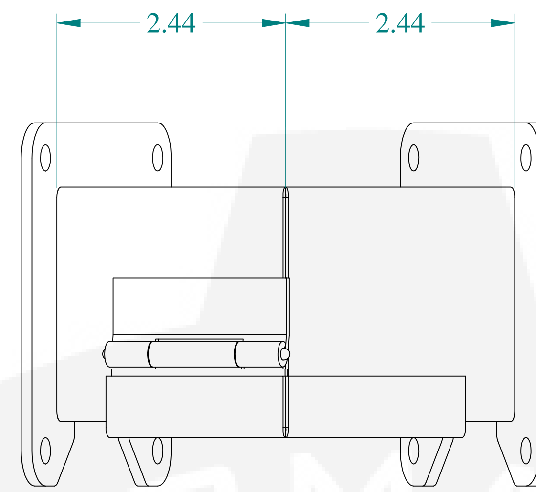
TOP VIEW
