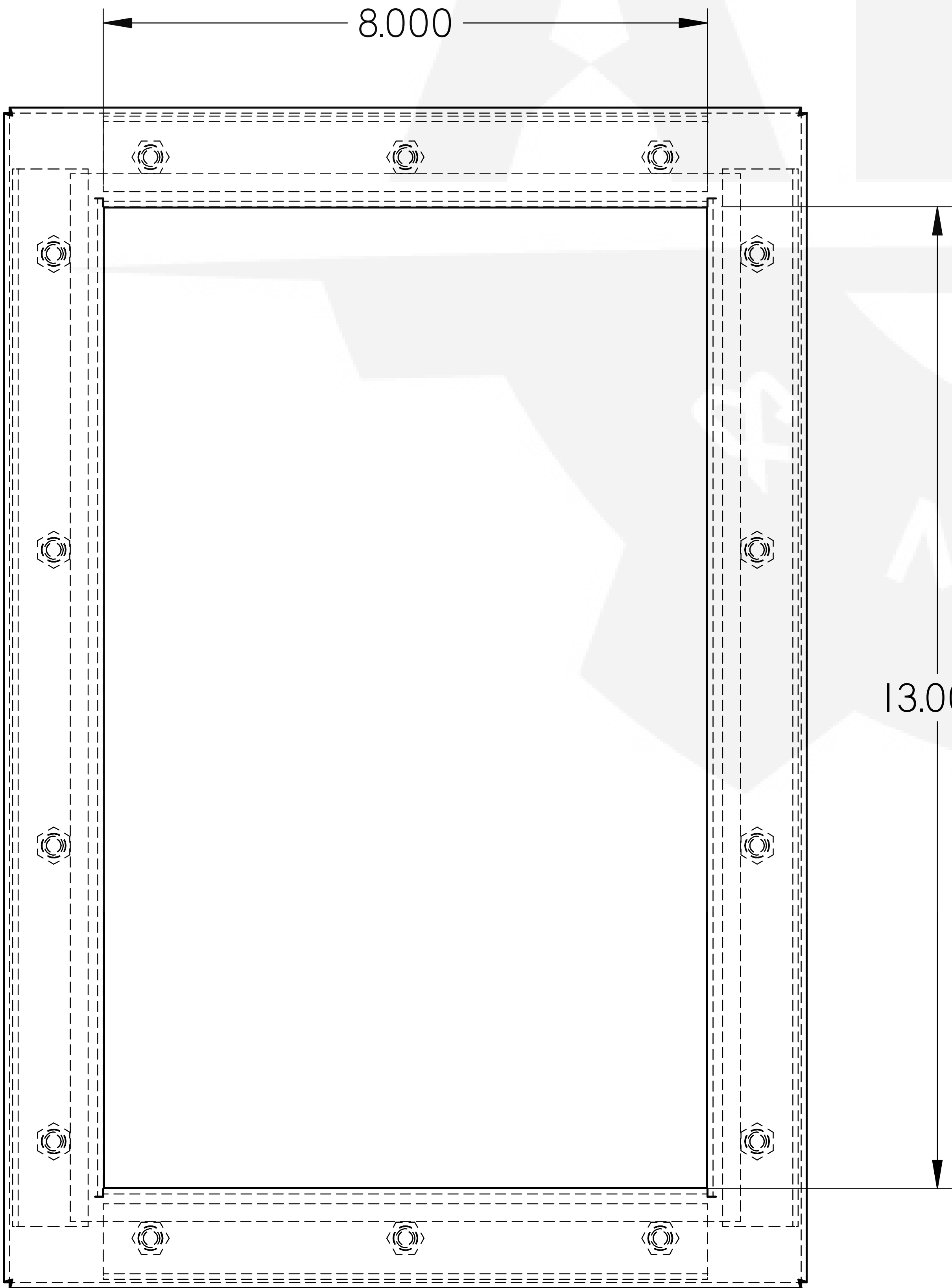
FRONT VIEW
