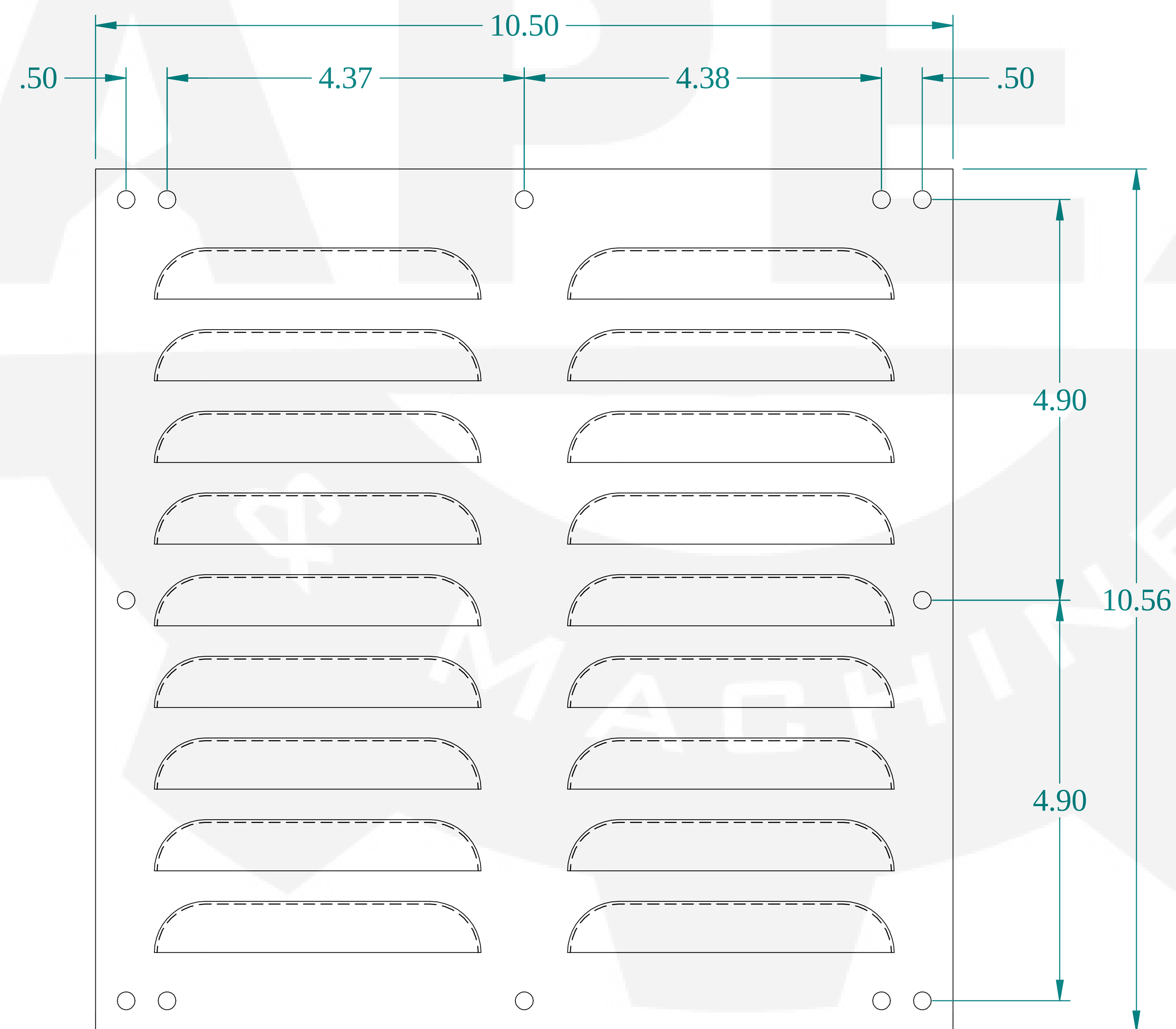
FRONT VIEW
