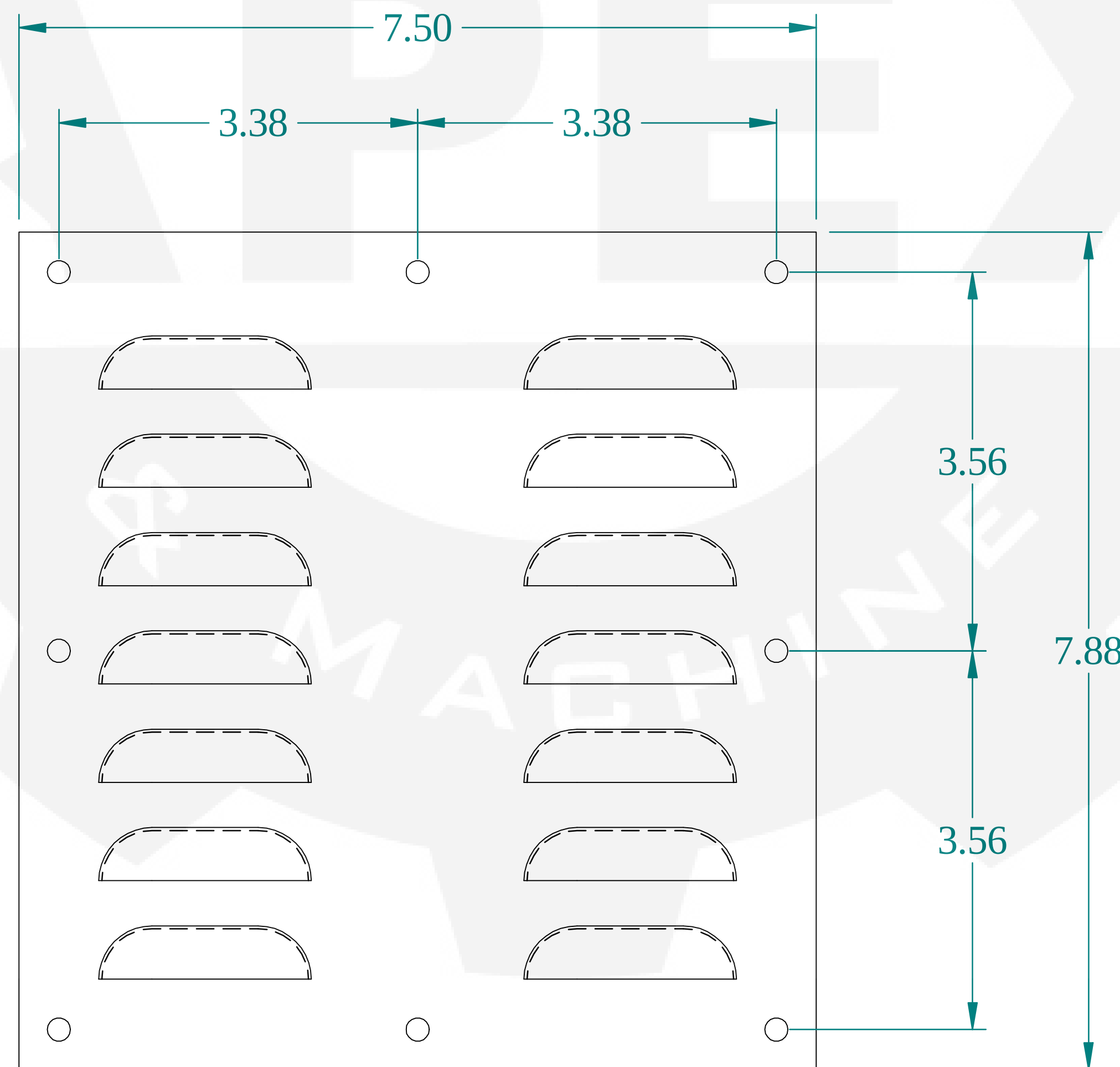
FRONT VIEW
