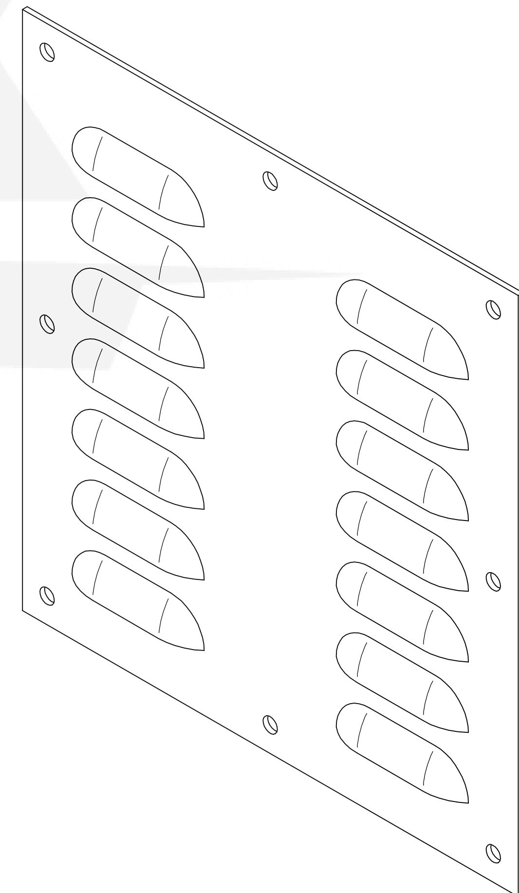
ISOMETRIC VIEW
