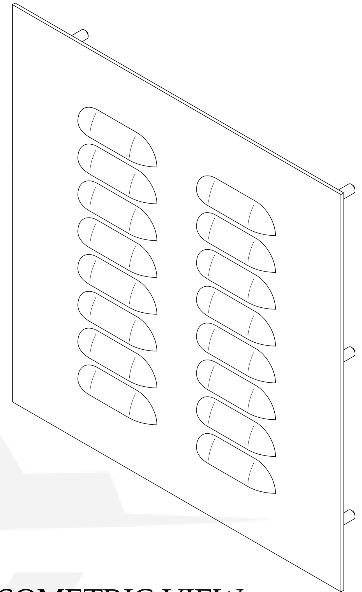
ISOMETRIC VIEW
