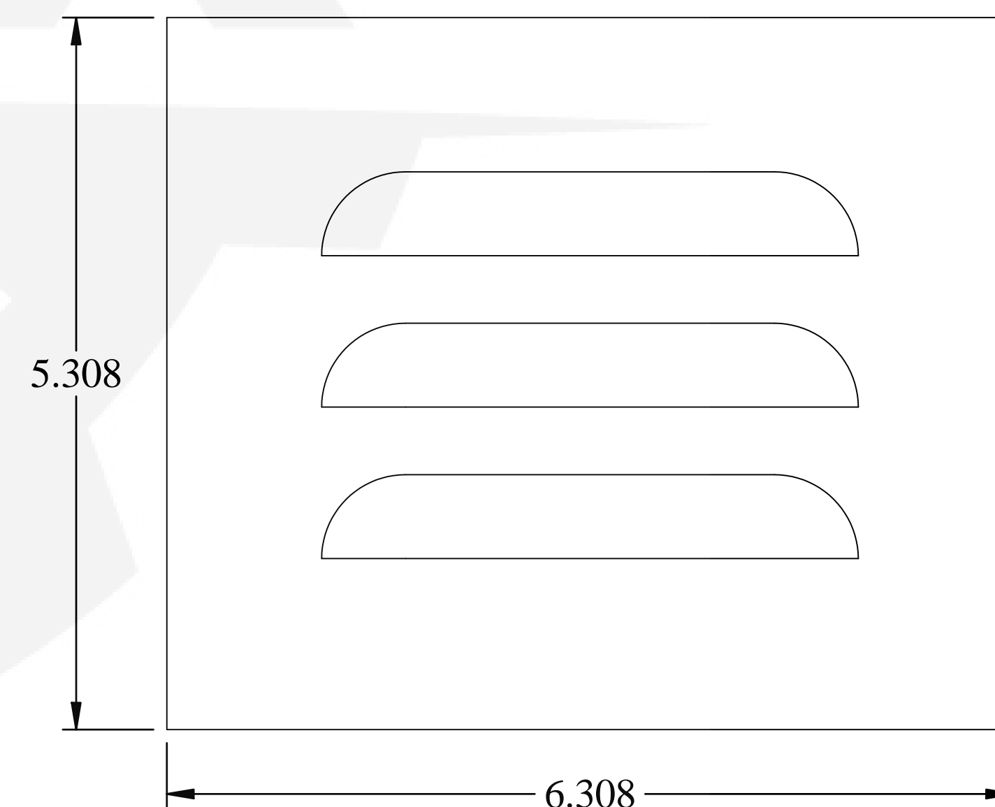
FRONT VIEW
