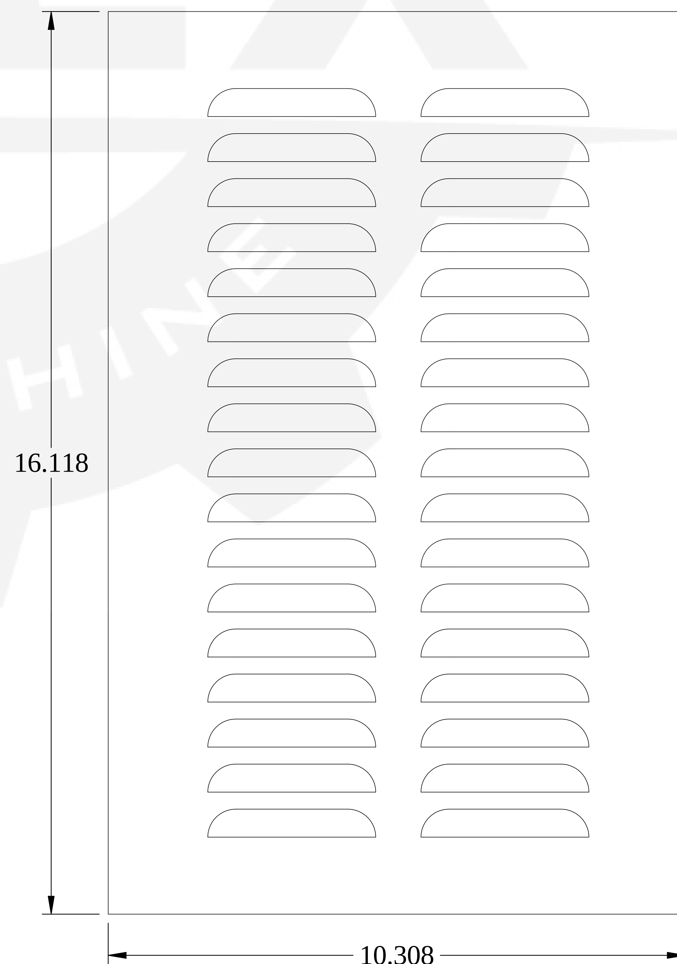
FRONT VIEW
