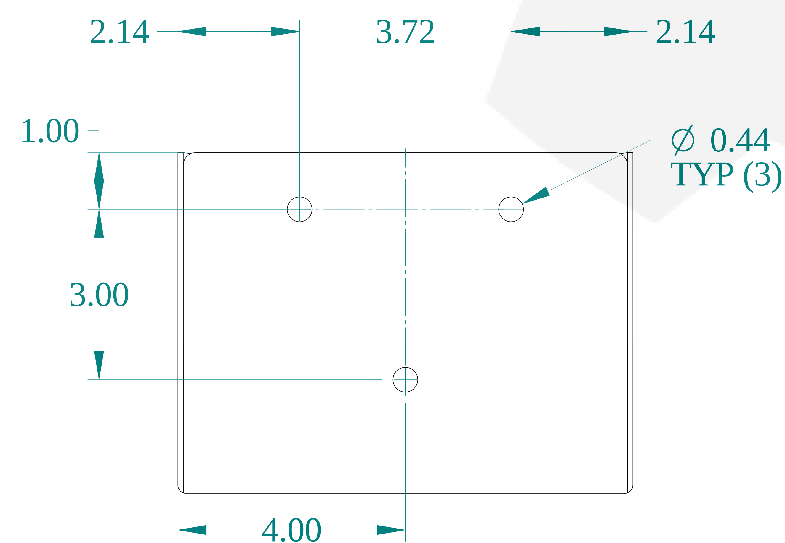
BOTTOM VIEW
