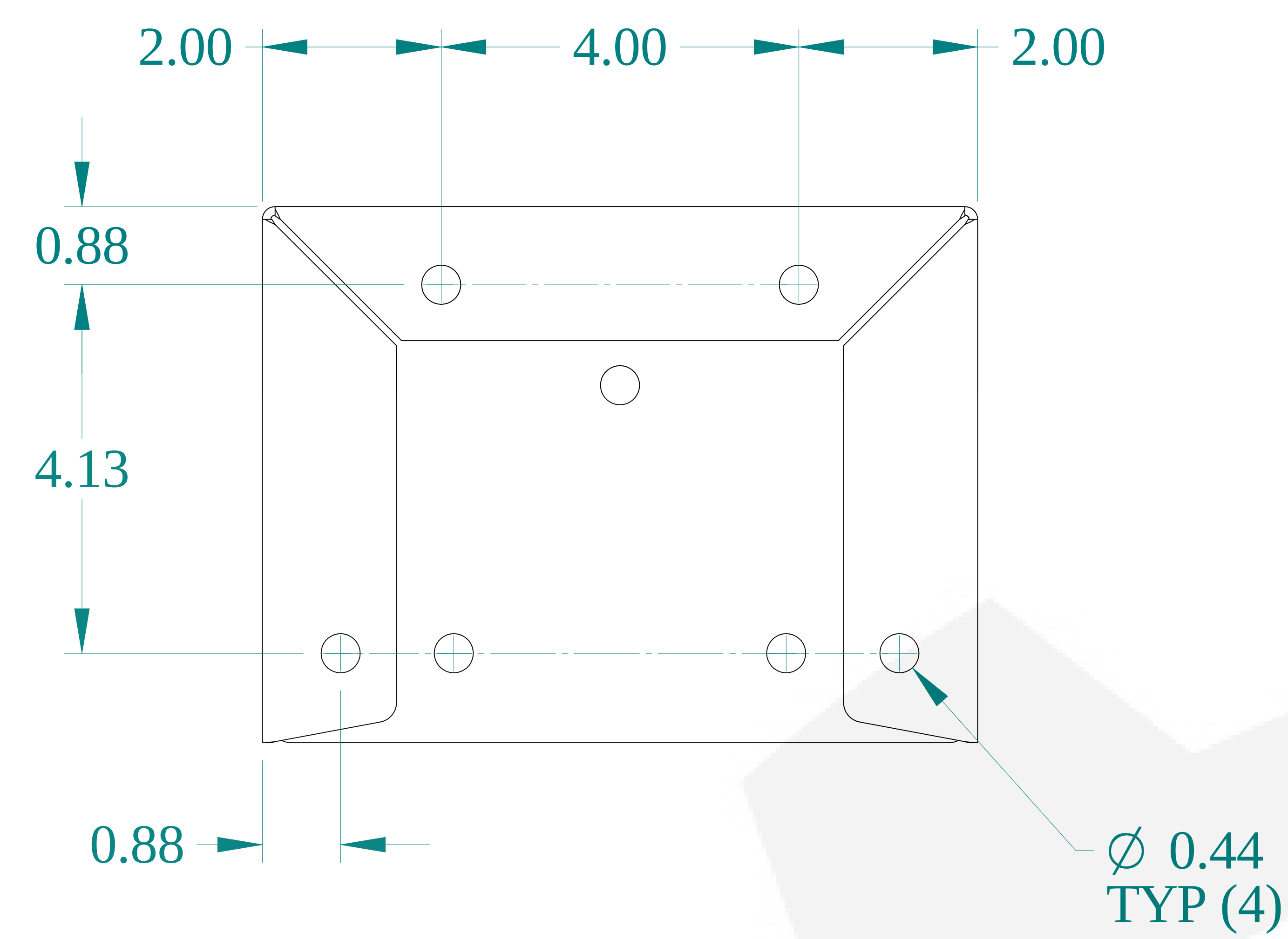
TOP VIEW
