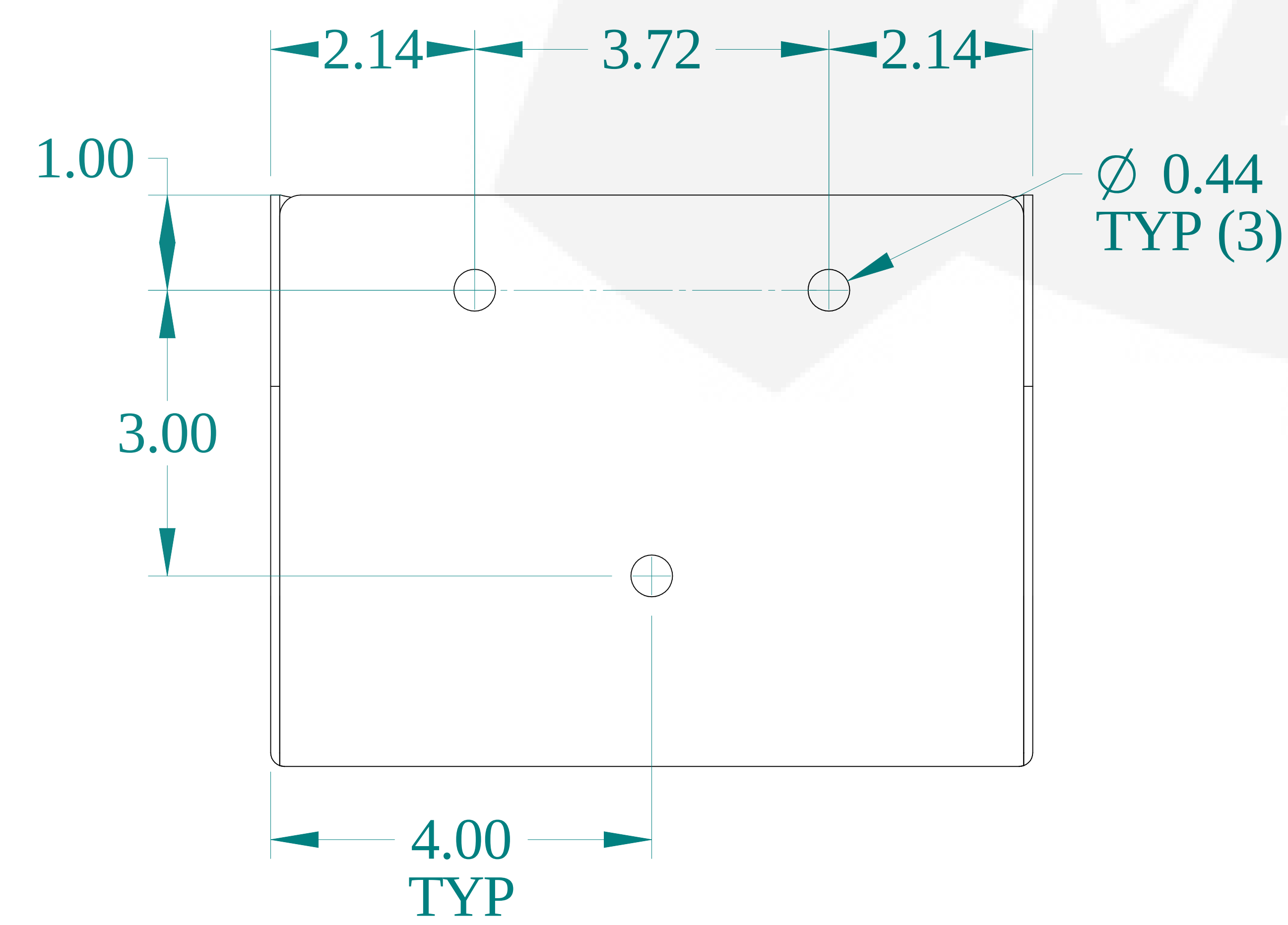
BOTTOM VIEW
