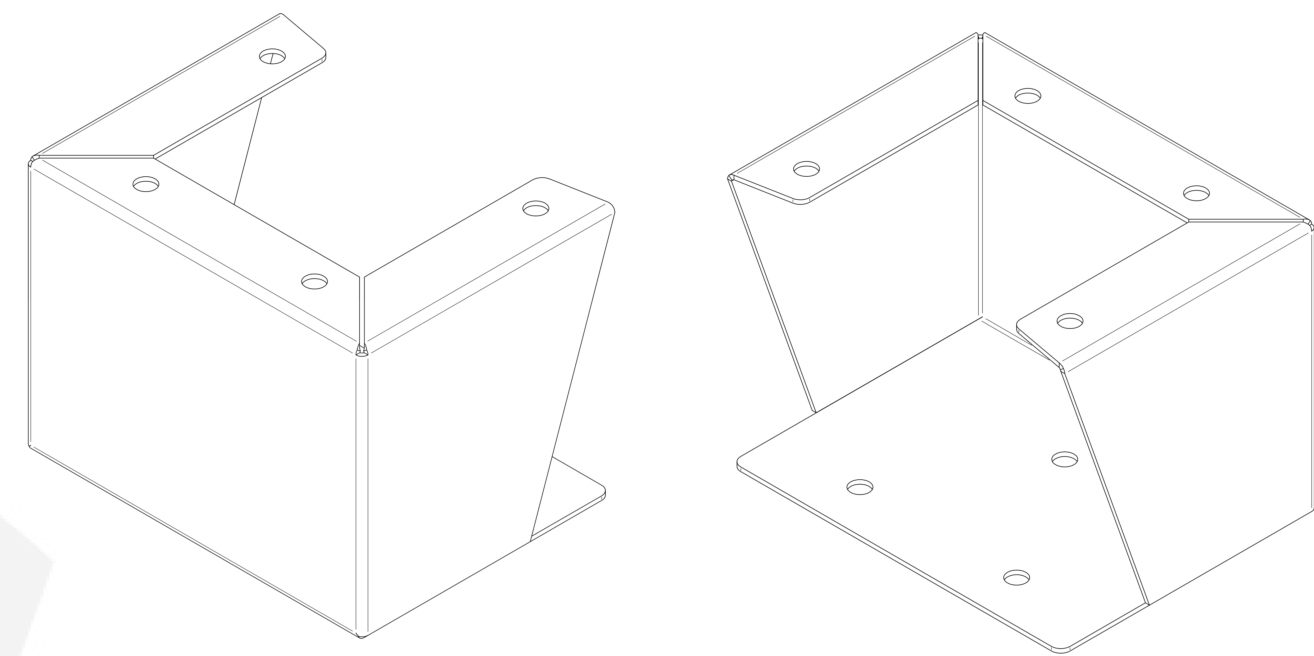
ISOMETRIC VIEWS
