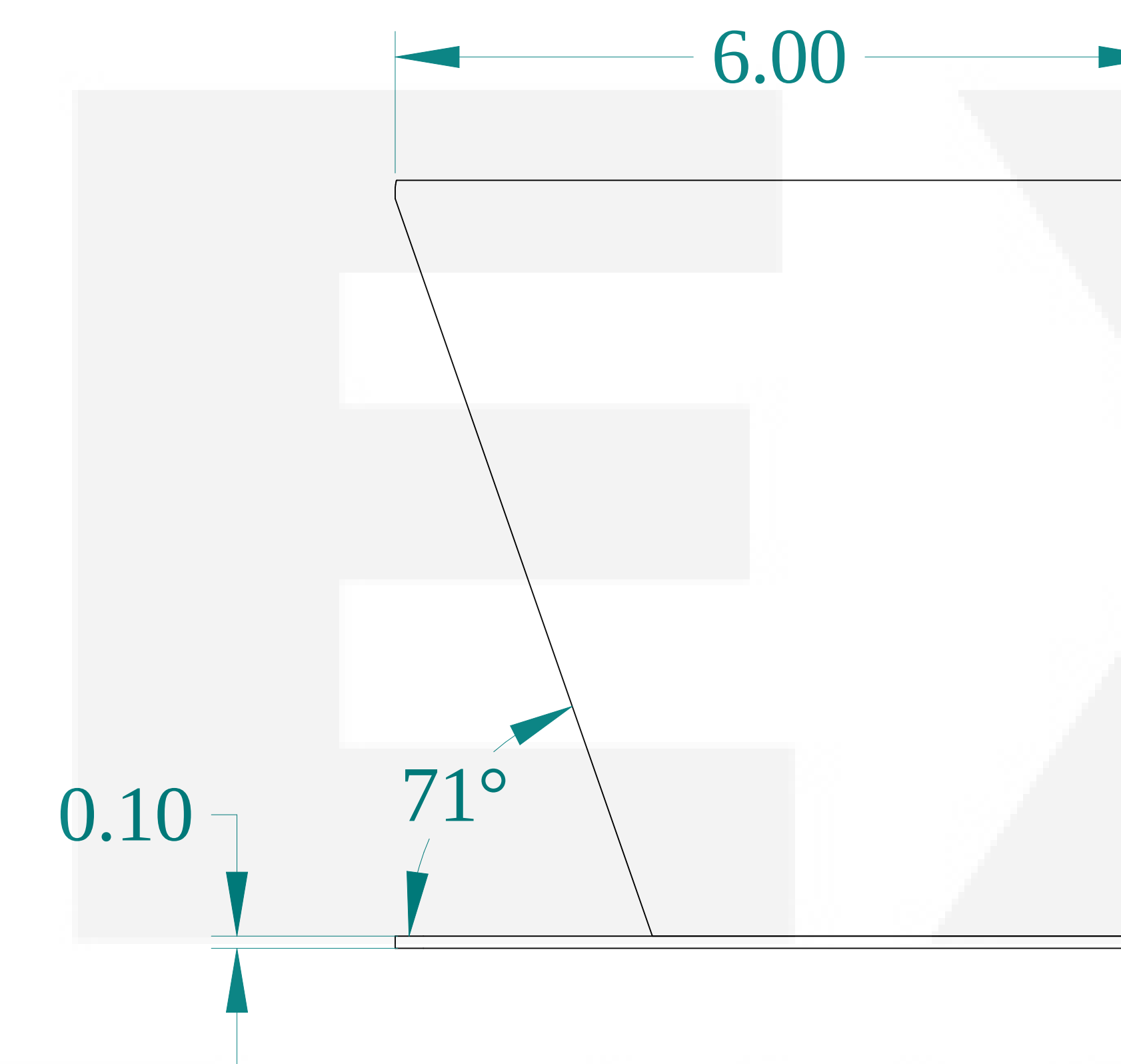
SIDE VIEW
